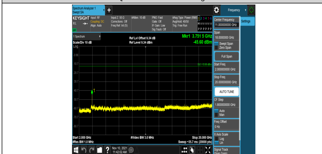
Band2-10MHz-16QAM-18900-1RB#0-Range5:2000~20000MHz
