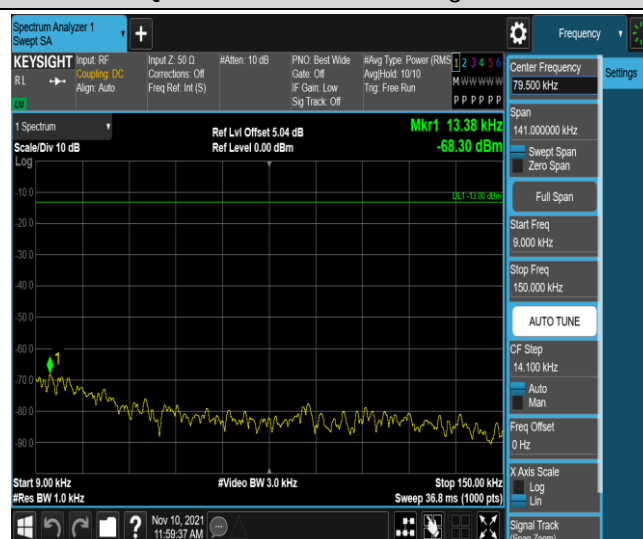
Band2-15MHz-16QAM-18675-1RB#0-Range1:0.009~0.15MHz
