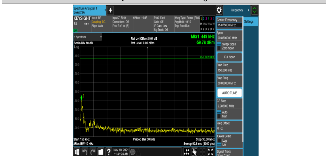
Band2-10MHz-16QAM-18900-1RB#0-Range2:0.15~30MHz
