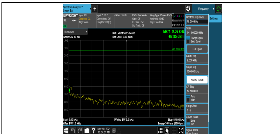
Band2-1.4MHz-16QAM-19193-1RB#0-Range1:0.009~0.15MHz
