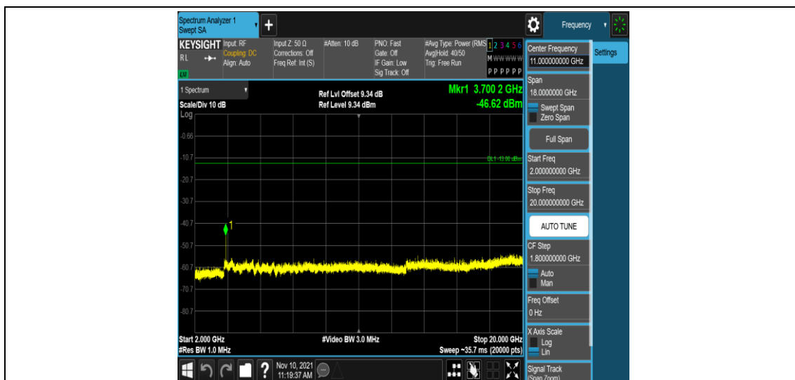
Band2-5MHz-16QAM-18625-1RB#0-Range5:2000~20000MHz
