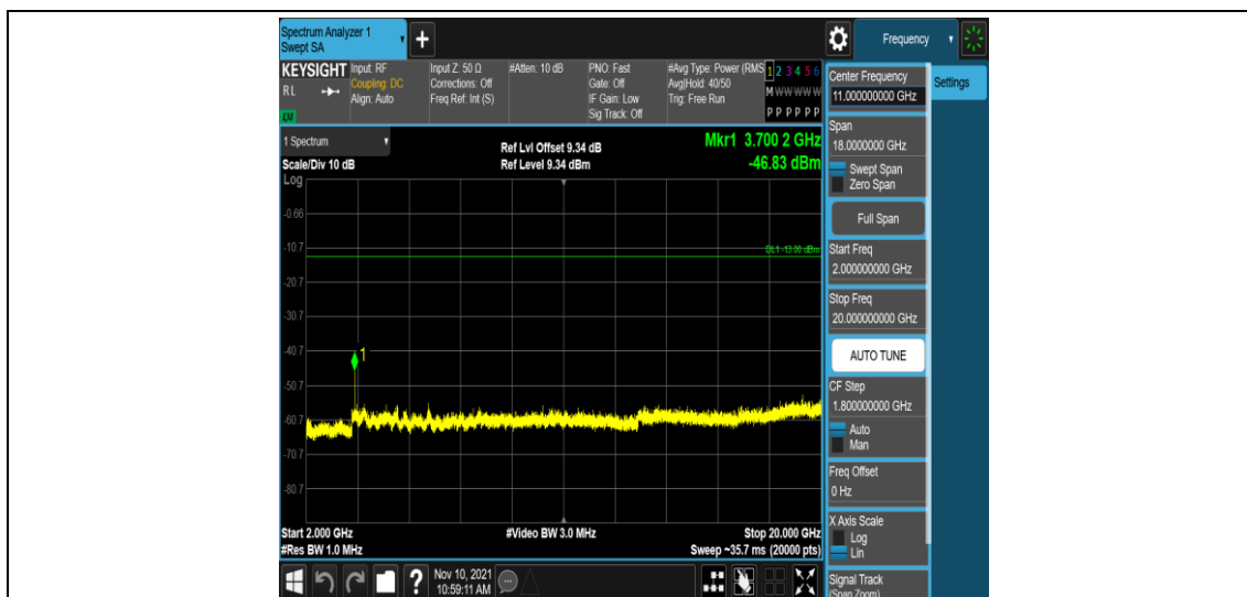
Band2-3MHz-16QAM-18615-1RB#0-Range5:2000~20000MHz
