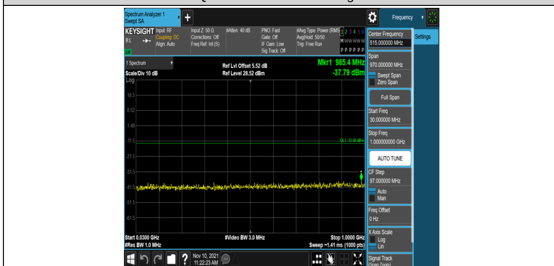
Band2-5MHz-QPSK-19175-1RB#0-Range3:30~1000MHz
