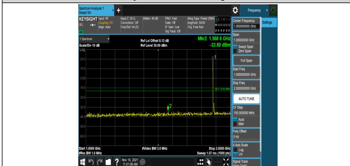
Band2-3MHz-16QAM-18900-1RB#0-Range4:1000~2000MHz
