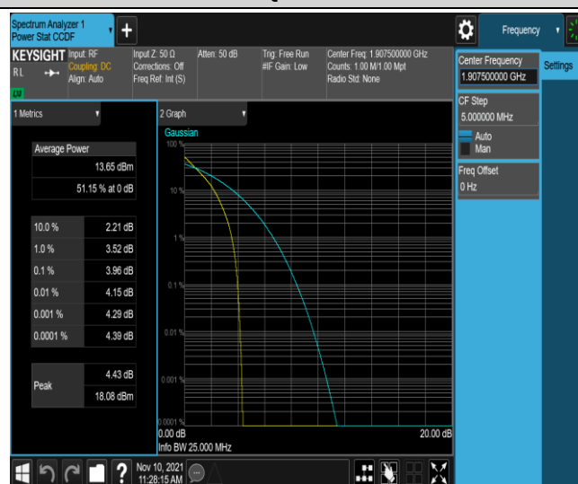
Band2-5MHz-QPSK-19175-25RB#0
