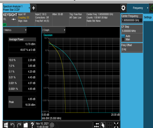
Band2-10MHz-QPSK-19150-50RB#0
