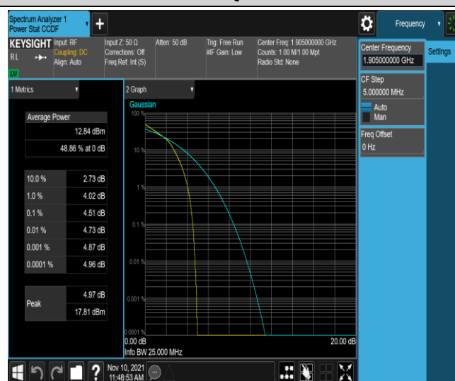
Band2-10MHz-16QAM-19150-50RB#0
