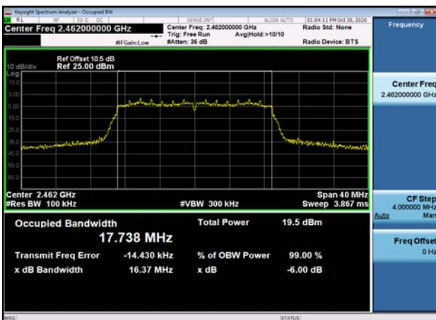
6dB Bandwidth-802.11n(HT20),2462MHz
