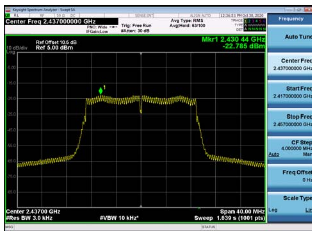
Power spectral density-802.11n(HT20) ,2437MHz
