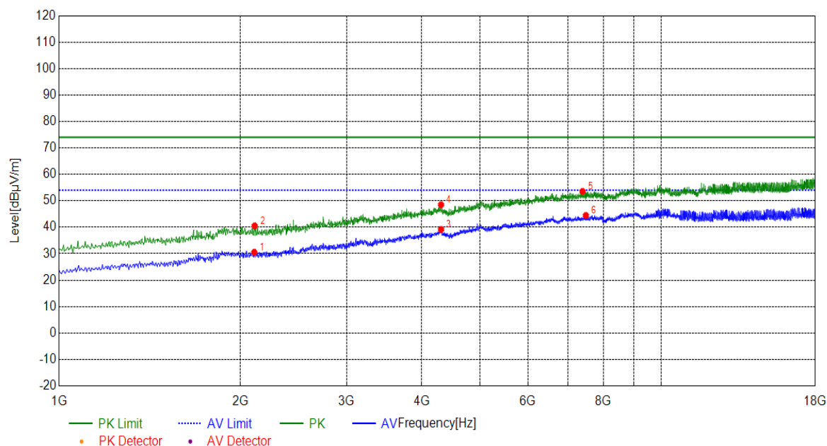
(Plot E: Test Antenna Horizontal 1G – 18G)
