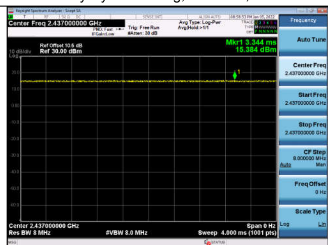
Output Power-802.11n (HT40),2437MHz,Ant0
