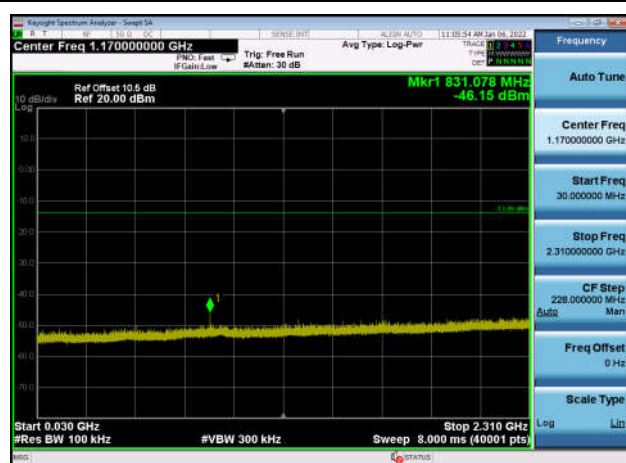
,Plot 3,30MHz~2310MHz-802.11g,2462MHz
