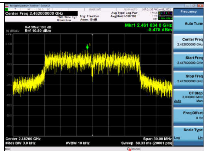
Power spectral density-802.11g ,2462MHz,Ant0
