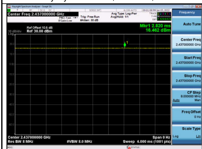
Output Power-802.11n (HT20),2437MHz,Ant0
