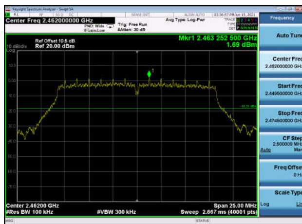
,Plot 1,Reference Level-802.11g ,2462MHz
