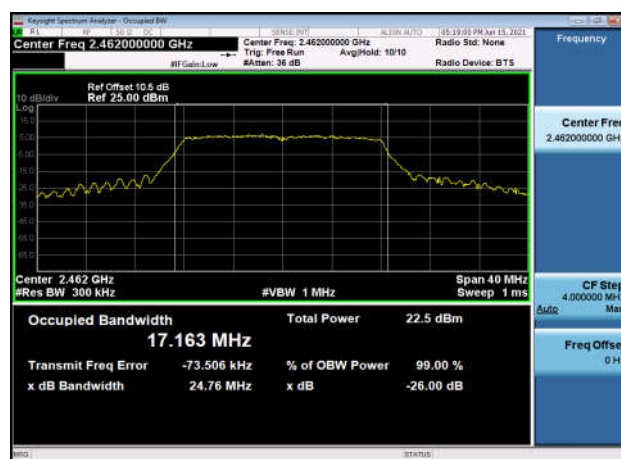
99% Bandwidth-802.11g,2462MHz
