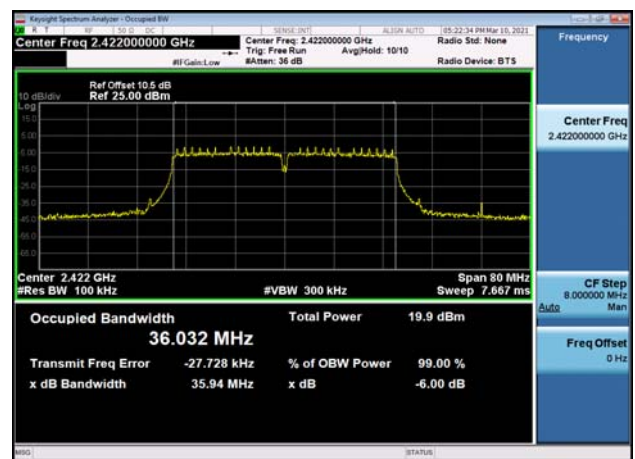
6dB Bandwidth-802.11n(HT40),2422MHz
