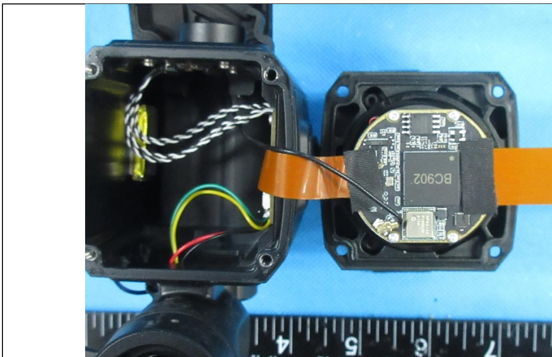
Details of: Internal view 5 of main unit(SUPER YOTER LRF 50mm)
