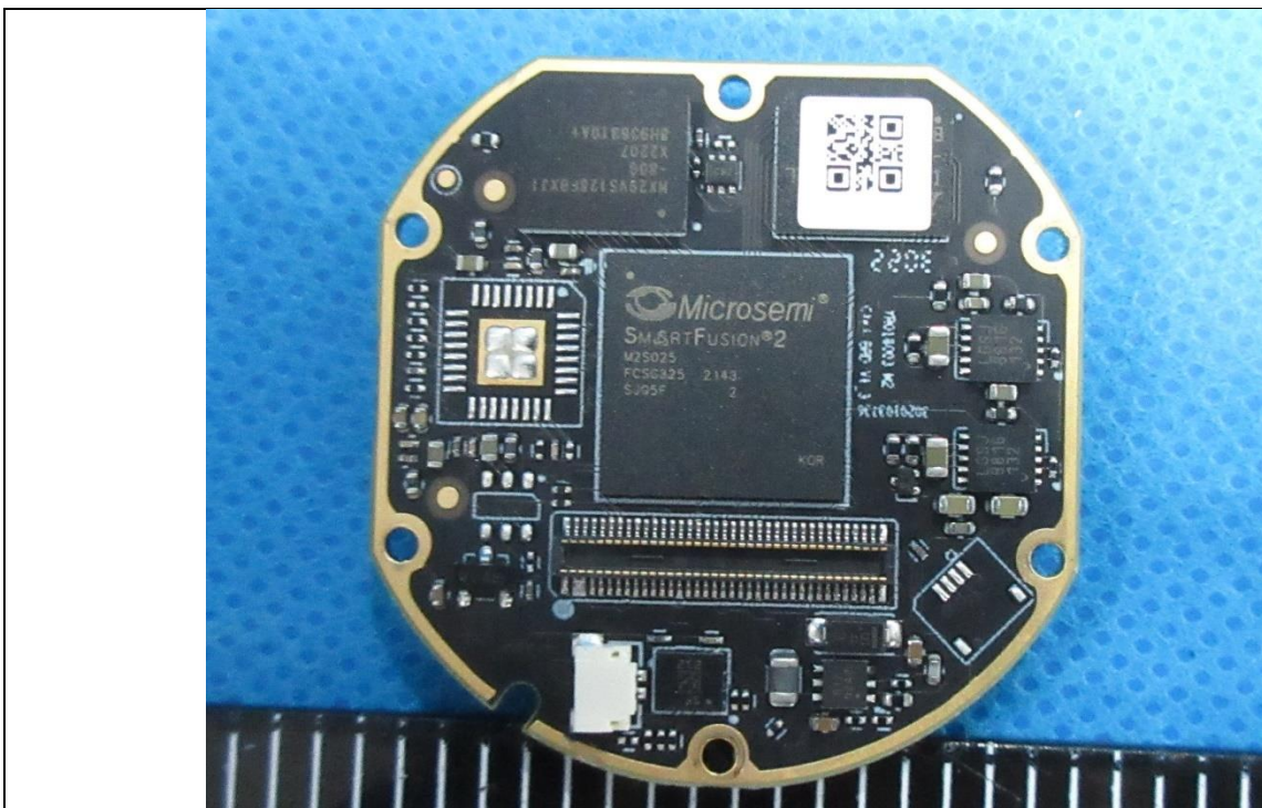
Details of: Internal view 12 of main unit(SUPER YOTER LRF 35mm)
