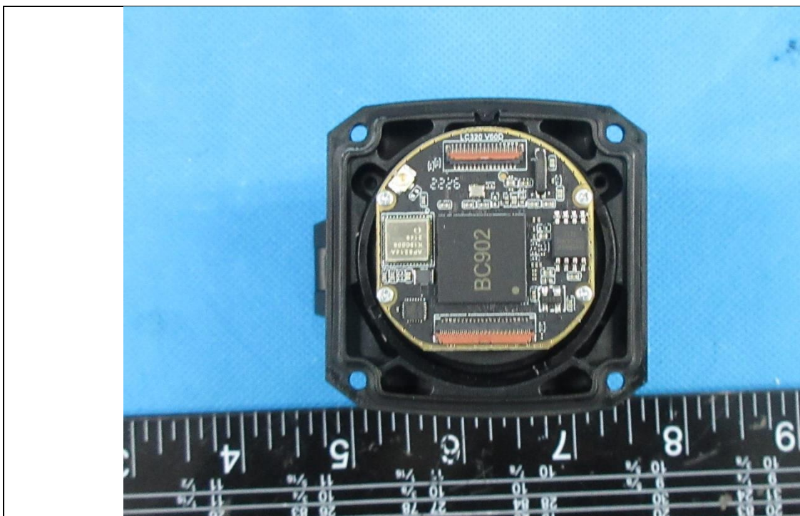
Details of: Internal view 6 of main unit(SUPER YOTER LRF 50mm)
