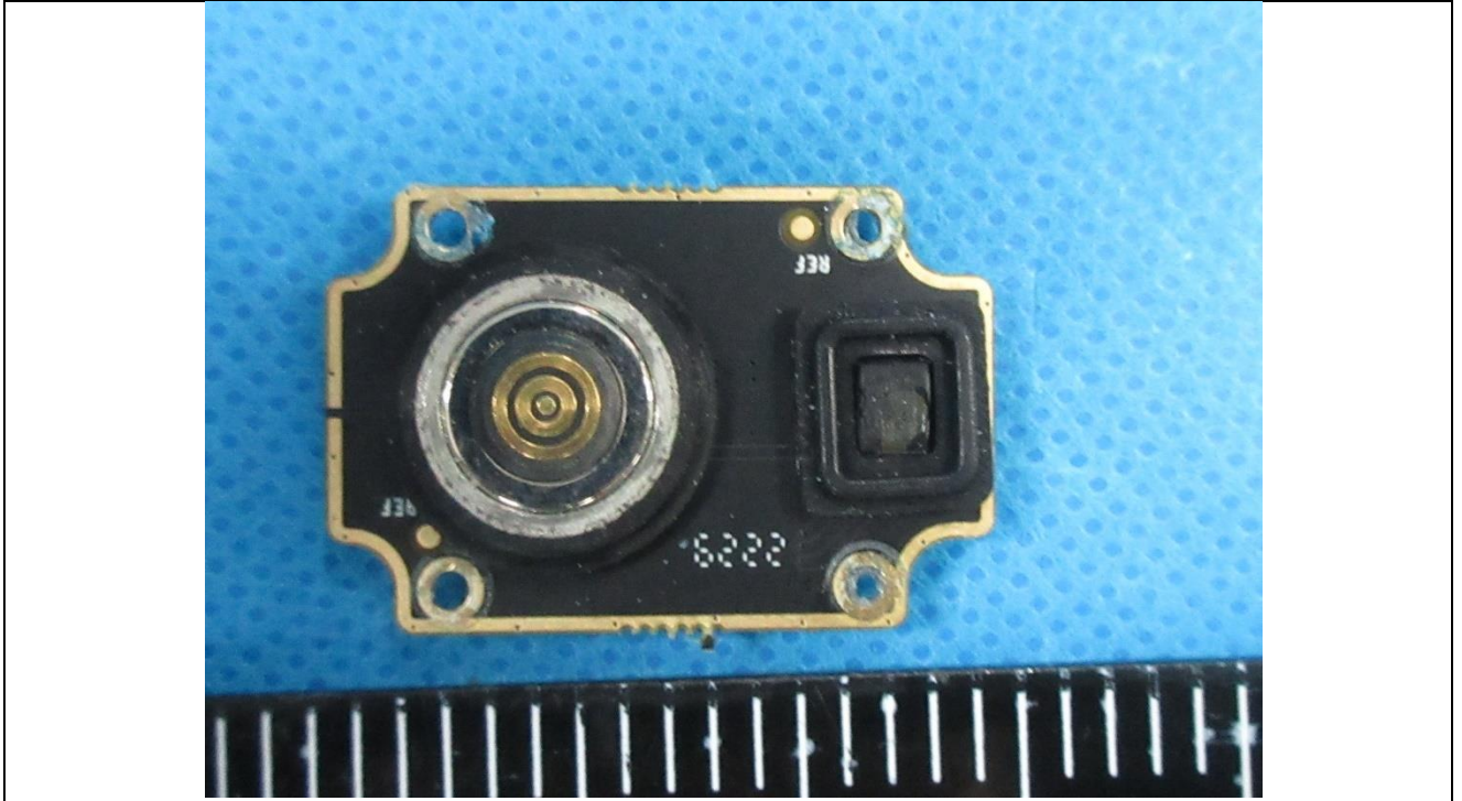
Details of: Internal view 21 of main unit(SUPER YOTER LRF 35mm)
