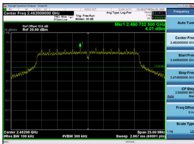
,Plot 1,Reference Level-802.11g ,2462MHz,Ant0
