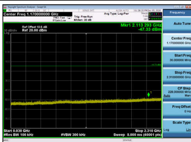
,Plot 3,30MHz~2310MHz-802.11g,2462MHz
