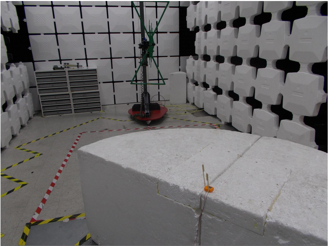
Module – radiated emissions 30MHz to 1GHz, showing use of bilog antenna
