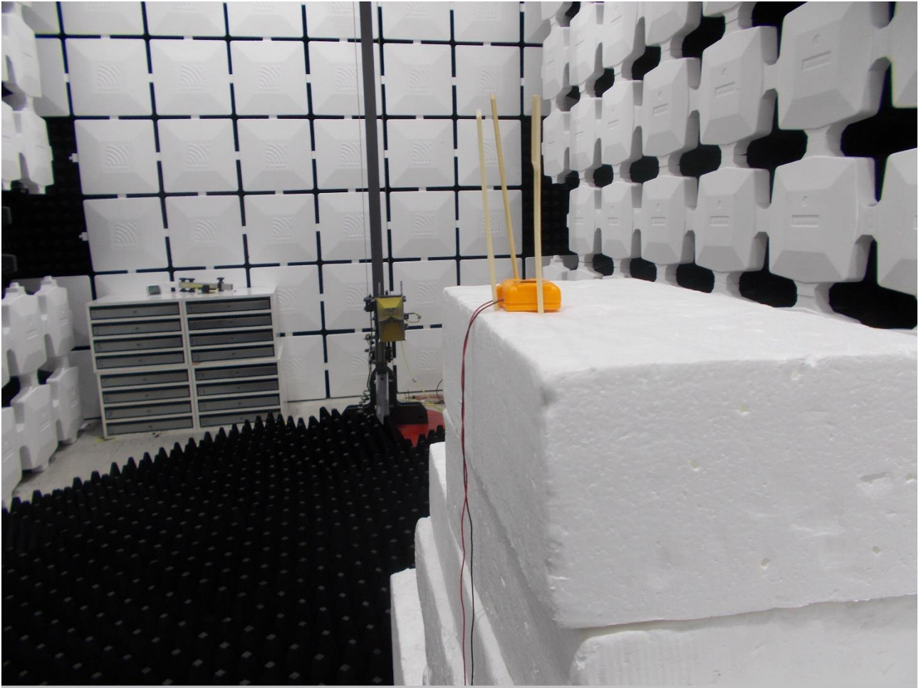
Module – Radiated emissions 1-18GHz
