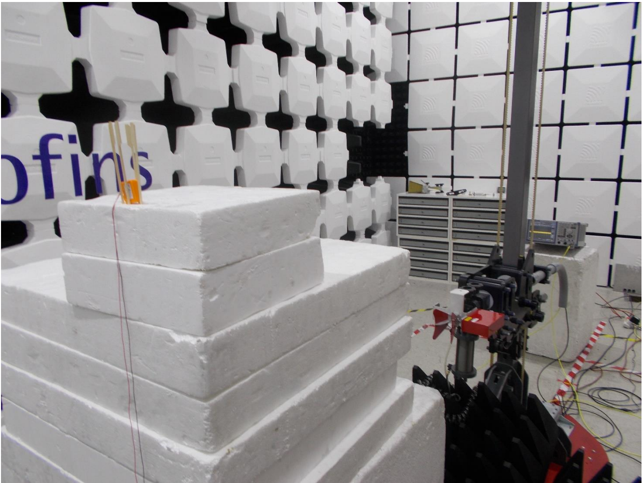
Radiated emissions investigation 18-26GHz
