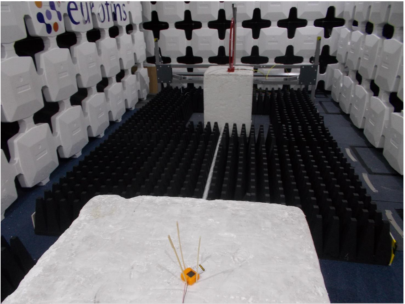
Module – Magnetic field test 9kHz to 30MHz – antenna perpendicular
