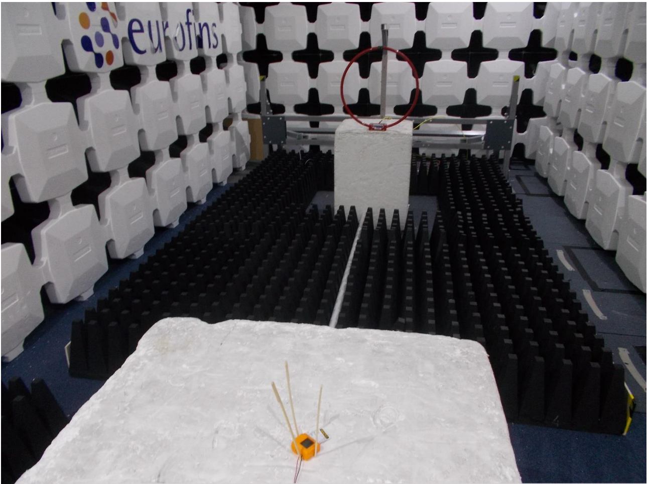
Module – Magnetic field test 9kHz to 30MHz – antenna parallel
