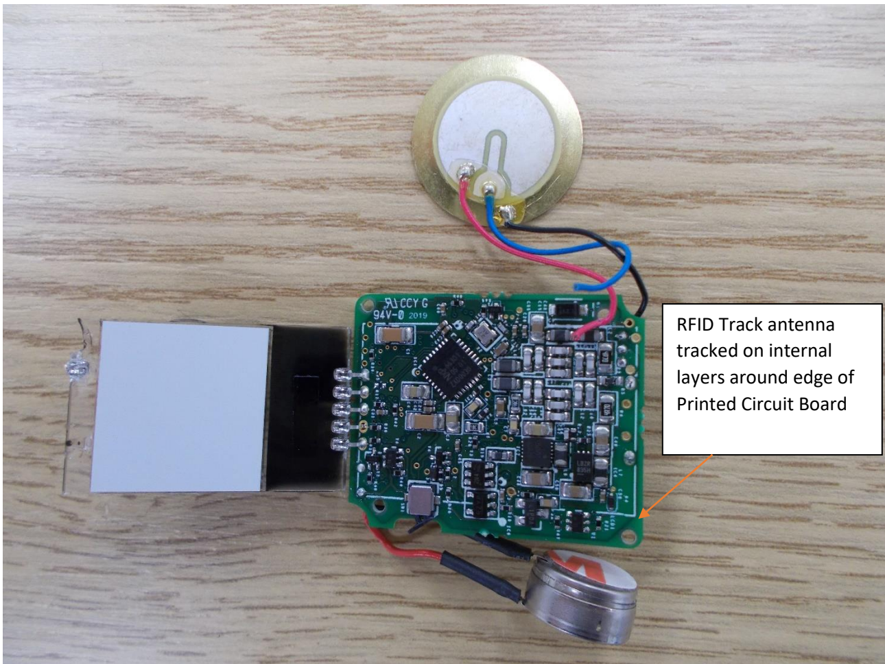
Component side – screen removed
