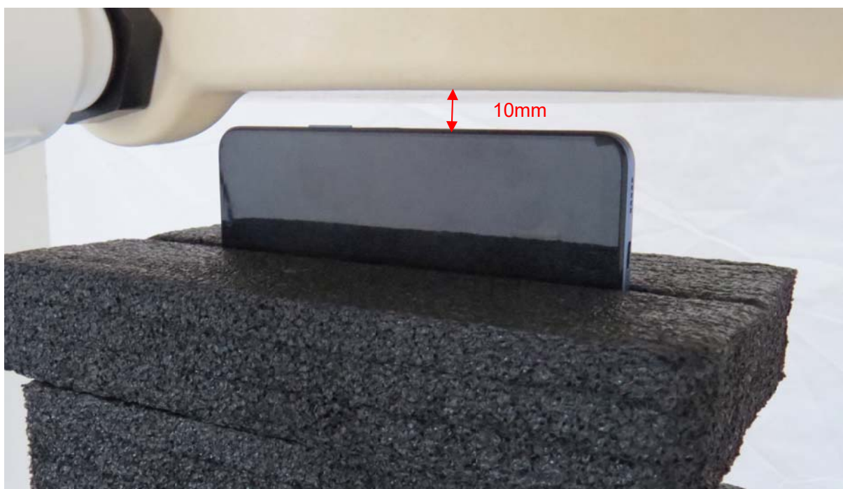
Picture 10: Right Edge, the distance from handset to the bottom of the Phantom is 10mm
