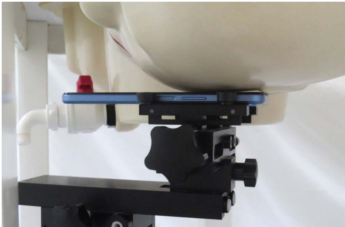
Picture 1: Left Hand Touch Cheek Position
