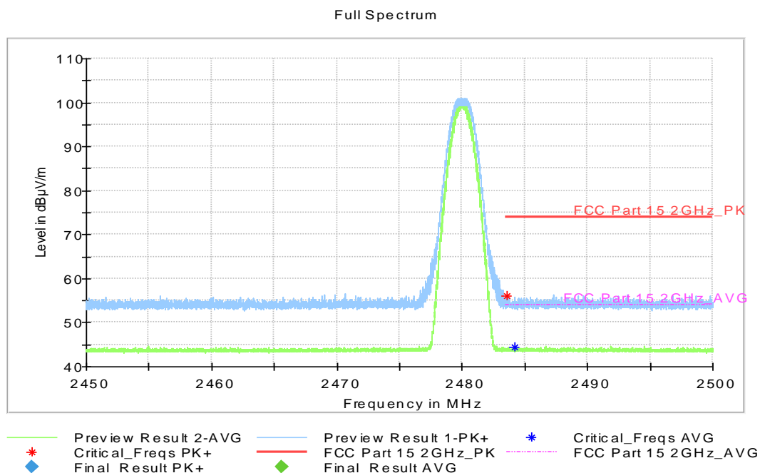
Fig.8. Frequency Band Edges: GFSK, 2480 MHz, Hopping Off, 2.45 GHz - 2.50GHz
