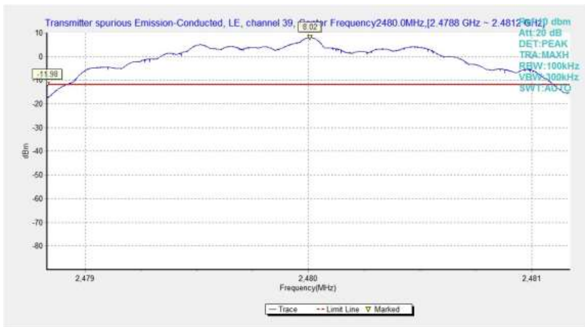
Fig.23. Transmitter Spurious Emission - Conducted: GFSK, 2480 MHz
