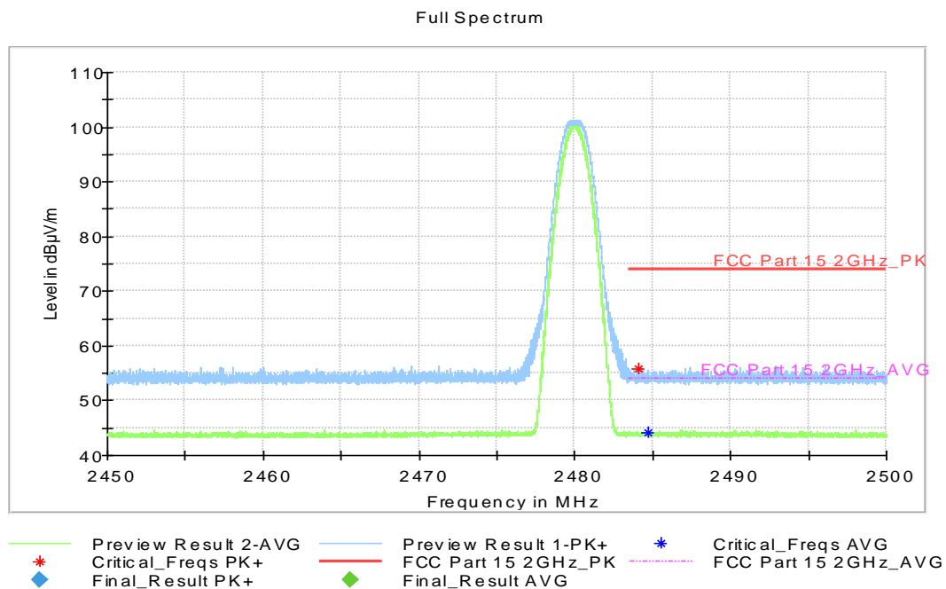
Fig.12. Frequency Band Edges: GFSK, 2480 MHz, Hopping Off, 2.45 GHz - 2.50GHz
