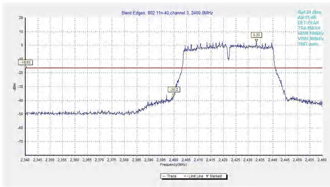
Fig.A.5.7 Band Edges (802.11n-HT40, Ch 3)
