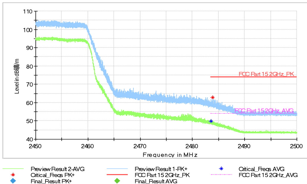
Fig.A.5.23 Band Edges (802.11n-HT40, Ch 7, 2.45 GHz – 2.5GHz)
