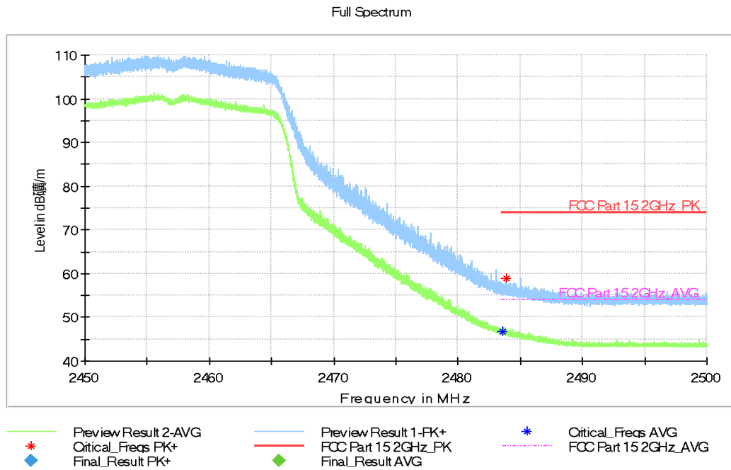
Fig.A.5.17 Band Edges (802.11n-HT20, Ch 10, 2.45 GHz – 2.5GHz)
