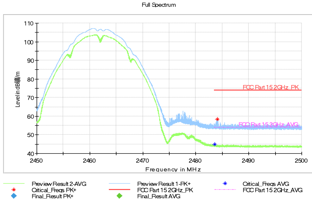
Fig.A.5.10 Band Edges (802.11b, Ch 11, 2.45 GHz – 2.5GHz)
