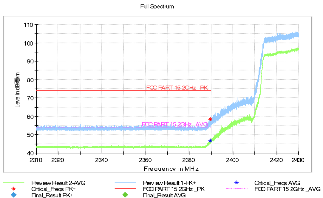
Fig.A.5.21 Band Edges (802.11n-HT40, Ch 5, 2.31 GHz – 2.43GHz)
