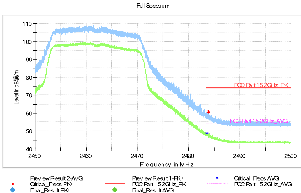
Fig.A.5.19 Band Edges (802.11n-HT20, Ch 11, 2.45 GHz – 2.5GHz)
