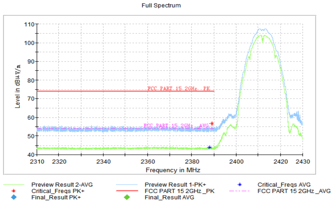
Fig.A.5.9 Band Edges (802.11b, Ch 1, 2.31GHz – 2.43GHz)
