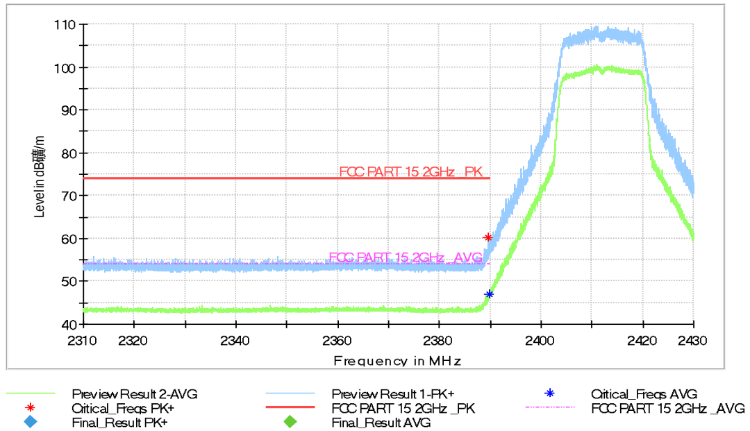
Fig.A.5.11 Band Edges (802.11g, Ch 1, 2.31GHz – 2.43GHz)
