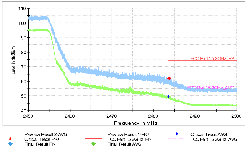
Fig.A.5.22 Band Edges (802.11n-HT40, Ch 6, 2.45 GHz – 2.5GHz)
