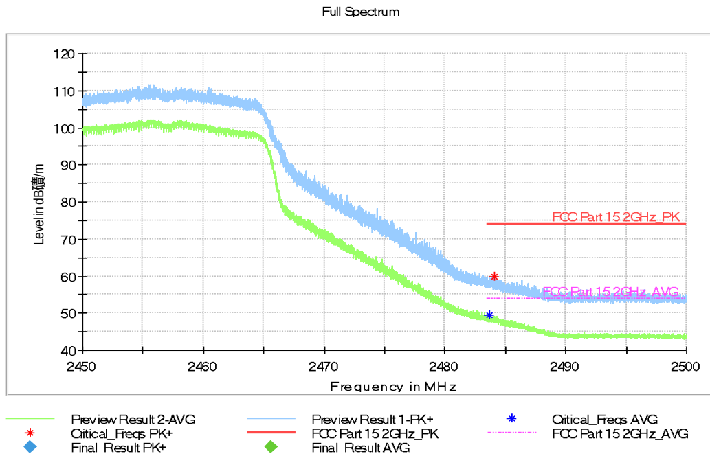
Fig.A.5.13 Band Edges (802.11g, Ch 10, 2.45 GHz – 2.5GHz)
