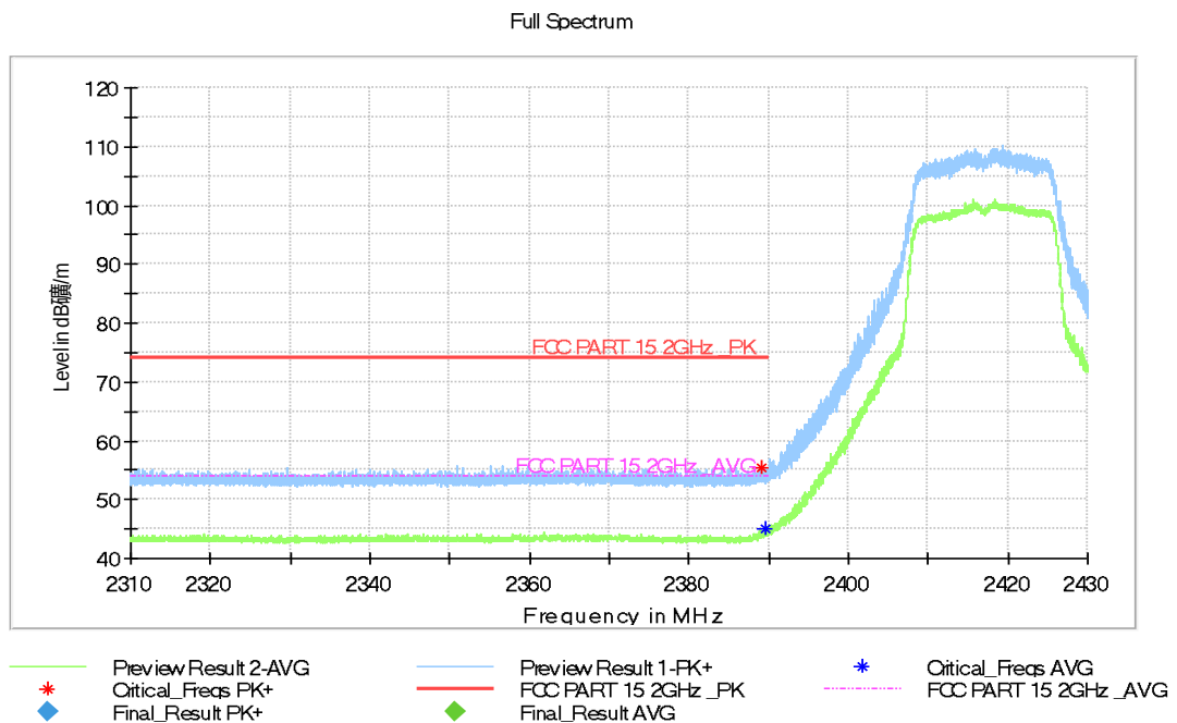
Fig.A.5.16 Band Edges (802.11n-HT20, Ch 2, 2.31 GHz – 2.43GHz)
