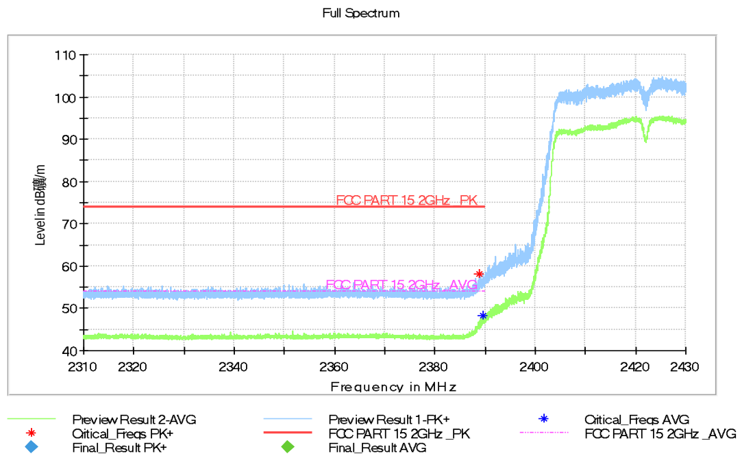
Fig.A.5.20 Band Edges (802.11n-HT40, Ch 3, 2.31 GHz – 2.43GHz)
