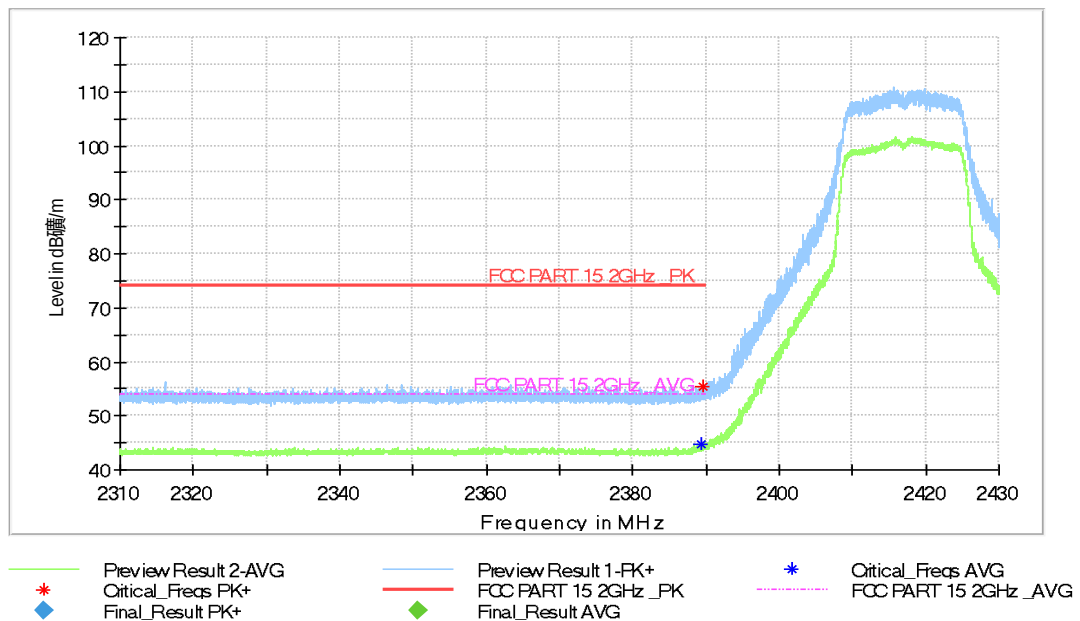
Fig.A.5.12 Band Edges (802.11g, Ch 2, 2.31 GHz – 2.43GHz)
