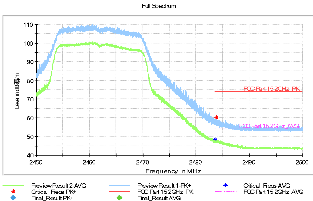
Fig.A.5.14 Band Edges (802.11g, Ch 11, 2.45 GHz – 2.5GHz)
