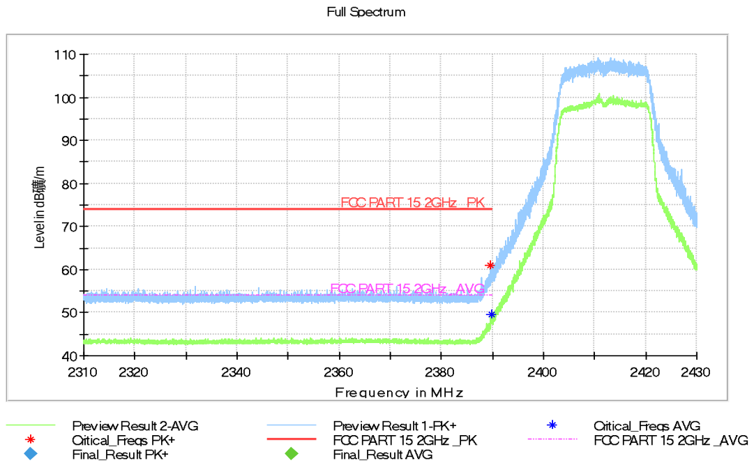
Fig.A.5.15 Band Edges (802.11n-HT20, Ch 1, 2.31GHz – 2.43GHz)
