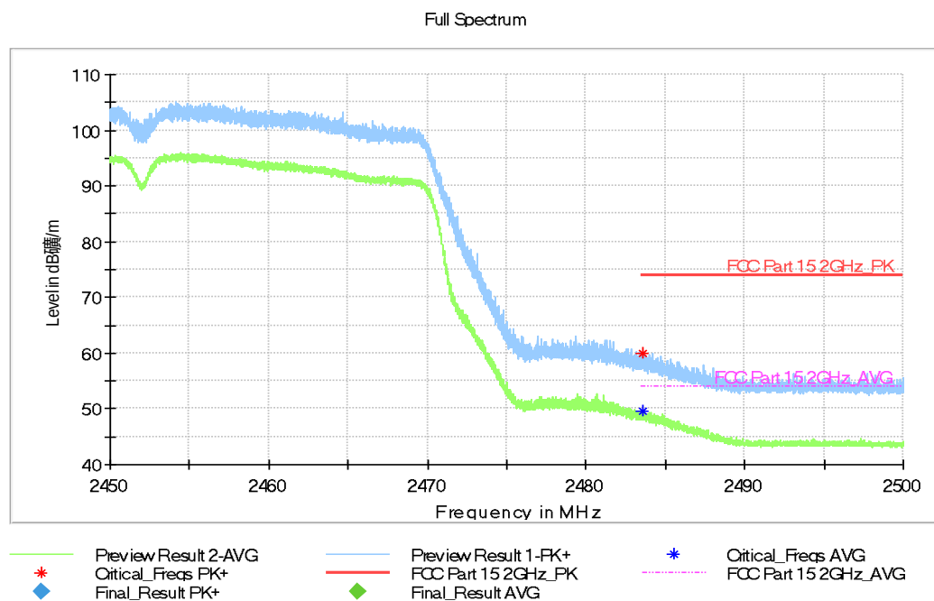
Fig.A.5.25 Band Edges (802.11n-HT40, Ch 9, 2.45 GHz – 2.5GHz)
