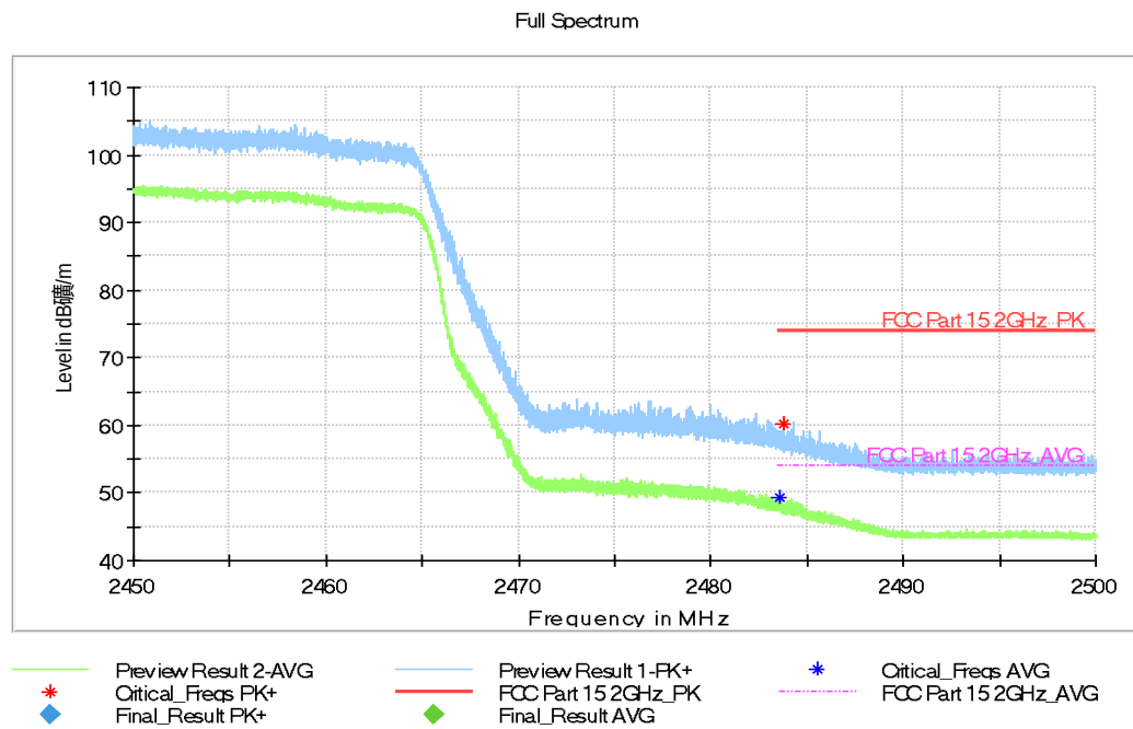
Fig.A.5.24 Band Edges (802.11n-HT40, Ch 8, 2.45 GHz – 2.5GHz)
