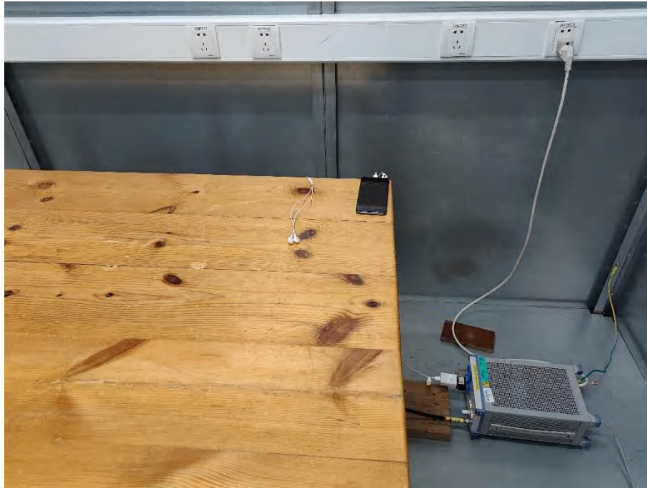
19. Conducted Emission (Part 15C&E, Bluetooth/Wi-Fi)
