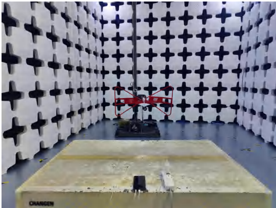
10. Radiated Emissions (Part 15C, 30MHz-1GHz)
