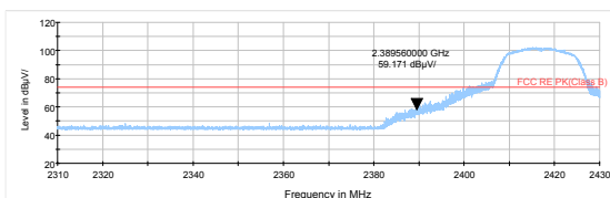
802.11g-Channel 2 Peak
