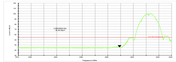
802.11b-Channel 1 Average
