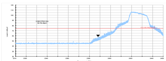
802.11g-Channel 4 Peak
