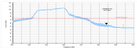
802.11g-Channel 9 Peak
