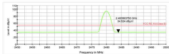
BLE (1M) Channel 39 Average
