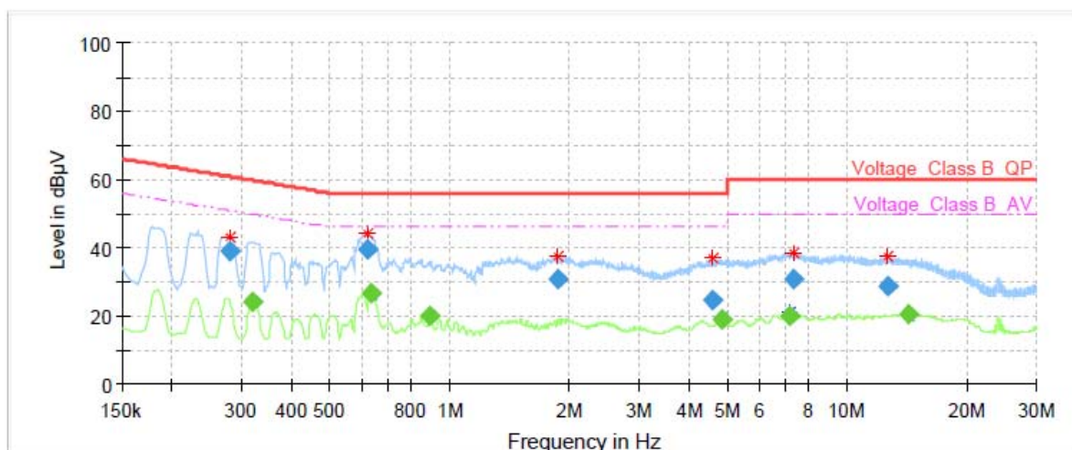
N line Conducted Emission from 150 KHz to 30 MHz
