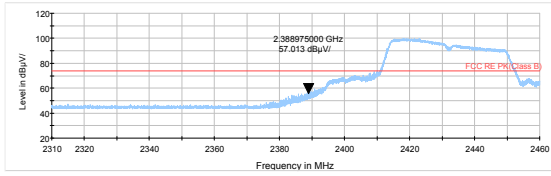
802.11n HT40 -Channel 5 Peak
