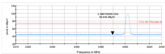
BLE (1M) Channel 0 Peak
