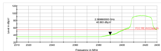
802.11g-Channel 2 Average
