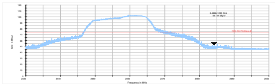
802.11g-Channel 10 Peak
