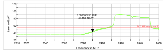
802.11n HT40 -Channel 5 Average
