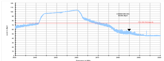
802.11n HT20 -Channel 9 Peak
