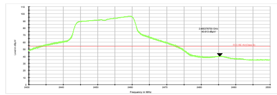
802.11g-Channel 9 Average
