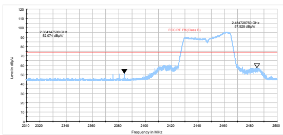
802.11n HT40 -Channel 8 Peak
