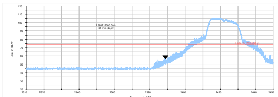
802.11g-Channel 3 Peak
