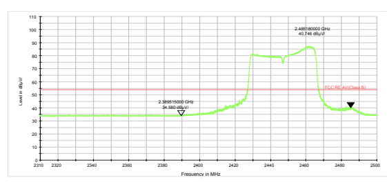
802.11n HT40 -Channel 8 Average
