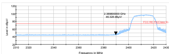
802.11g-Channel 1 Peak
