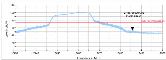
802.11n HT20 -Channel 10 Peak
