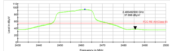
802.11g-Channel 10 Average
