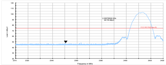
802.11b-Channel 1 Peak
