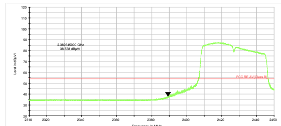
802.11n HT40 -Channel 4 Average
