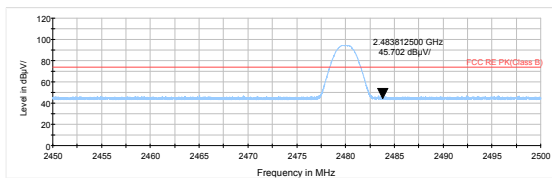
BLE (1M) Channel 39 Peak
