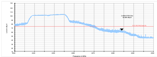
802.11n HT20 -Channel 8 Peak
