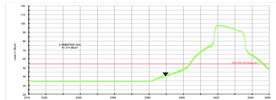
802.11g-Channel 4 Average
