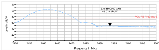
802.11b-Channel 11 Peak
