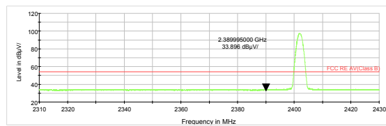
BLE (1M) Channel 0 Average
