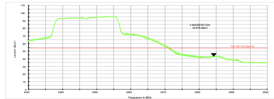
802.11n HT20 -Channel 8 Average
