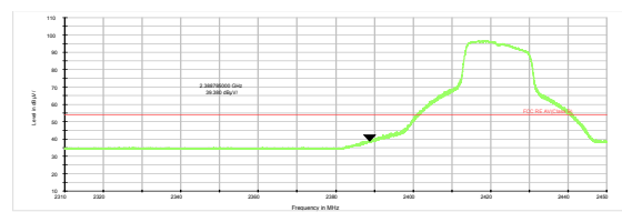
802.11g-Channel 3 Average
