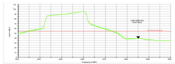
802.11n HT20 -Channel 9 Average
