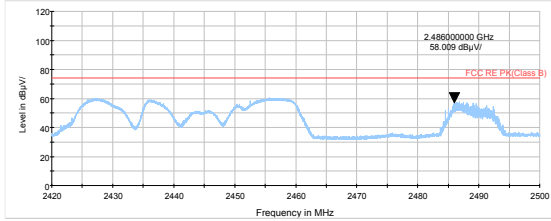
802.11n HT40 -Channel 7 Peak
