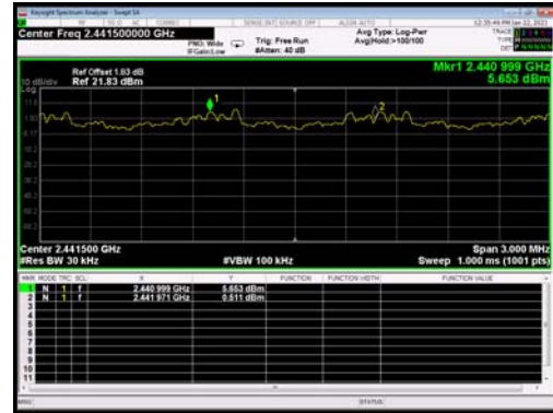
BT 3DH5 CH39, Carrier frequency (MHz): 2441
