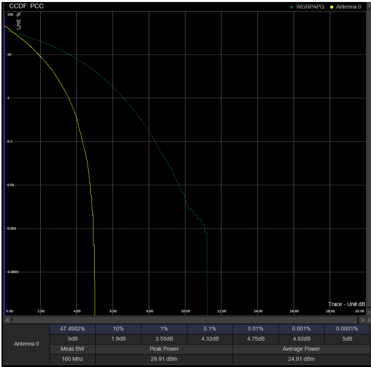
PAPR/PC2\N78(3450-3550)\90M DFT 633666 100%RB QPSK
