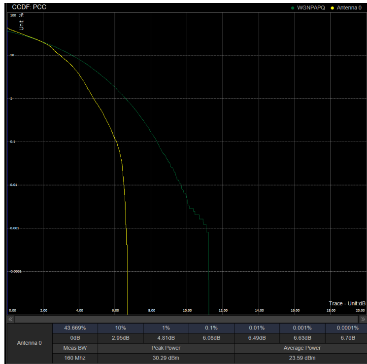
PAPR/PC2\N78(3450-3550)\50M DFT 635000 100%RB 16QAM
