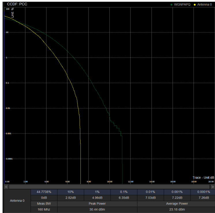
PAPR/PC2\N78(3450-3550)\60M DFT 632000 100%RB 256QAM
