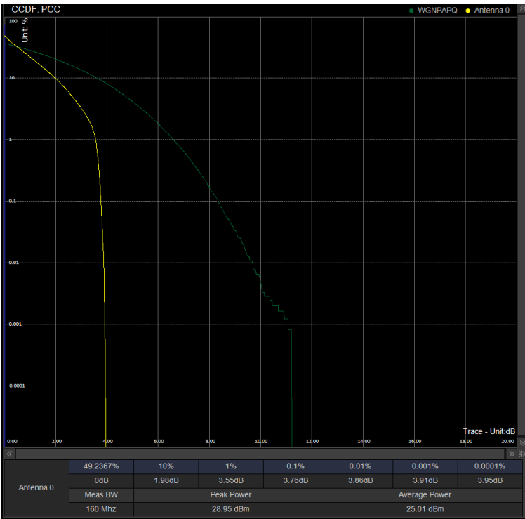
PAPR/PC2\N78(3450-3550)\50M DFT 635000 100%RB BPSK
