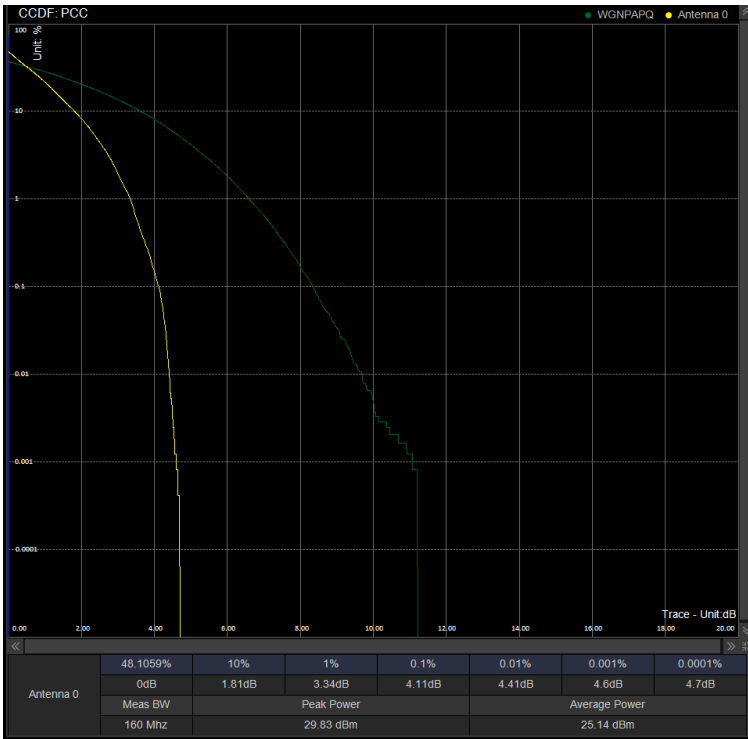
PAPR/PC2\N78(3450-3550)\60M DFT 633334 100%RB BPSK
