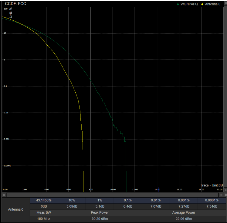
PAPR/PC2\N78(3450-3550)\80M DFT 632668 100%RB 256QAM
