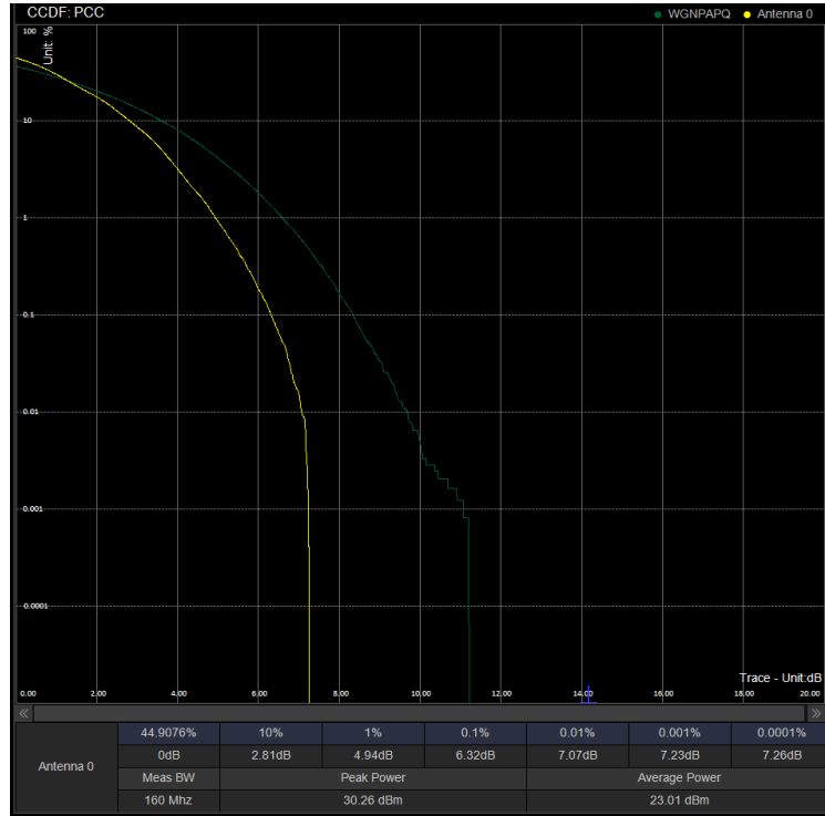
PAPR/PC2\N78(3450-3550)\60M DFT 634666 100%RB 64QAM
