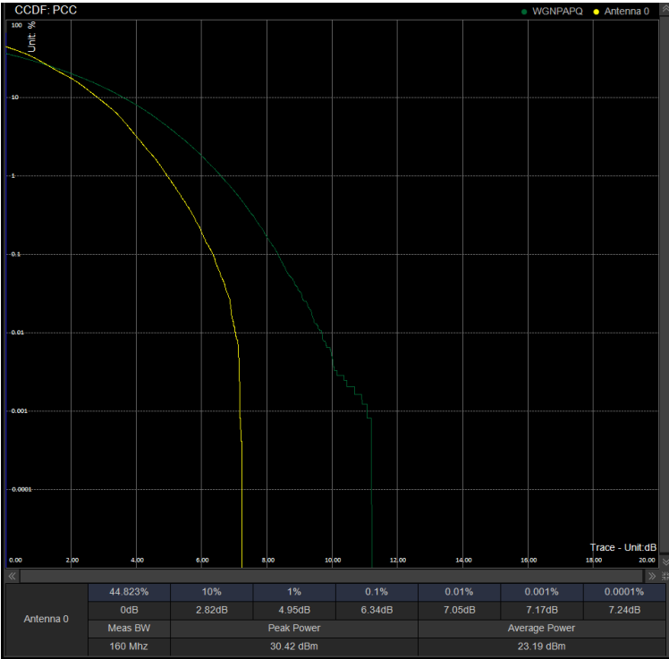
PAPR/PC2\N78(3450-3550)\60M DFT 632000 100%RB 64QAM
