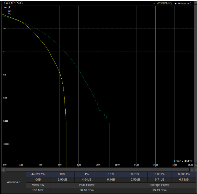
PAPR/PC2\N78(3450-3550)\80M DFT 634000 100%RB 16QAM
