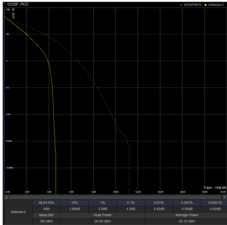
PAPR/PC2\N78(3450-3550)\50M DFT 633334 100%RB BPSK
