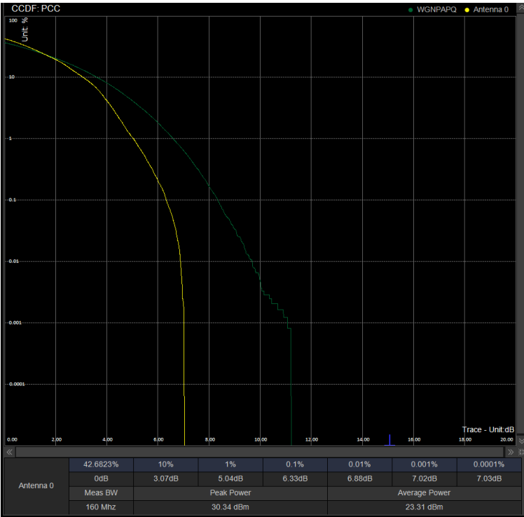
PAPR/PC2\N78(3450-3550)\50M DFT 631668 100%RB 64QAM
