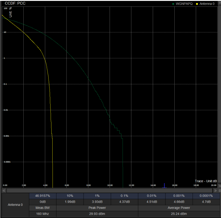
PAPR/PC2\N78(3450-3550)\50M DFT 631668 100%RB BPSK
