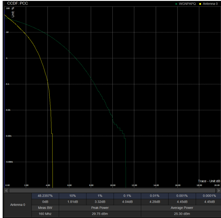
PAPR/PC2\N78(3450-3550)\60M DFT 632000 100%RB QPSK
