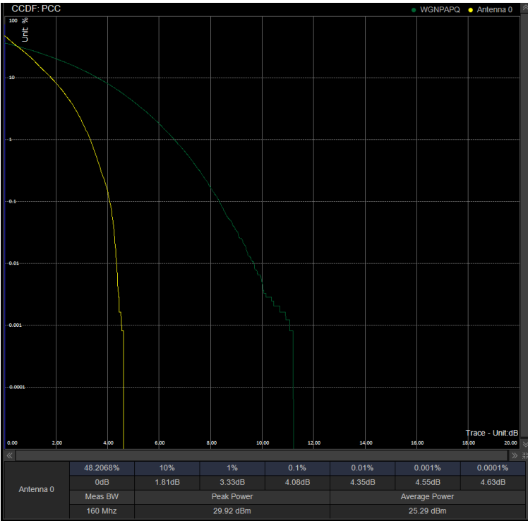
PAPR/PC2\N78(3450-3550)\60M DFT 632000 100%RB BPSK
