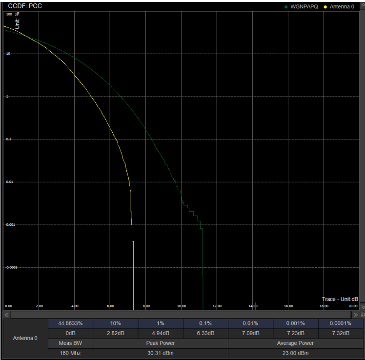
PAPR/PC2\N78(3450-3550)\60M DFT 634666 100%RB 256QAM
