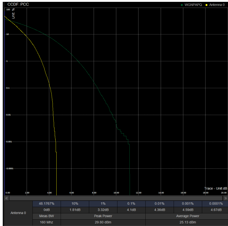
PAPR/PC2\N78(3450-3550)\60M DFT 634666 100%RB BPSK
