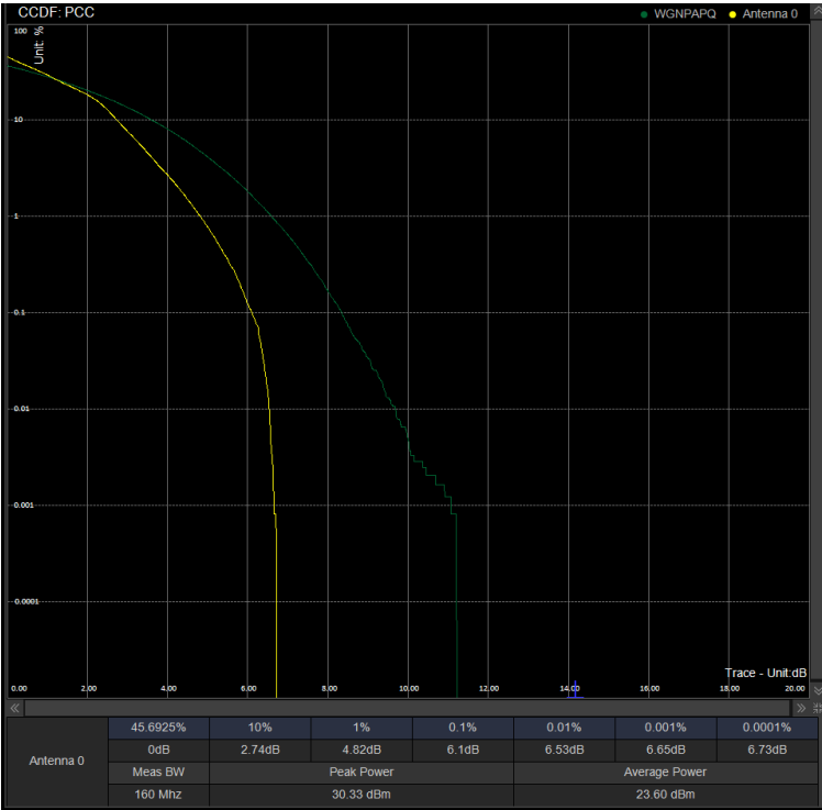
PAPR/PC2\N78(3450-3550)\60M DFT 634666 100%RB 16QAM
