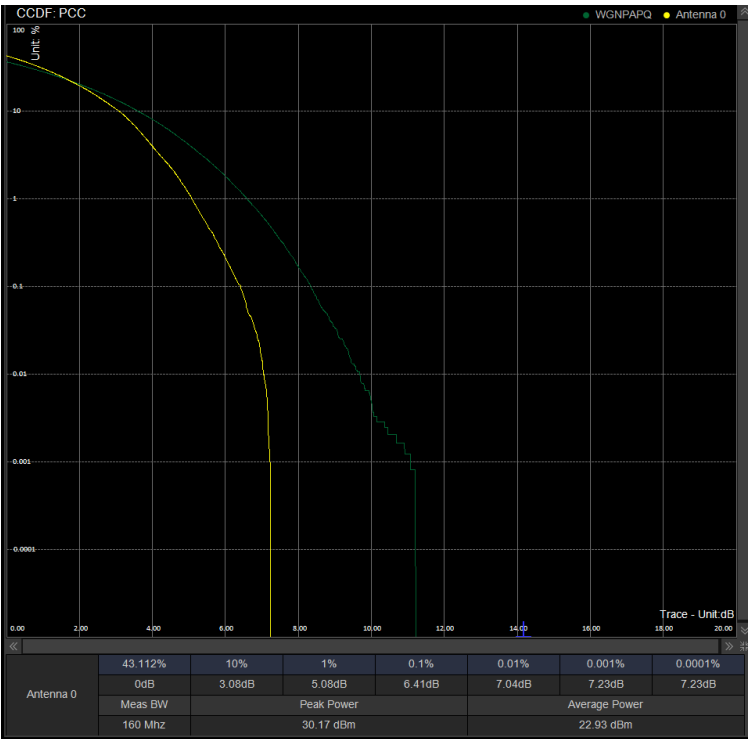
PAPR/PC2\N78(3450-3550)\80M DFT 634000 100%RB 64QAM
