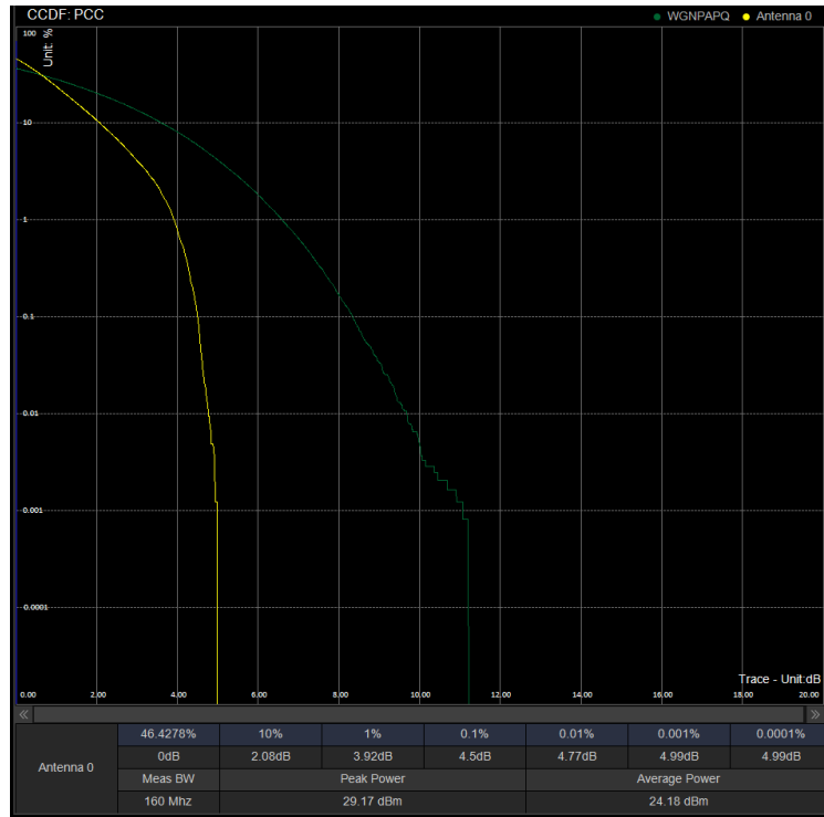
PAPR/PC2\N41\50M DFT 518598 100%RB BPSK
