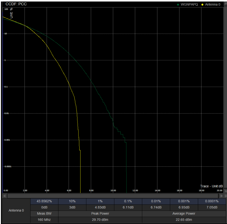
PAPR/PC2\N41\50M DFT 532998 100%RB 16QAM
