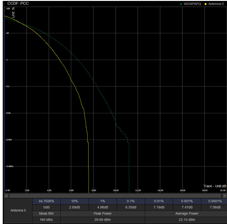
PAPR/PC2\N41\60M DFT 531996 100%RB 256QAM
