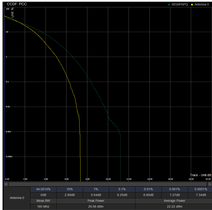
PAPR/PC2\N41\40M DFT 518598 100%RB 256QAM
