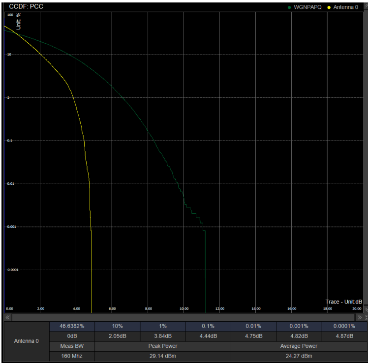
PAPR/PC2\N41\50M DFT 504204 100%RB QPSK
