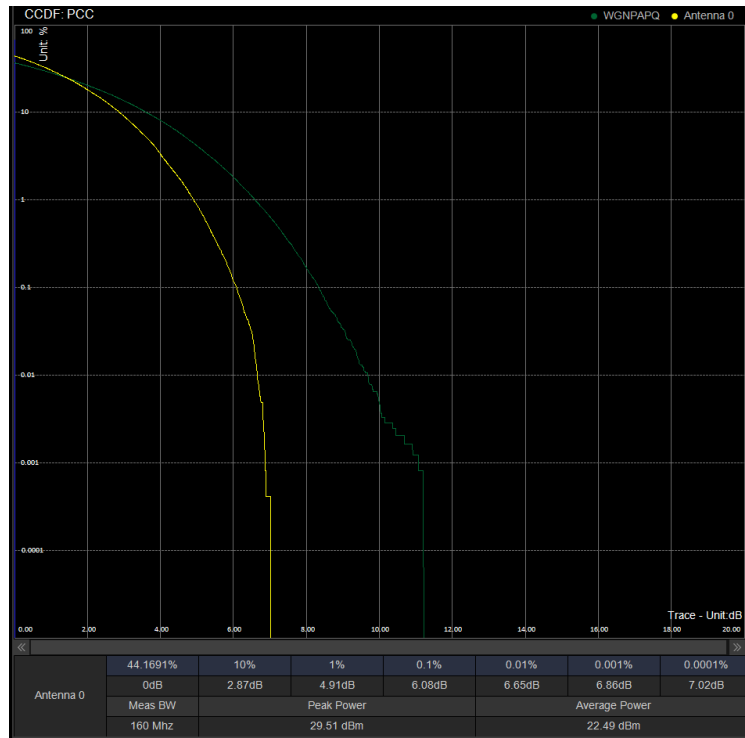
PAPR/PC2\N41\40M DFT 503202 100%RB 64QAM
