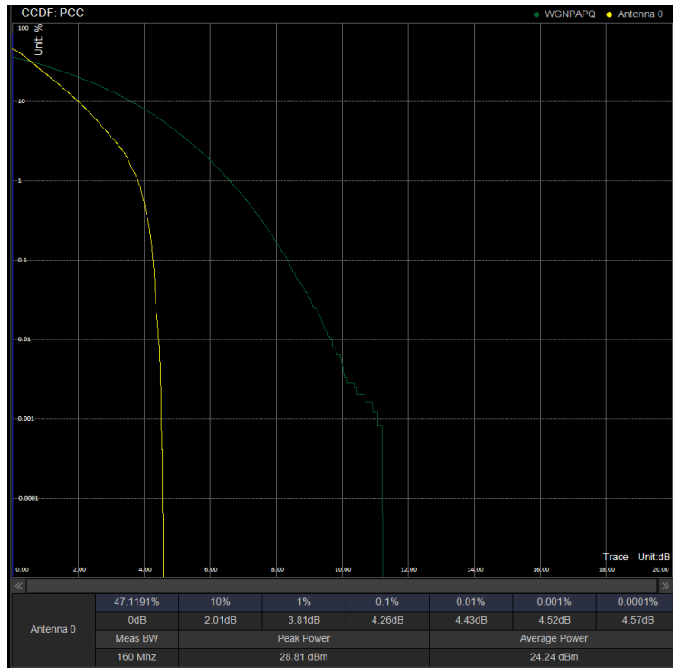
PAPR/PC2\N41\50M DFT 532998 100%RB BPSK
