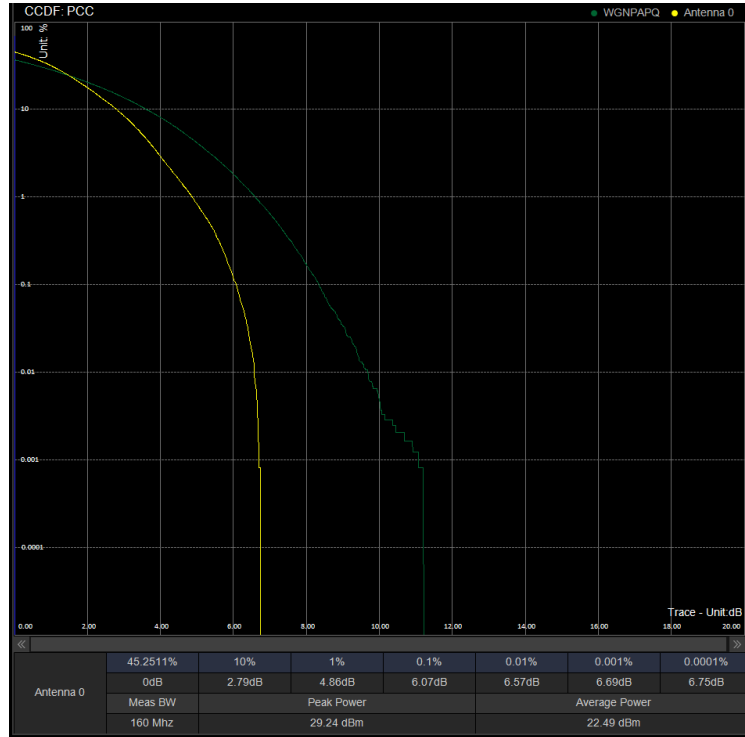
PAPR/PC2\N41\30M DFT 502200 100%RB 64QAM
