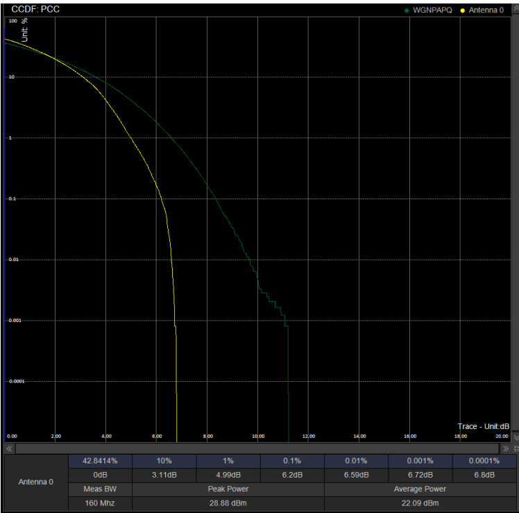
PAPR/PC2\N41\50M DFT 518598 100%RB 256QAM
