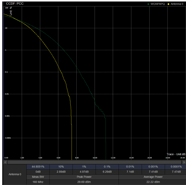
PAPR/PC2\N41\60M DFT 531996 100%RB 64QAM
