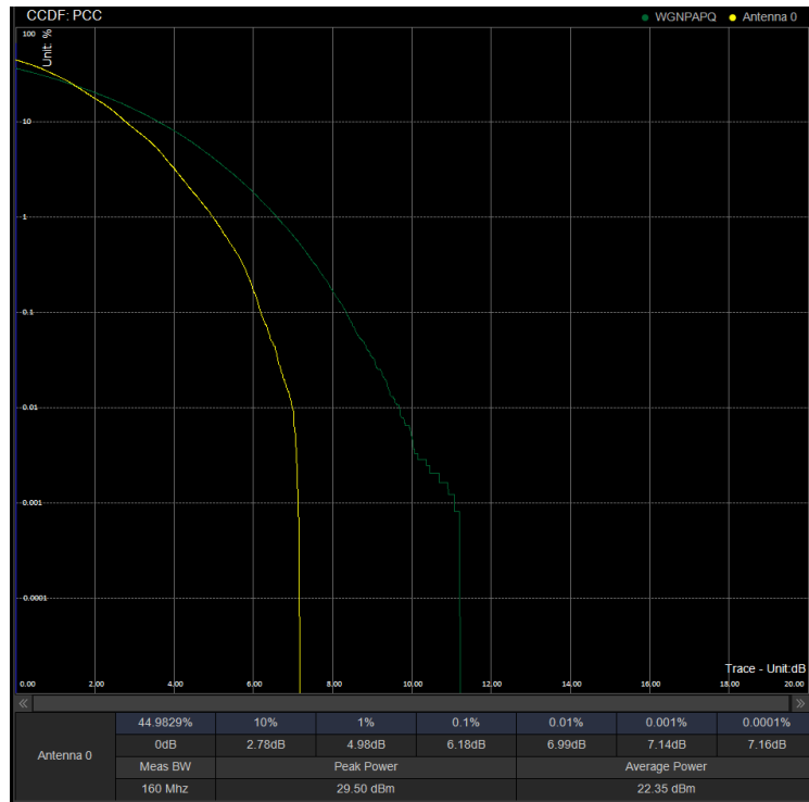
PAPR/PC2\N41\30M DFT 534996 100%RB 256QAM
