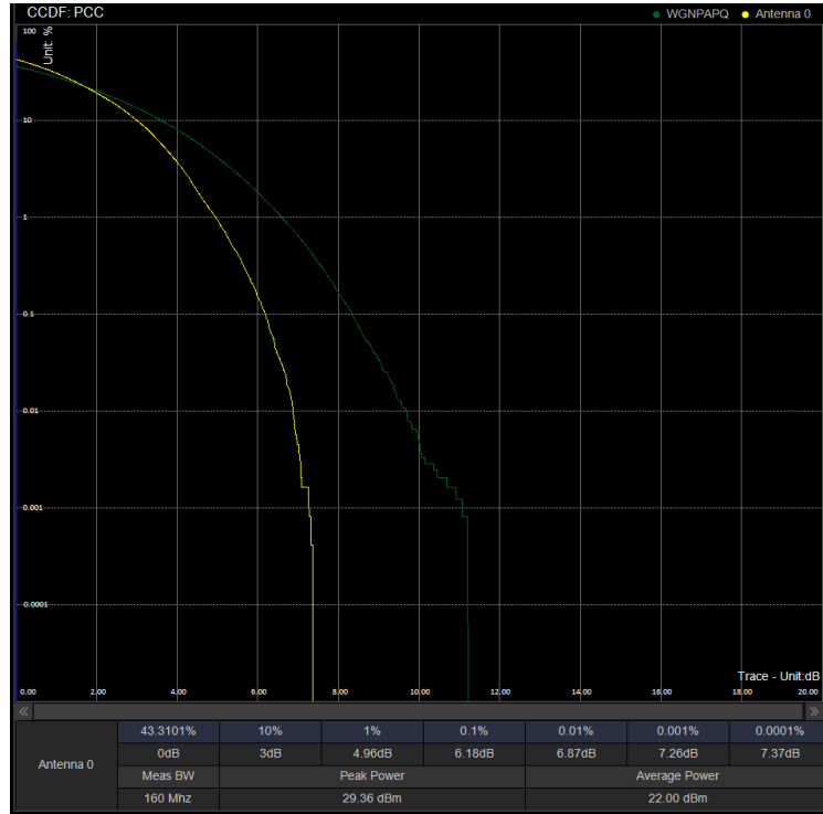
PAPR/PC2\N41\70M DFT 506202 100%RB 64QAM
