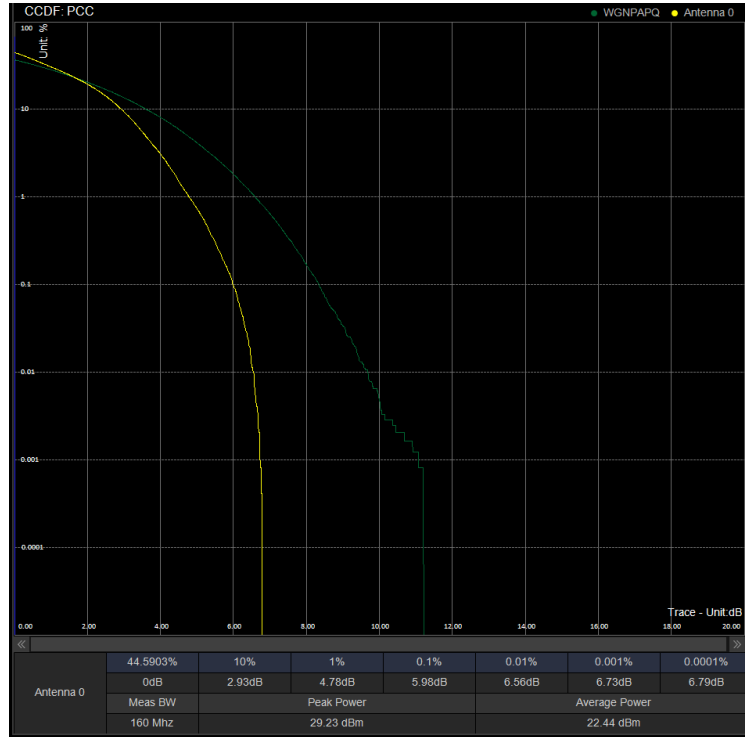
PAPR/PC2\N41\70M DFT 506202 100%RB 16QAM
