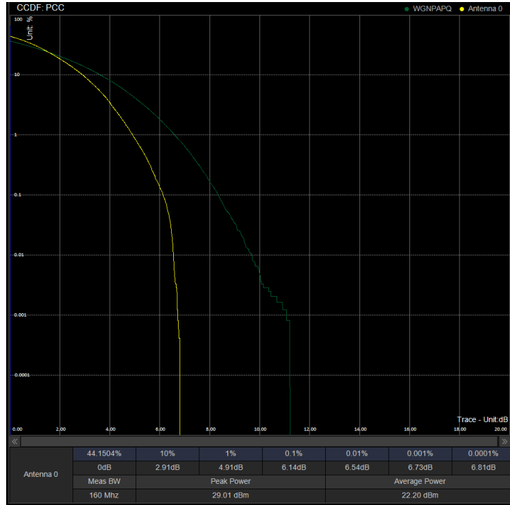
PAPR/PC2\N41\60M DFT 518598 100%RB 64QAM
