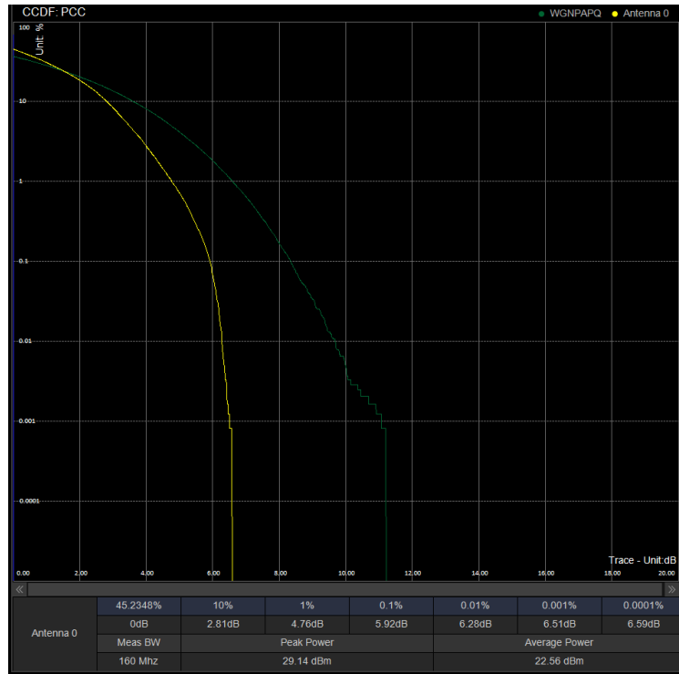
PAPR/PC2\N41\60M DFT 518598 100%RB 16QAM
