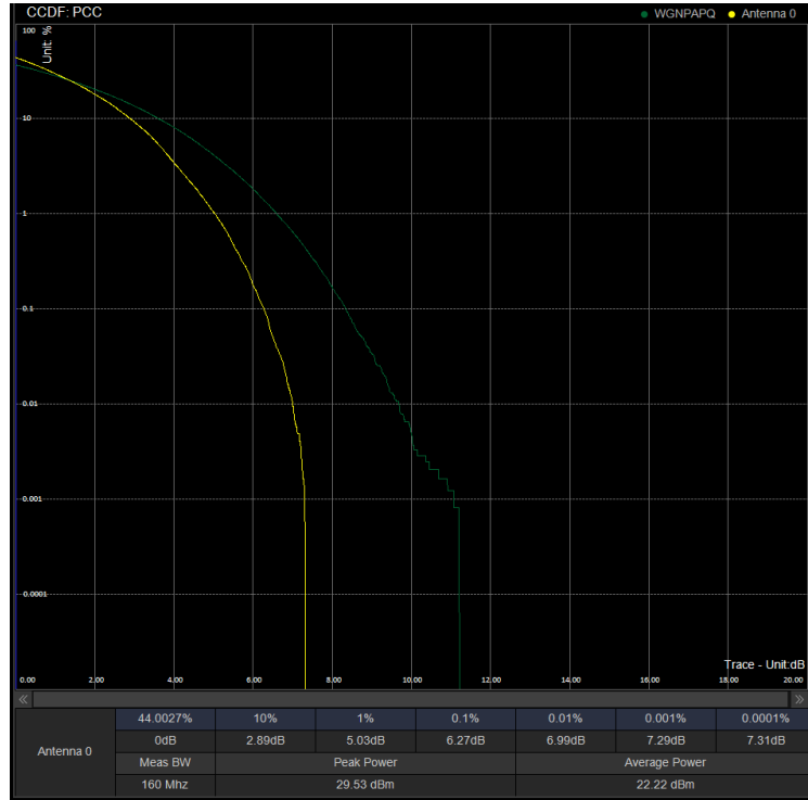
PAPR/PC2\N41\40M DFT 518598 100%RB 64QAM
