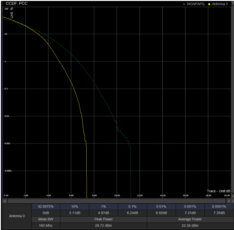
PAPR/PC2\N41\50M DFT 504204 100%RB 64QAM
