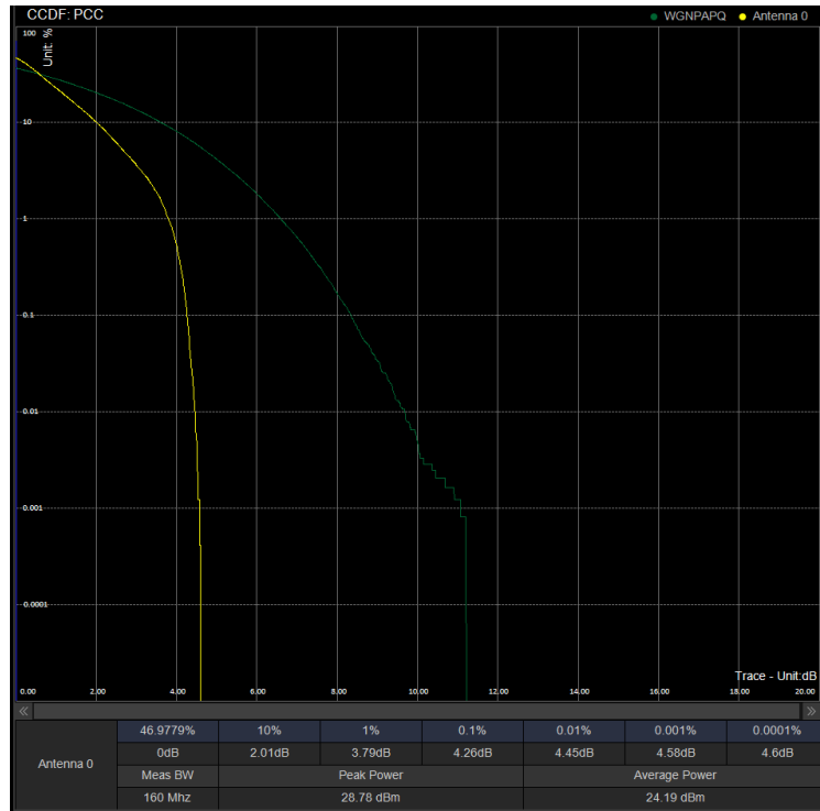
PAPR/PC2\N41\50M DFT 532998 100%RB QPSK
