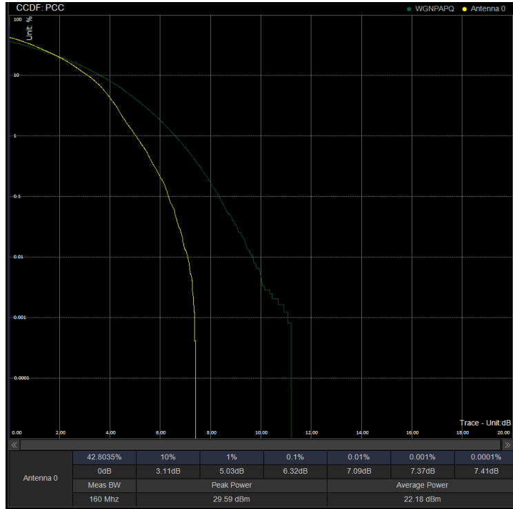
PAPR/PC2\N41\50M DFT 532998 100%RB 64QAM
