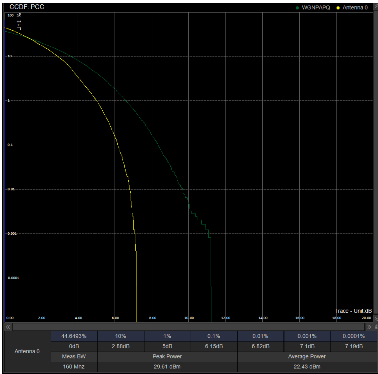
PAPR/PC2\N41\40M DFT 534000 100%RB 256QAM
