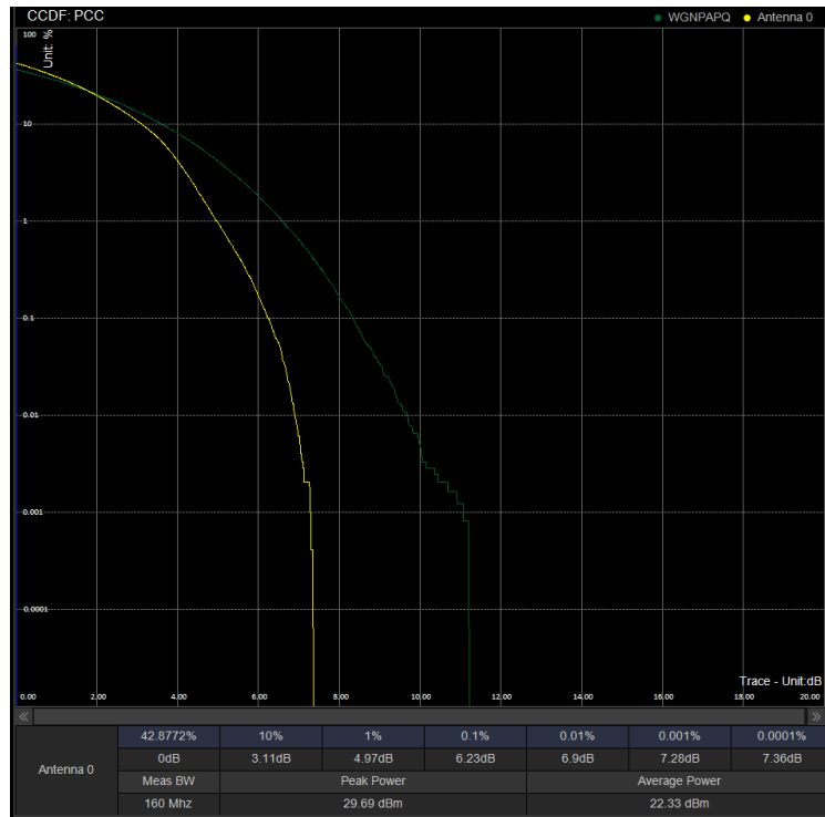
PAPR/PC2\N41\50M DFT 504204 100%RB 256QAM
