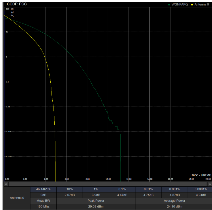
PAPR/PC2\N41\50M DFT 518598 100%RB QPSK
