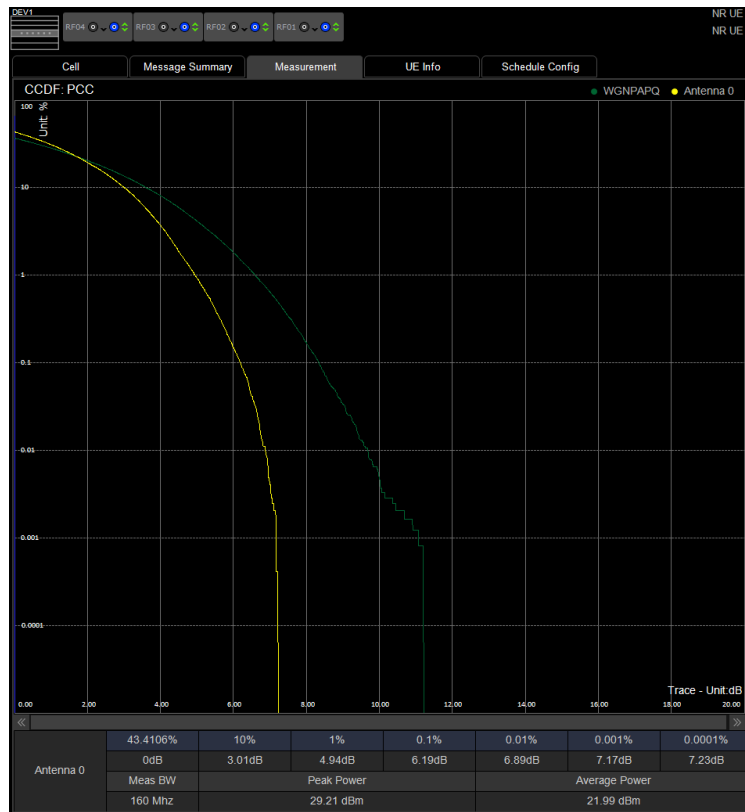
PAPR/PC2\N41\70M DFT 506202 100%RB 256QAM
