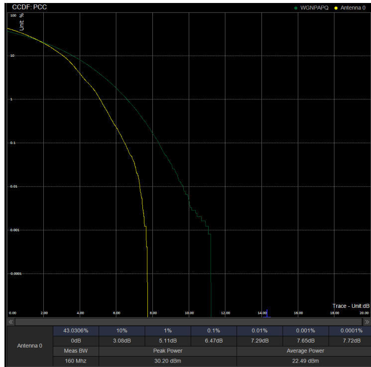
PAPR/PC3\N78(3450-3550)\80M DFT 633334 100%RB 256QAM
