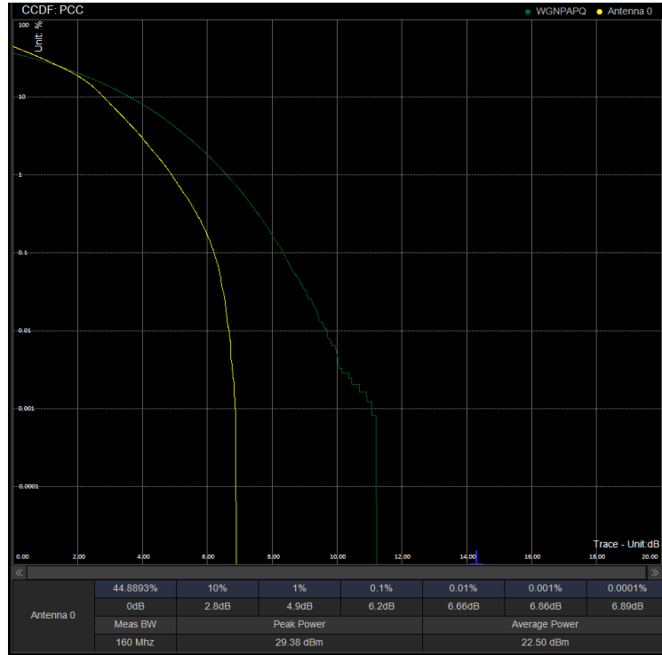
PAPR/PC3\N78(3450-3550)\90M DFT 633000 100%RB 16QAM
