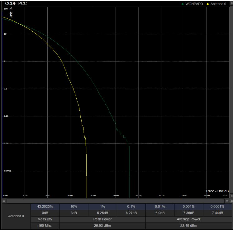
PAPR/PC2\N41\100M DFT 528000 100%RB 16QAM
