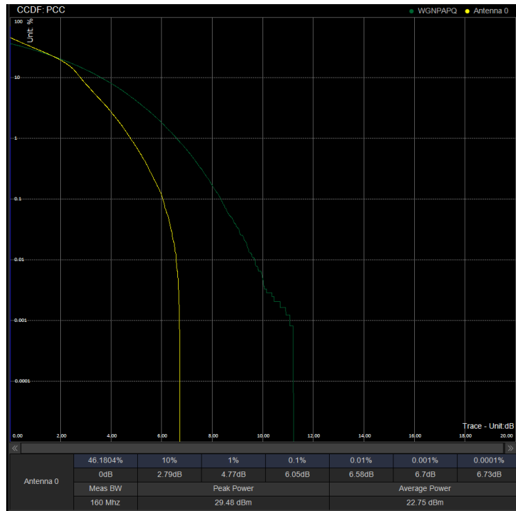
PAPR/PC2\N41\20M DFT 535998 100%RB 16QAM
