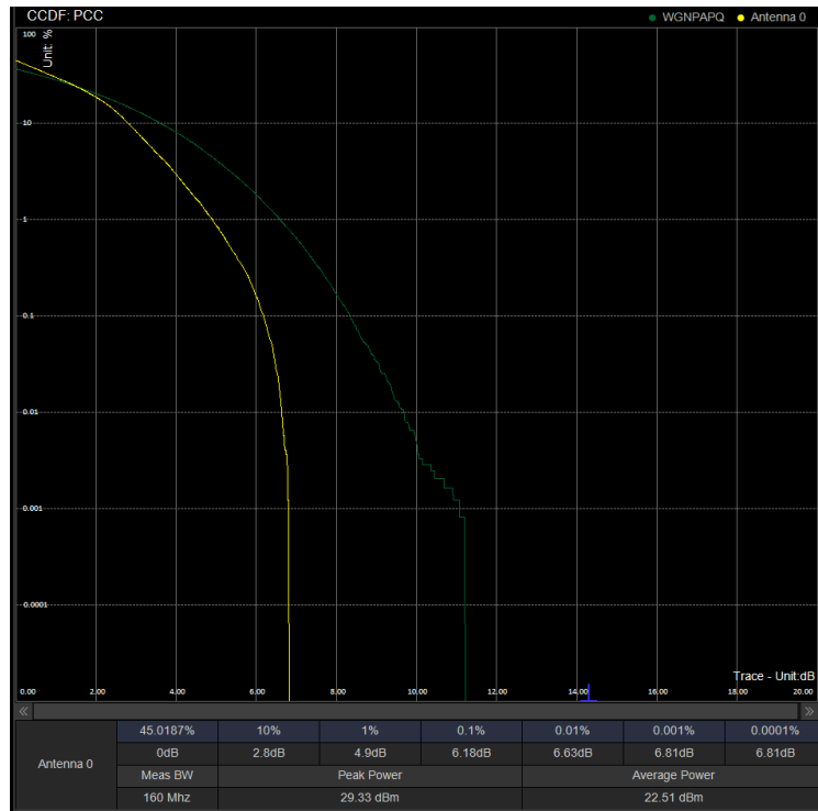
PAPR/PC3\N78(3450-3550)\90M DFT 633334 100%RB 16QAM
