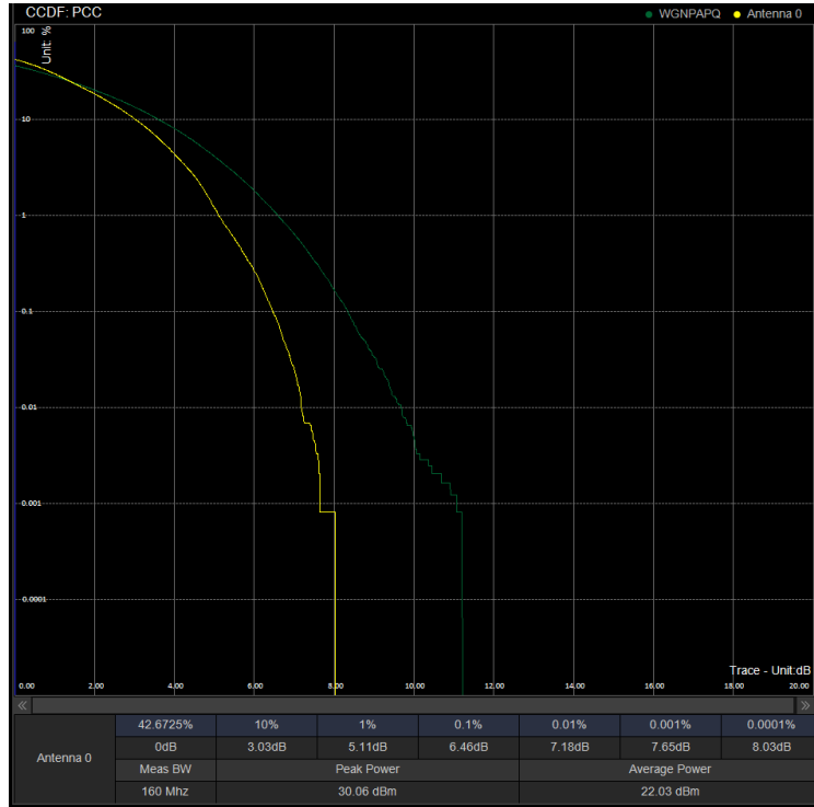
PAPR/PC2\N41\100M DFT 518598 100%RB 256QAM
