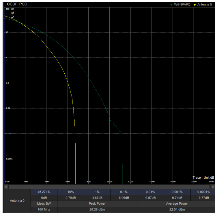
PAPR/PC2\N41\30M DFT 502200 100%RB 256QAM
