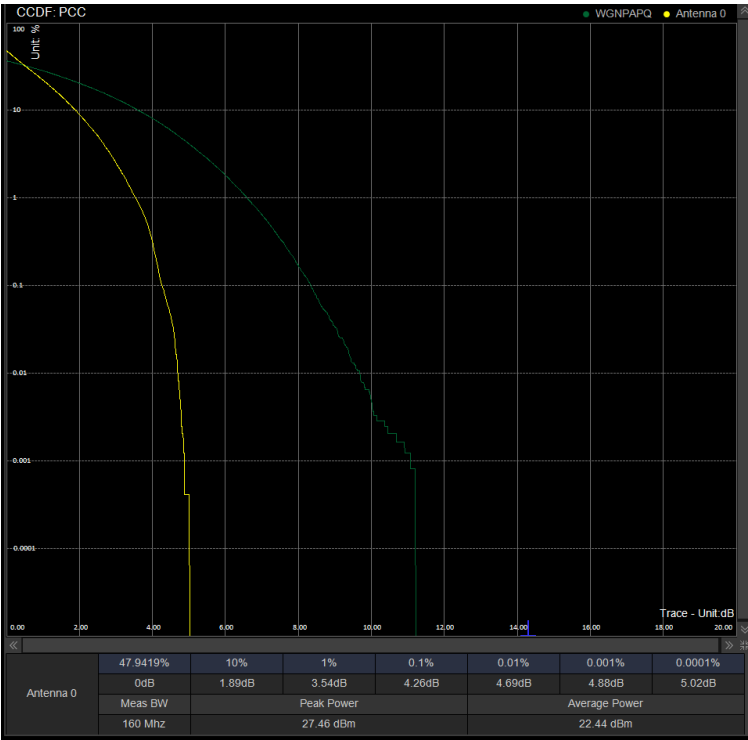
PAPR/PC3\N78(3450-3550)\90M DFT 633334 100%RB QPSK
