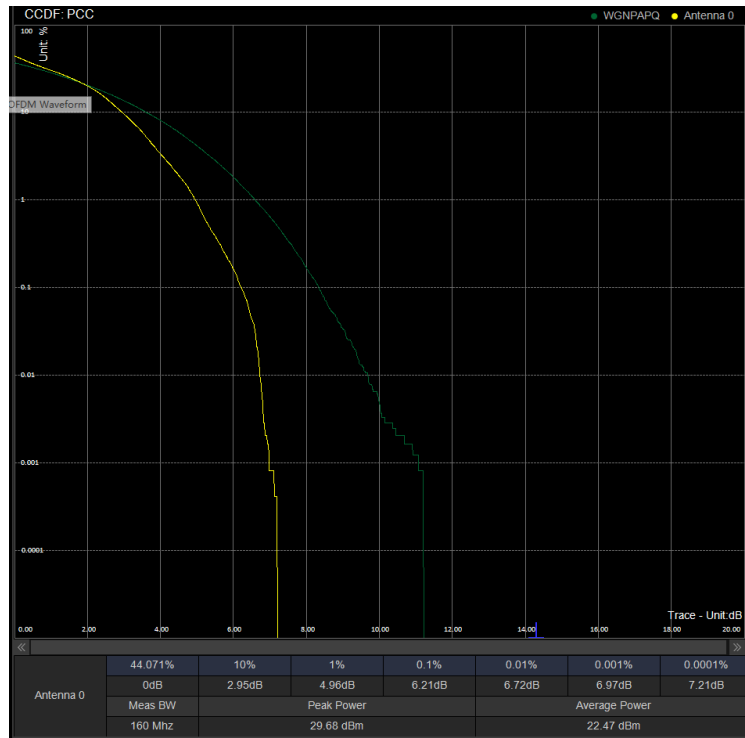
PAPR/PC3\N78(3450-3550)\80M DFT 634000 100%RB 16QAM
