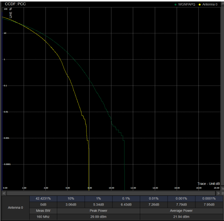
PAPR/PC2\N41\100M DFT 528000 100%RB 64QAM
