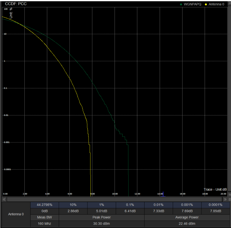
PAPR/PC3\N78(3450-3550)\90M DFT 633666 100%RB 256QAM
