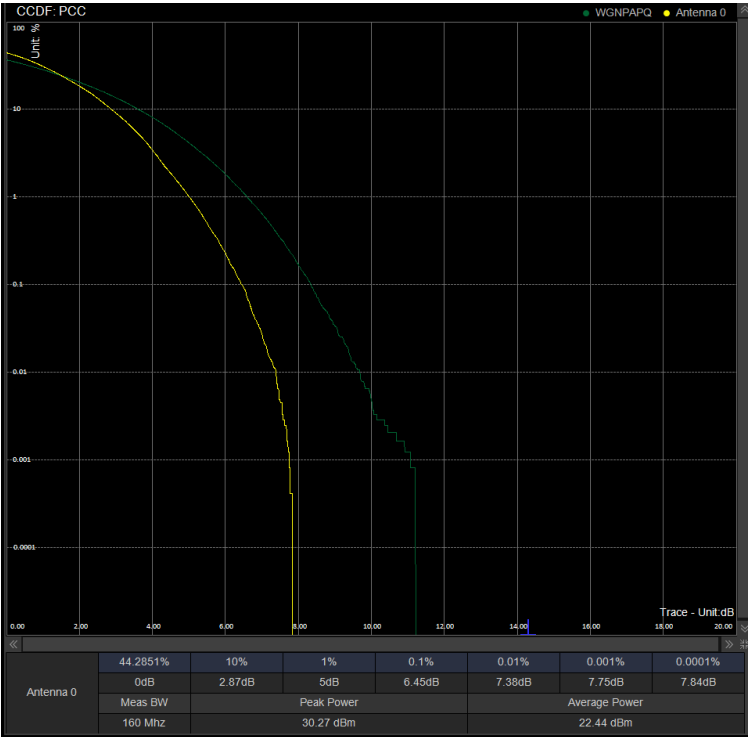
PAPR/PC3\N78(3450-3550)\90M DFT 633334 100%RB 256QAM
