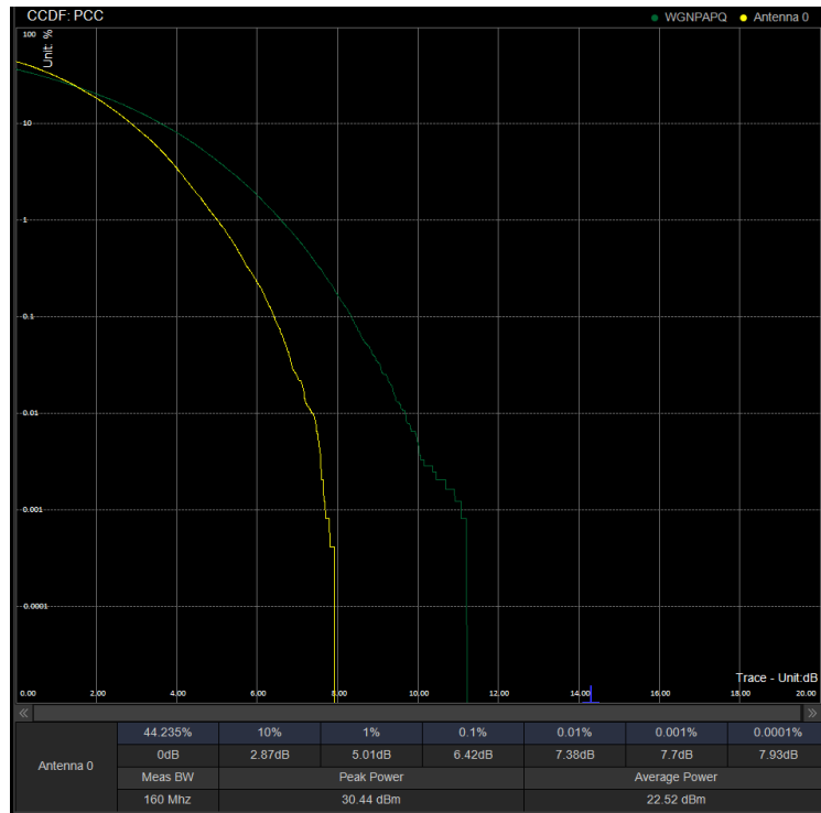
PAPR/PC3\N78(3450-3550)\90M DFT 633000 100%RB 256QAM
