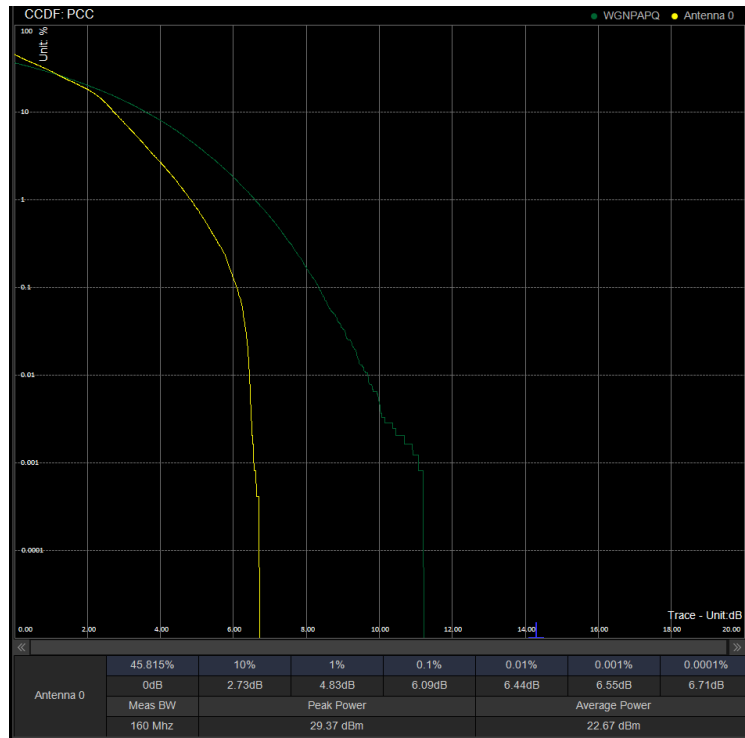
PAPR/PC3\N78(3450-3550)60M DFT 634666 100%RB 16QAM
