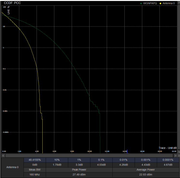
PAPR/PC3\N78(3450-3550)\60M DFT 632000 100%RB QPSK
