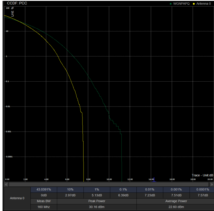
PAPR/PC3\N78(3450-3550)\100M DFT 633334 100%RB 64QAM
