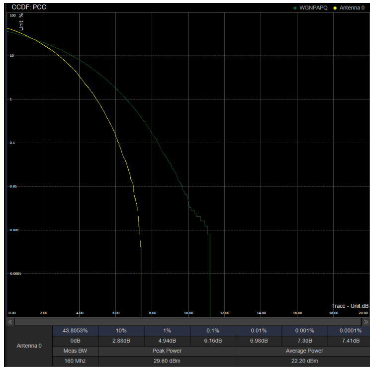
PAPR/PC3\N41\40M DFT 503202 100%RB 64QAM
