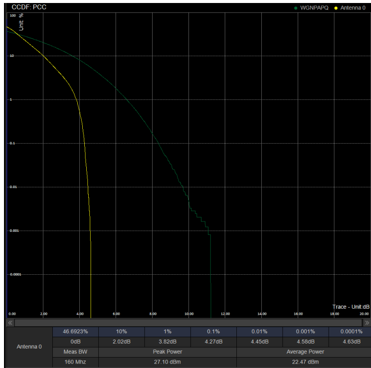
PAPR/PC3\N41\50M DFT 532998 100%RB BPSK
