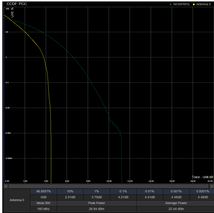
PAPR/PC3\N41\50M DFT 532998 100%RB QPSK
