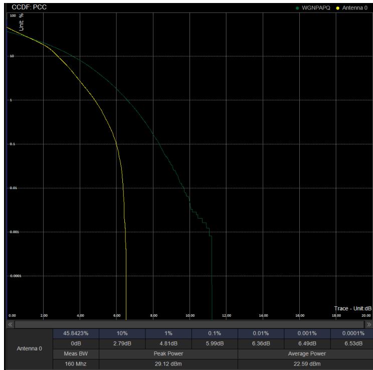
PAPR/PC3\N41\40M DFT 534000 100%RB 16QAM
