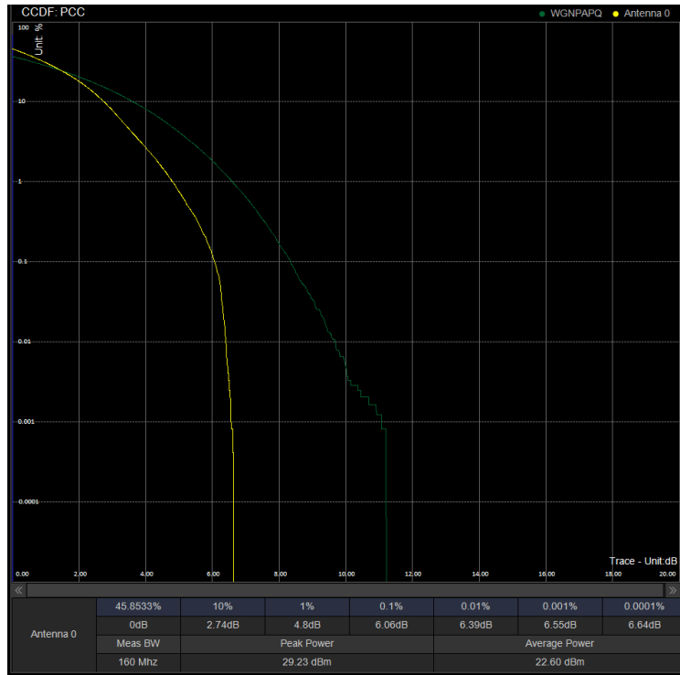
PAPR/PC3\N41\30M DFT 502200 100%RB 16QAM
