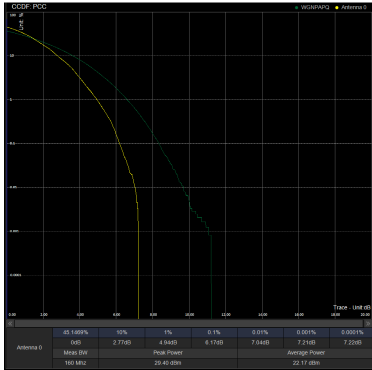
PAPR/PC3\N41\30M DFT 534996 100%RB 64QAM
