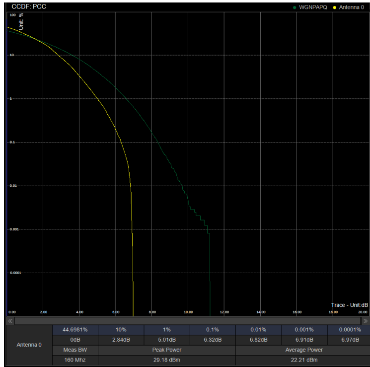
PAPR/PC3\N41\20M DFT 535998 100%RB 256QAM
