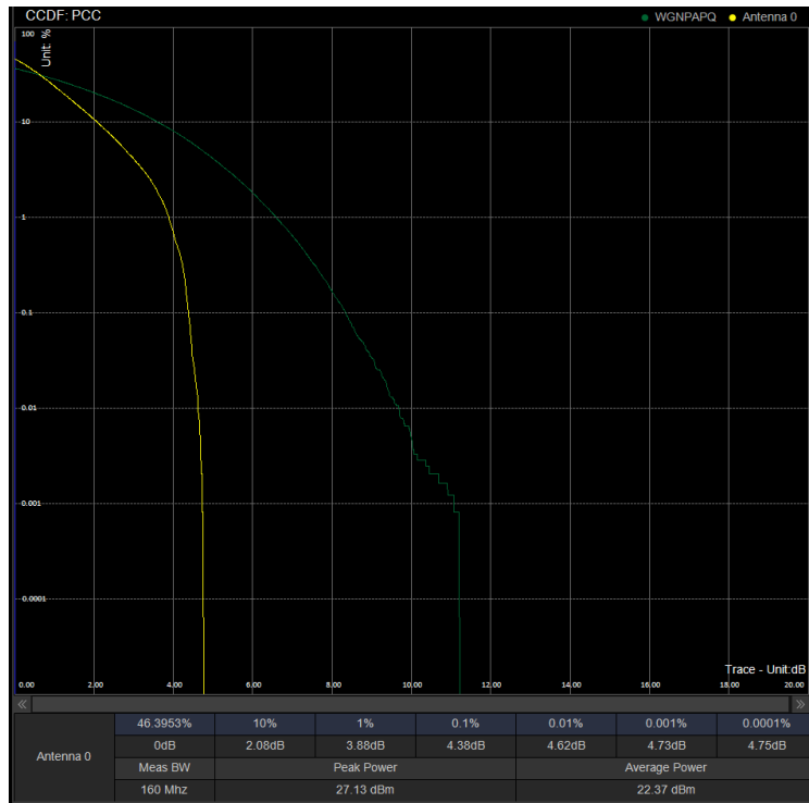
PAPR/PC3\N41\50M DFT 518598 100%RB QPSK
