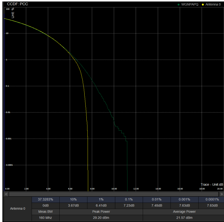
PAPR/PC3\N41\50M CP 532998 100%RB 64QAM
