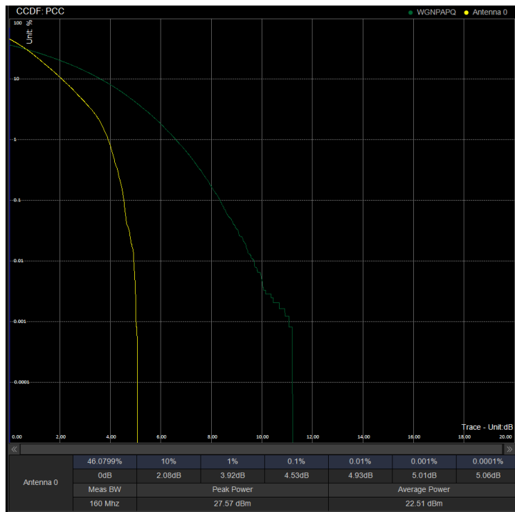
PAPR/PC3\N41\50M DFT 504204 100%RB BPSK
