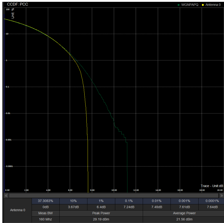
PAPR/PC3\N41\50M CP 532998 100%RB 256QAM
