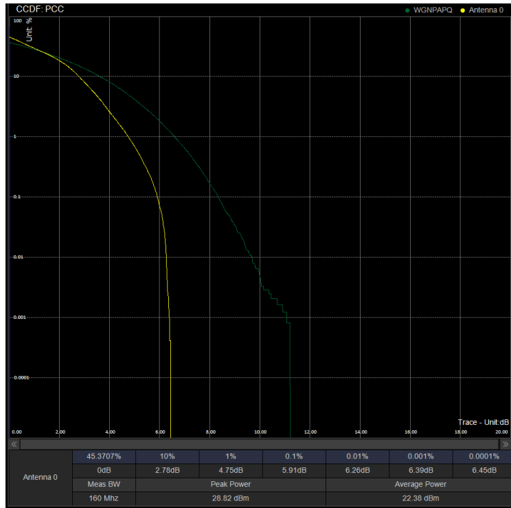
PAPR/PC3\N41\40M DFT 518598 100%RB 16QAM
