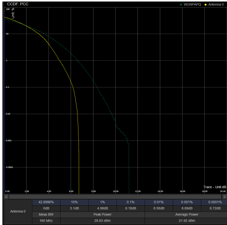
PAPR/PC3\N41\50M DFT 518598 100%RB 256QAM
