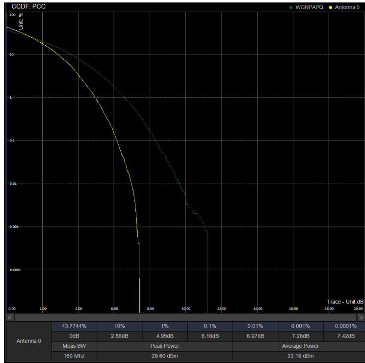
PAPR/PC3\N41\40M DFT 503202 100%RB 256QAM
