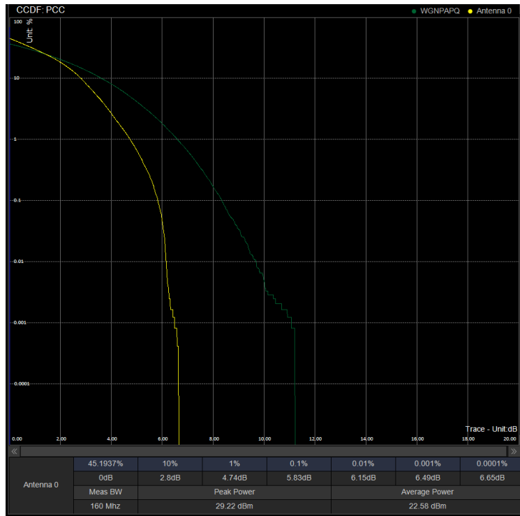
PAPR/PC3\N41\40M DFT 503202 100%RB 16QAM
