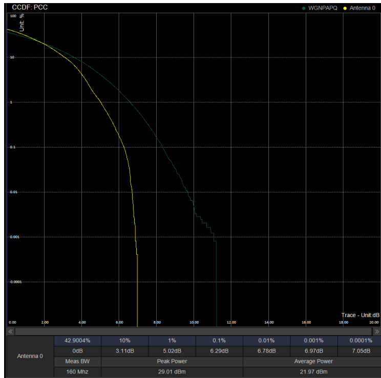
PAPR/PC3\N41\50M DFT 532998 100%RB 256QAM
