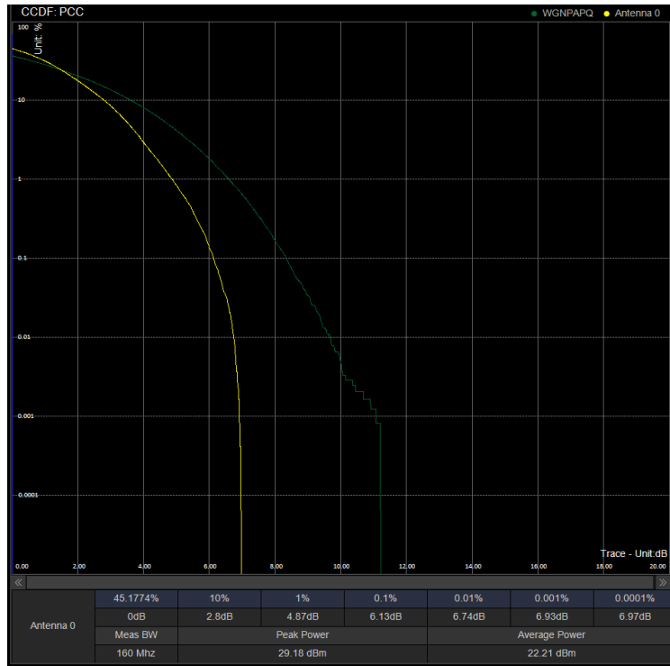
PAPR/PC3\N41\30M DFT 502200 100%RB 64QAM
