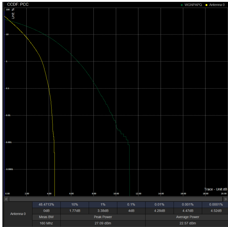
PAPR/PC3\N41\40M DFT 534000 100%RB QPSK
