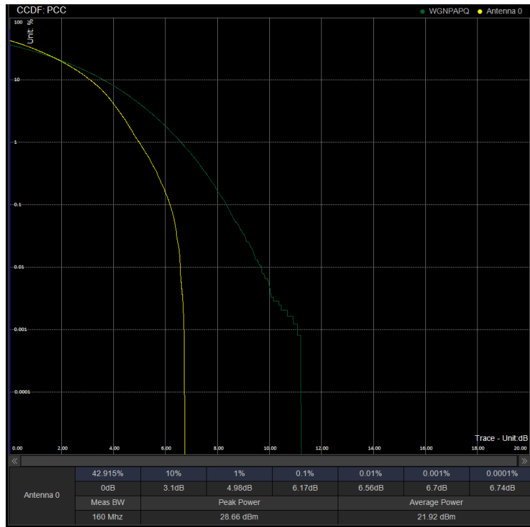
PAPR/PC3\N41\50M DFT 518598 100%RB 64QAM
