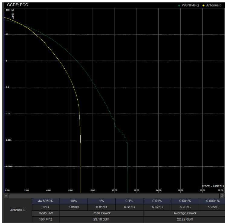
PAPR/PC3\N41\20M DFT 535998 100%RB 64QAM
