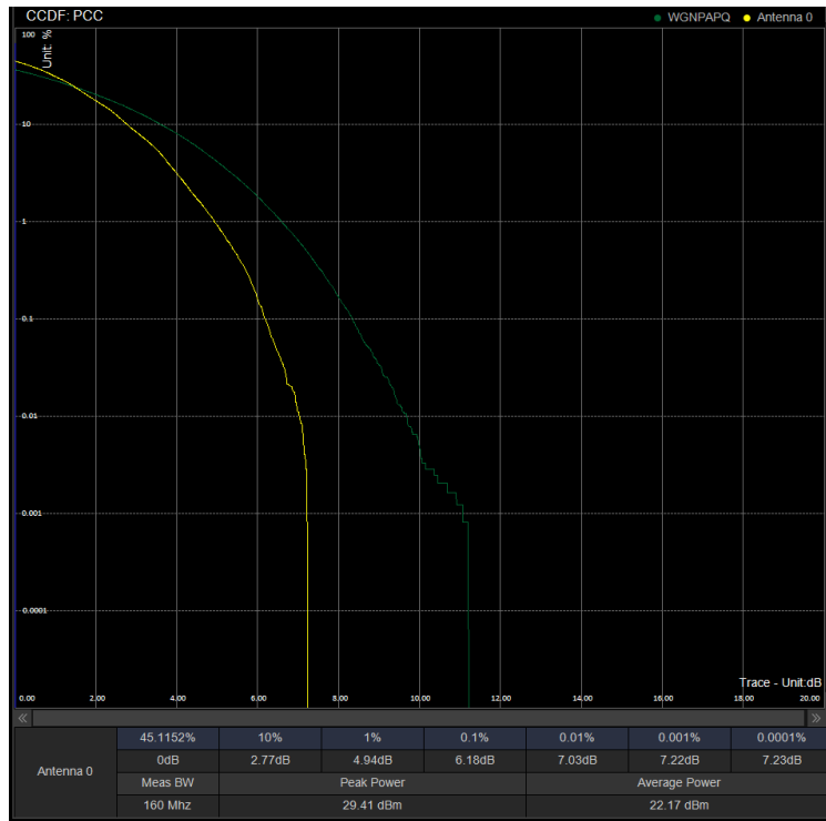
PAPR/PC3\N41\30M DFT 534996 100%RB 256QAM
