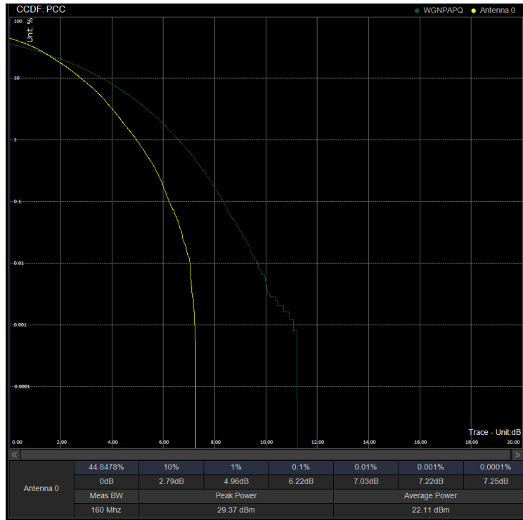
PAPR/PC3\N41\30M DFT 518598 100%RB 256QAM
