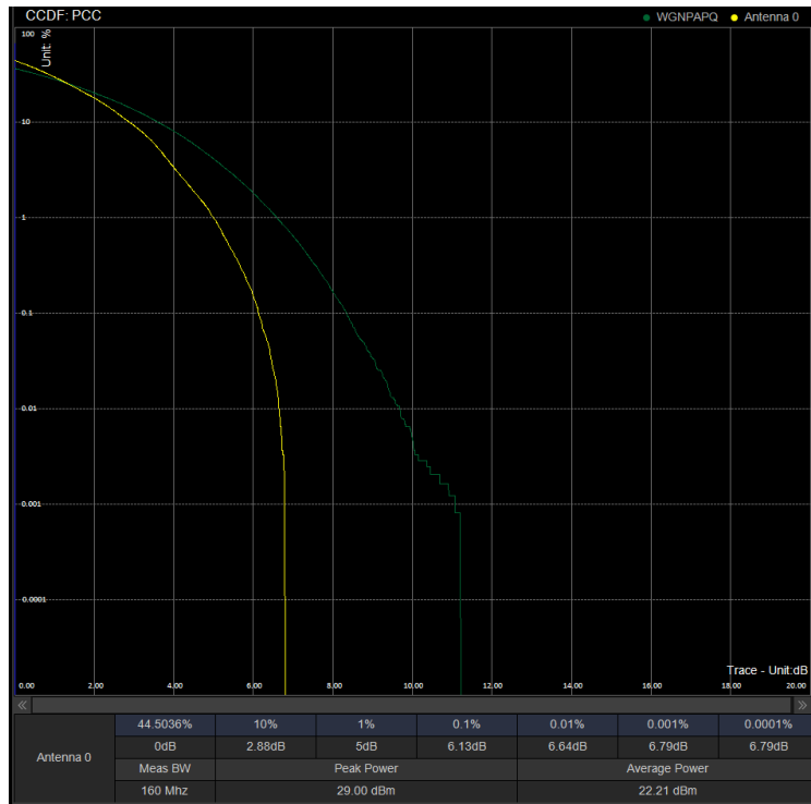
PAPR/PC3\N41\40M DFT 534000 100%RB 64QAM
