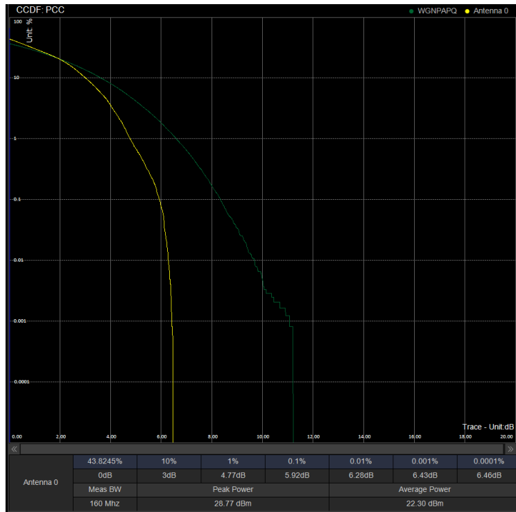
PAPR/PC3\N41\50M DFT 518598 100%RB 16QAM
