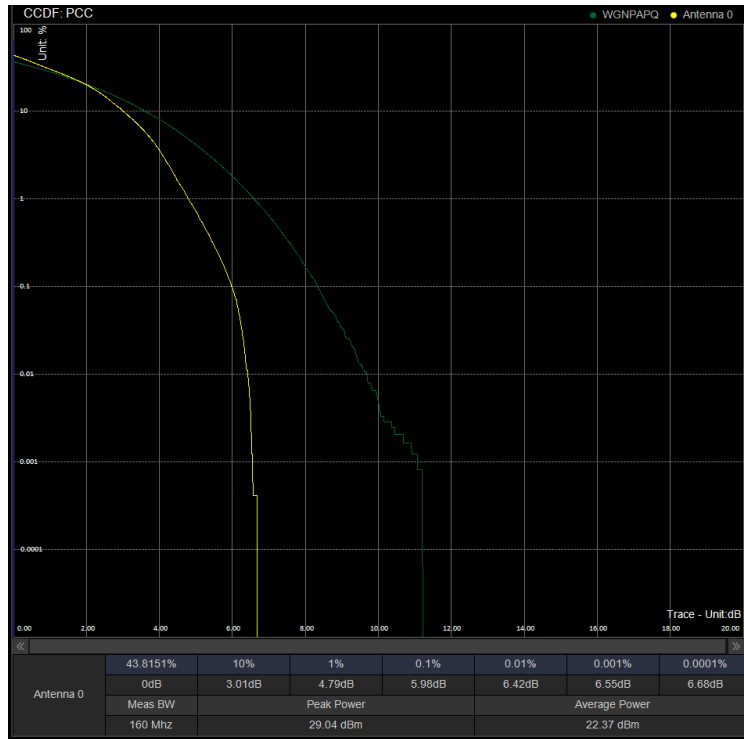
PAPR/PC3\N41\50M DFT 504204 100%RB 16QAM
