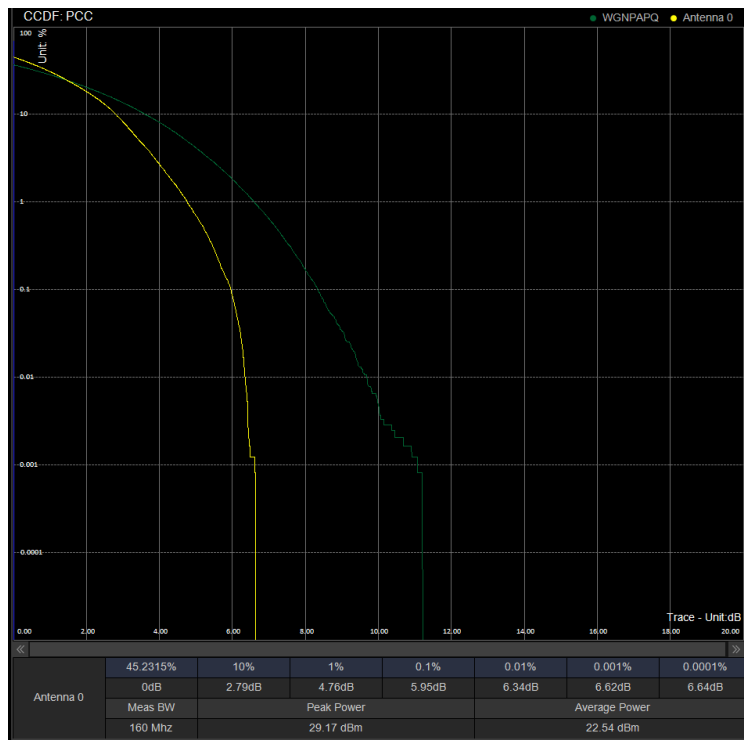
PAPR/PC3\N41\60M DFT 505200 100%RB 16QAM
