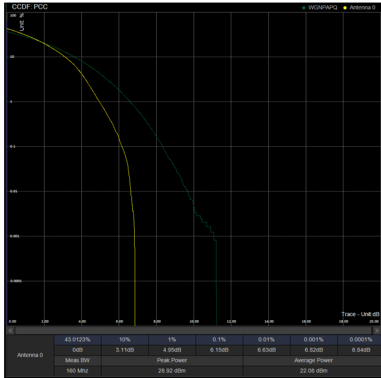
PAPR/PC3\N41\50M DFT 504204 100%RB 64QAM
