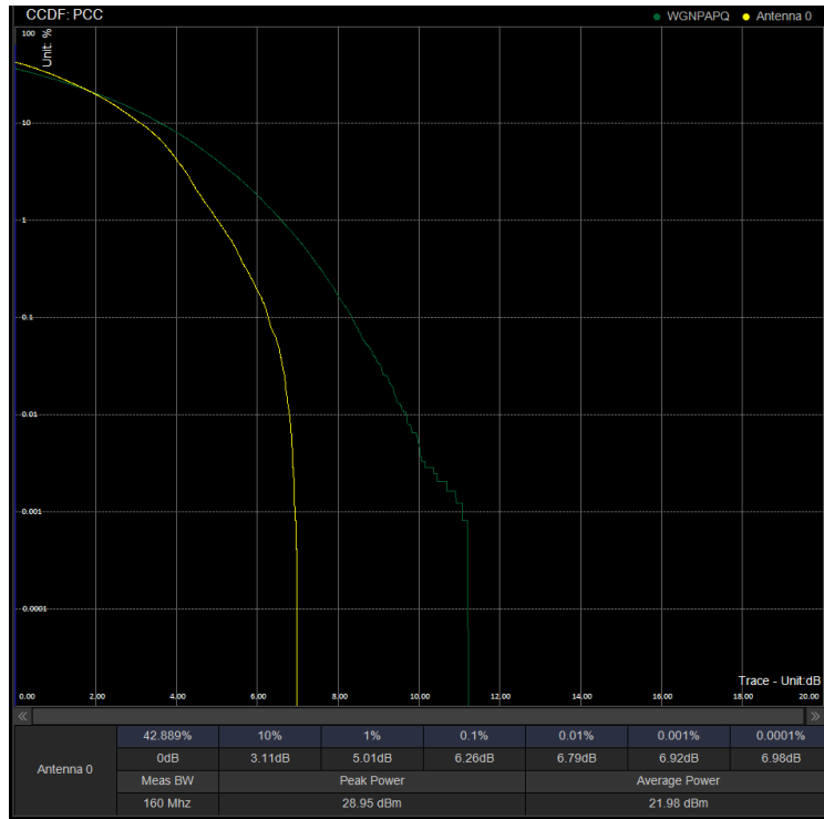
PAPR/PC3\N41\50M DFT 532998 100%RB 64QAM
