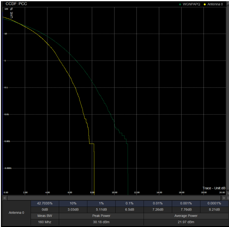
PAPR/PC3\N41\100M DFT 518598 100%RB 64QAM
