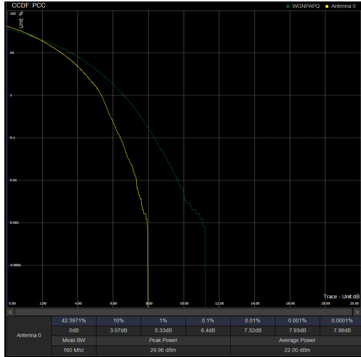
PAPR/PC3\N41\100M DFT 528000 100%RB 64QAM
