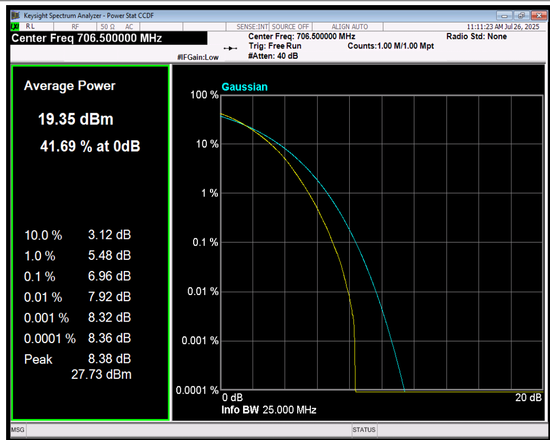
Band17 256QAM BW=5MHz Channel=23755 RB Size=25 Position=#0
