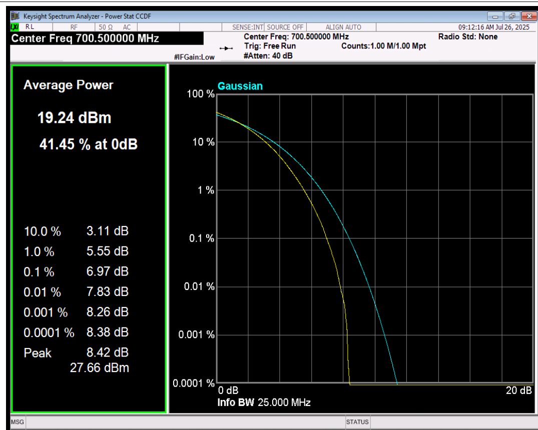
Band12 256QAM BW=3MHz Channel=23025 RB Size=15 Position=#0
