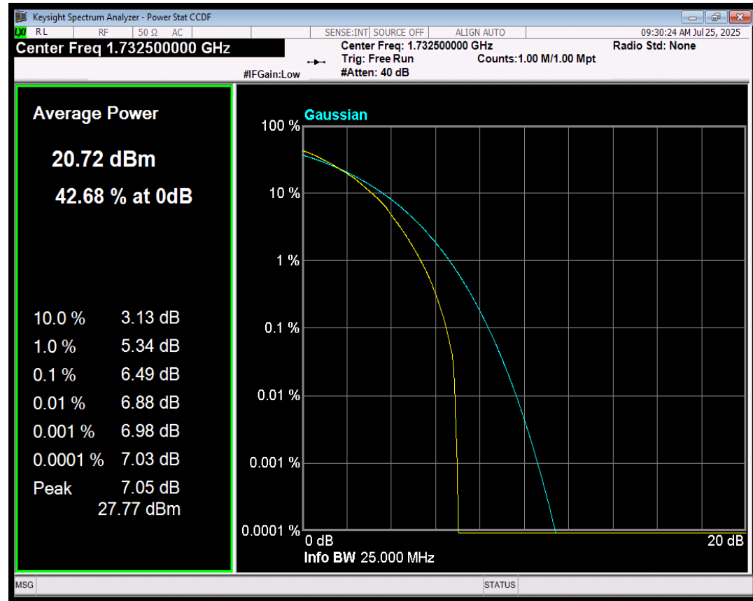
Band4 64QAM BW=3MHz Channel=20175 RB Size=15 Position=#0
