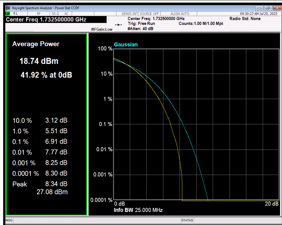
Band4 256QAM BW=3MHz Channel=20175 RB Size=15 Position=#0
