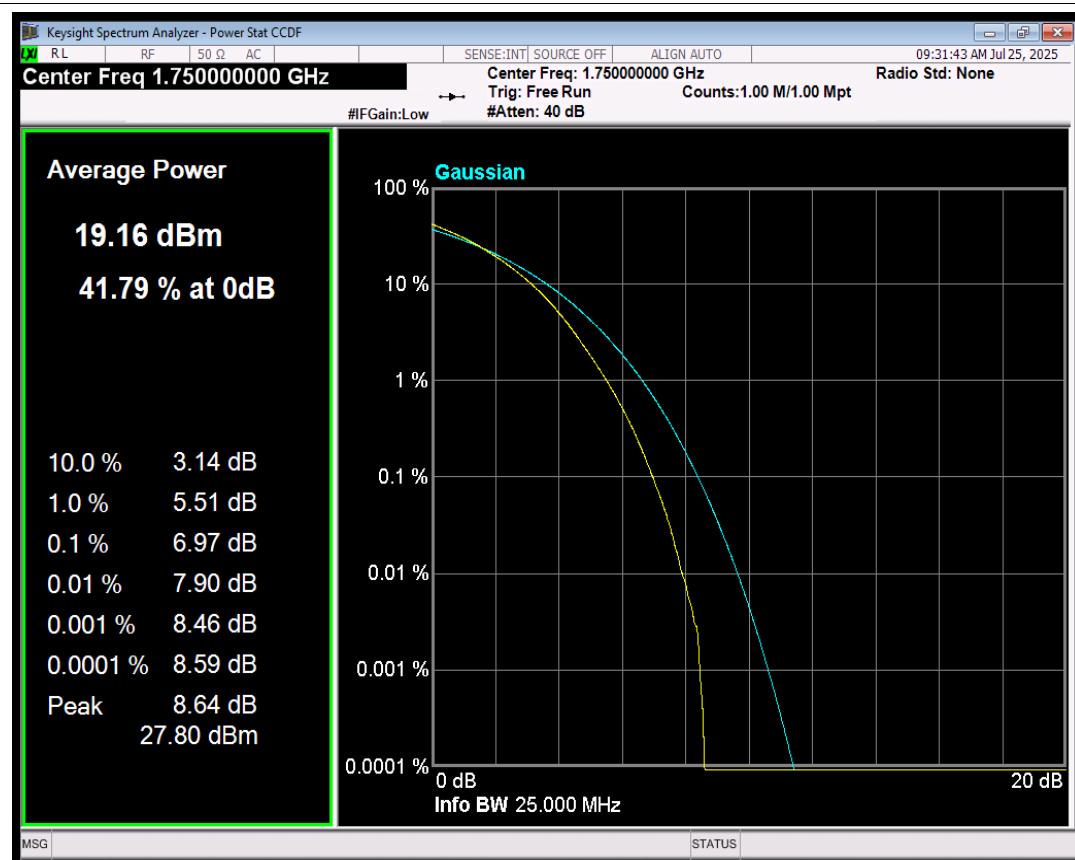
Band4 256QAM BW=10MHz Channel=20350 RB Size=50 Position=#0
