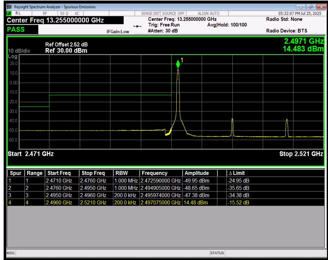
Band41 256QAM BW=20MHz LowChannel=39750 RB Size=1 Position=#0
