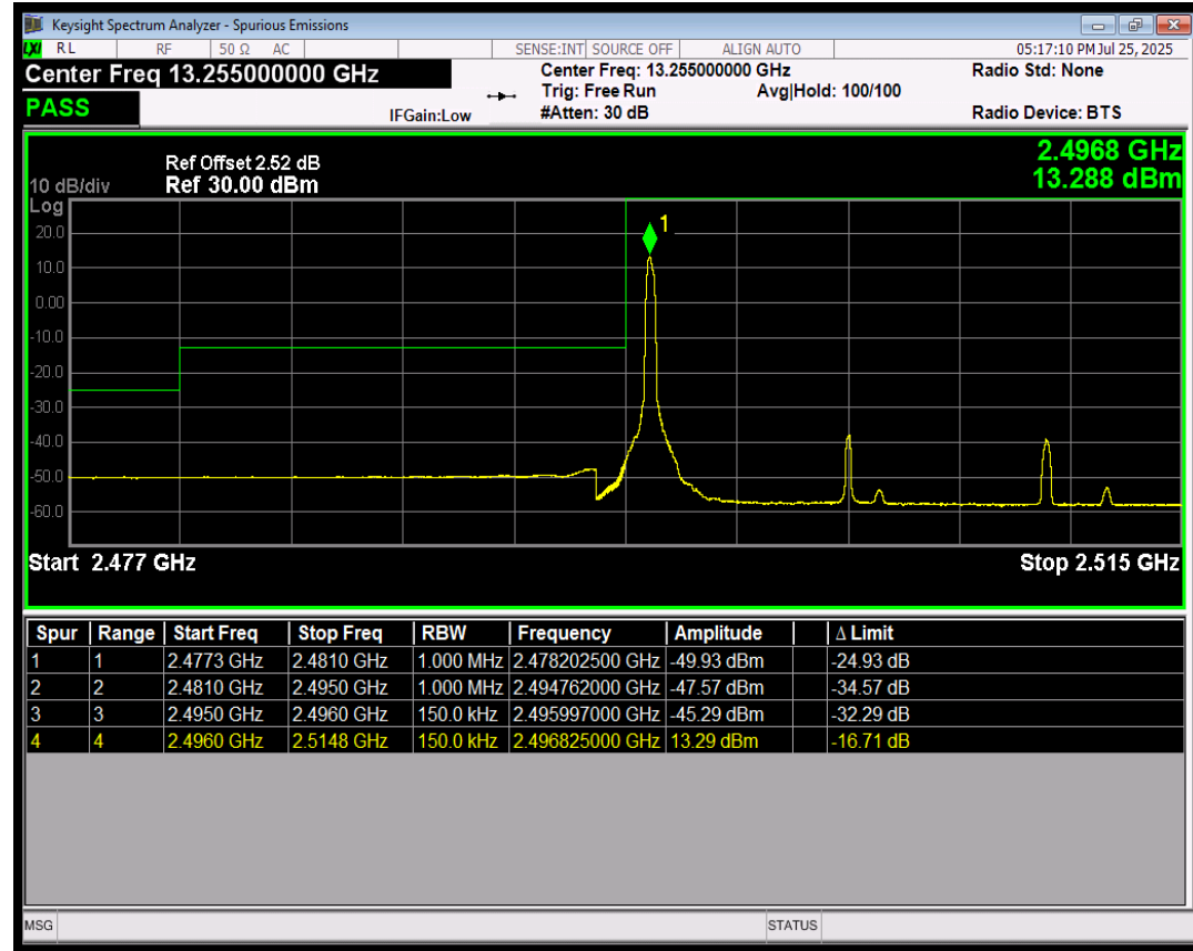
Band41 256QAM BW=15MHz LowChannel=39725 RB Size=1 Position=#0
