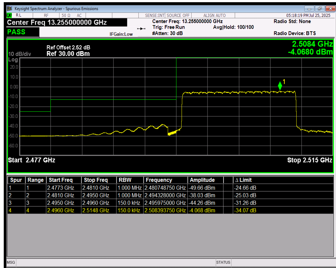
Band41 256QAM BW=15MHz LowChannel=39725 RB Size=75 Position=#0
