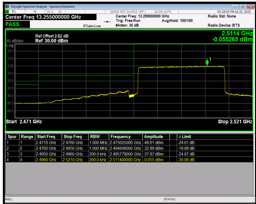
Band41 QPSK BW=20MHz LowChannel=39750 RB Size=100 Position=#0
