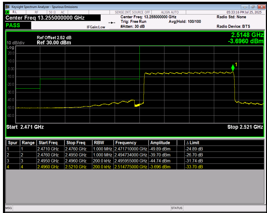
Band41 256QAM BW=20MHz LowChannel=39750 RB Size=100 Position=#0
