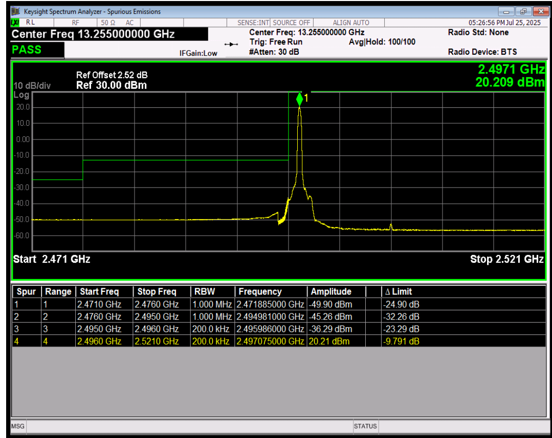
Band41 QPSK BW=20MHz LowChannel=39750 RB Size=1 Position=#0
