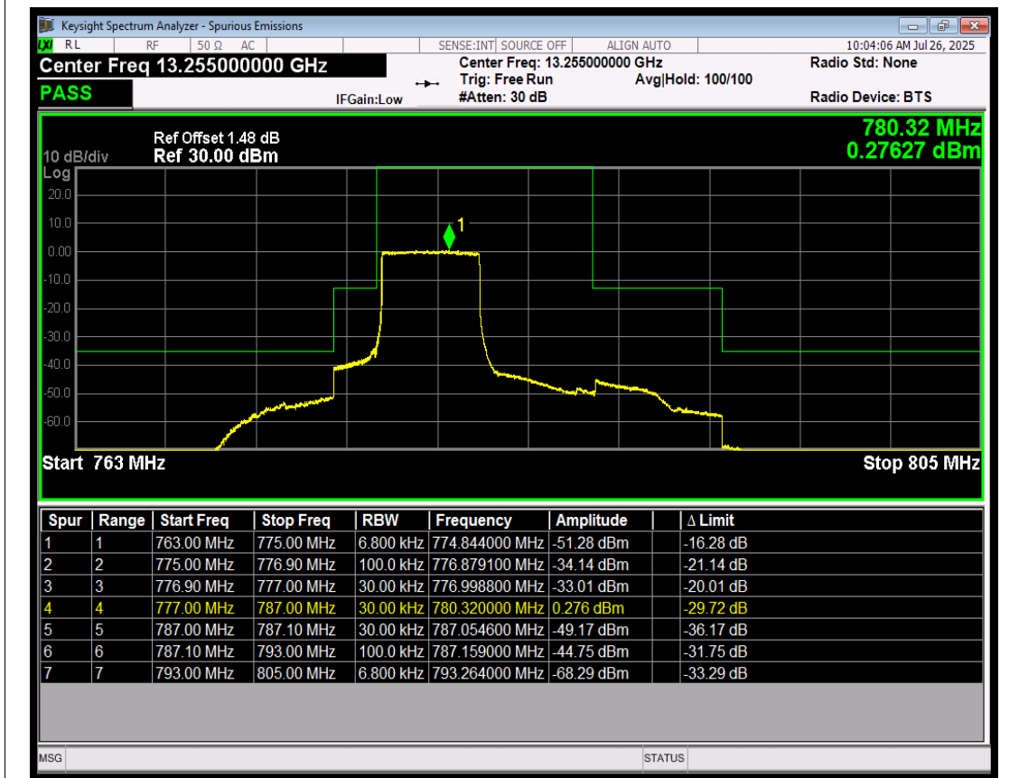
Band13 QPSK BW=5MHz LowChannel=23205 RB Size=25 Position=#0
