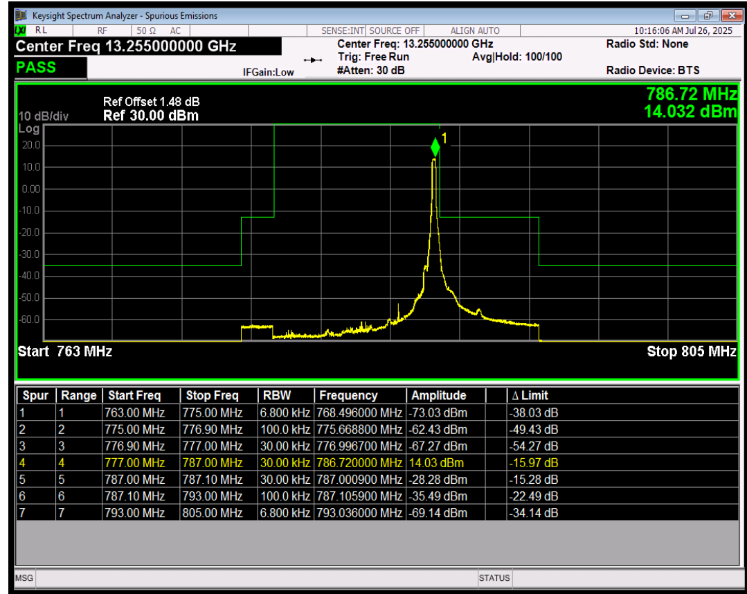
Band13 16QAM BW=5MHz HighChannel=23255 RB Size=1 Position=#Max
