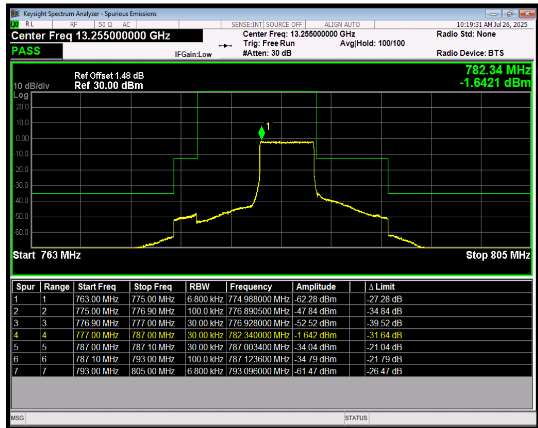
Band13 64QAM BW=5MHz HighChannel=23255 RB Size=25 Position=#0
