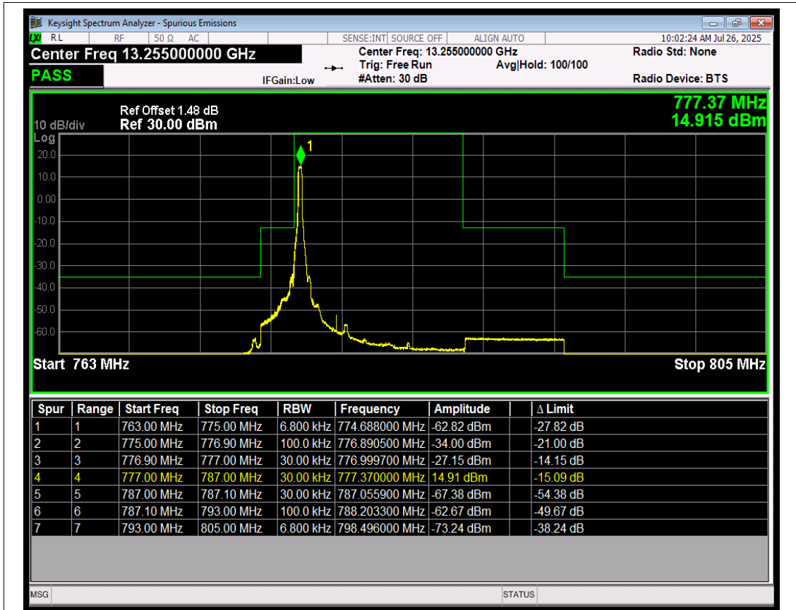
Band13 QPSK BW=5MHz LowChannel=23205 RB Size=1 Position=#0
