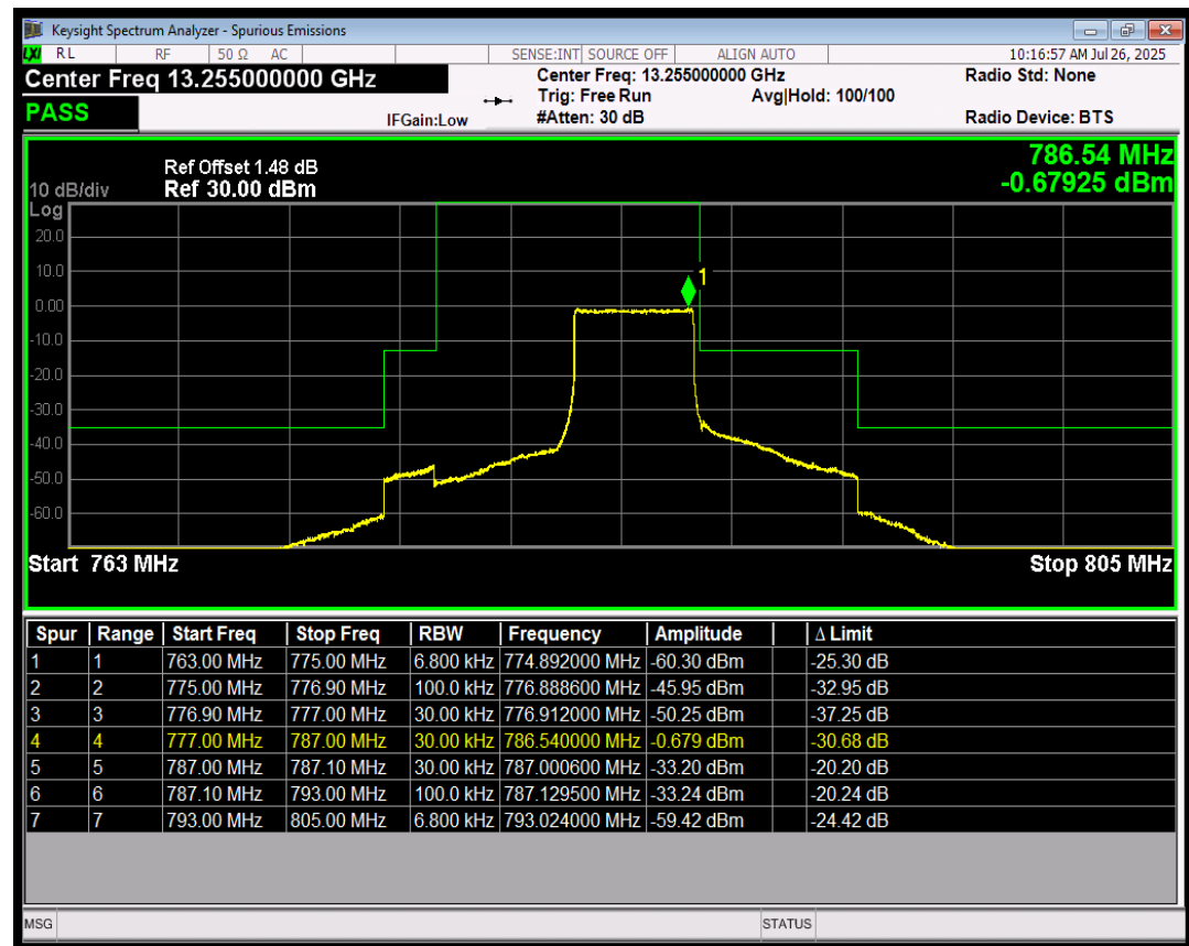
Band13 16QAM BW=5MHz HighChannel=23255 RB Size=25 Position=#0
