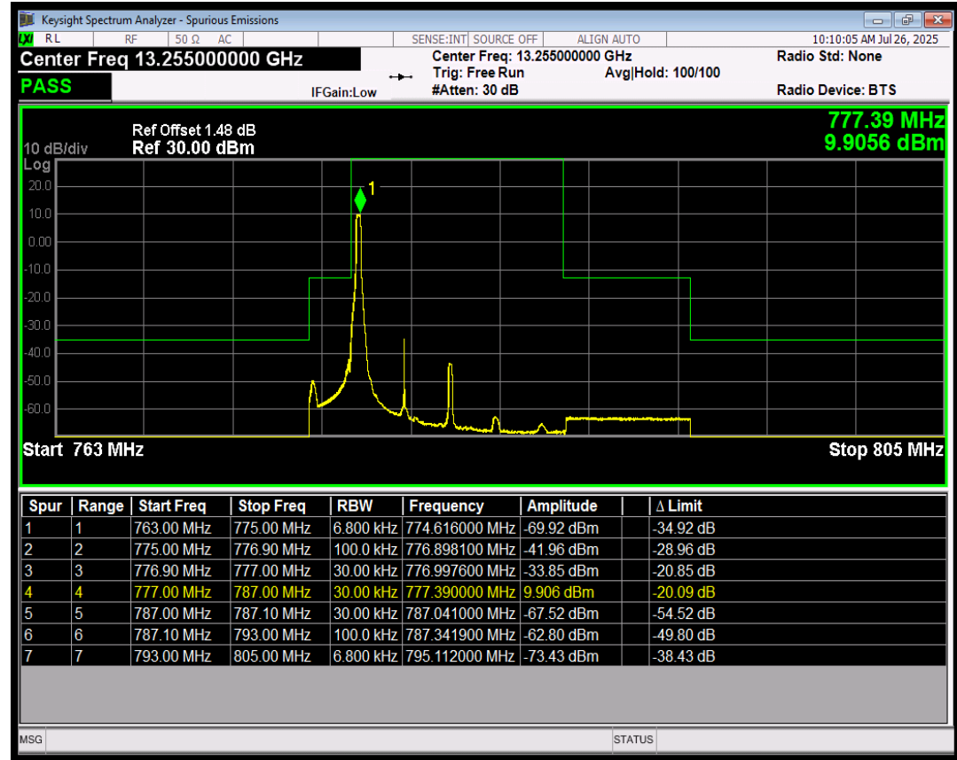
Band13 256QAM BW=5MHz LowChannel=23205 RB Size=1 Position=#0
