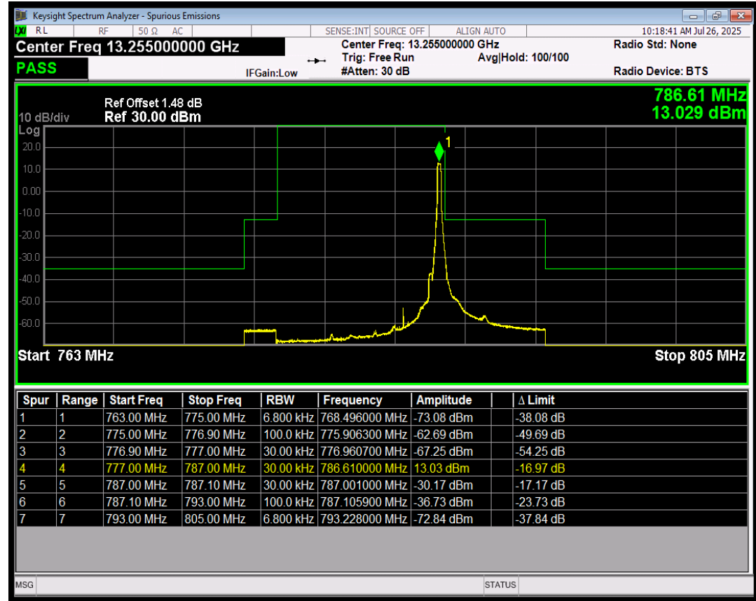
Band13 64QAM BW=5MHz HighChannel=23255 RB Size=1 Position=#Max
