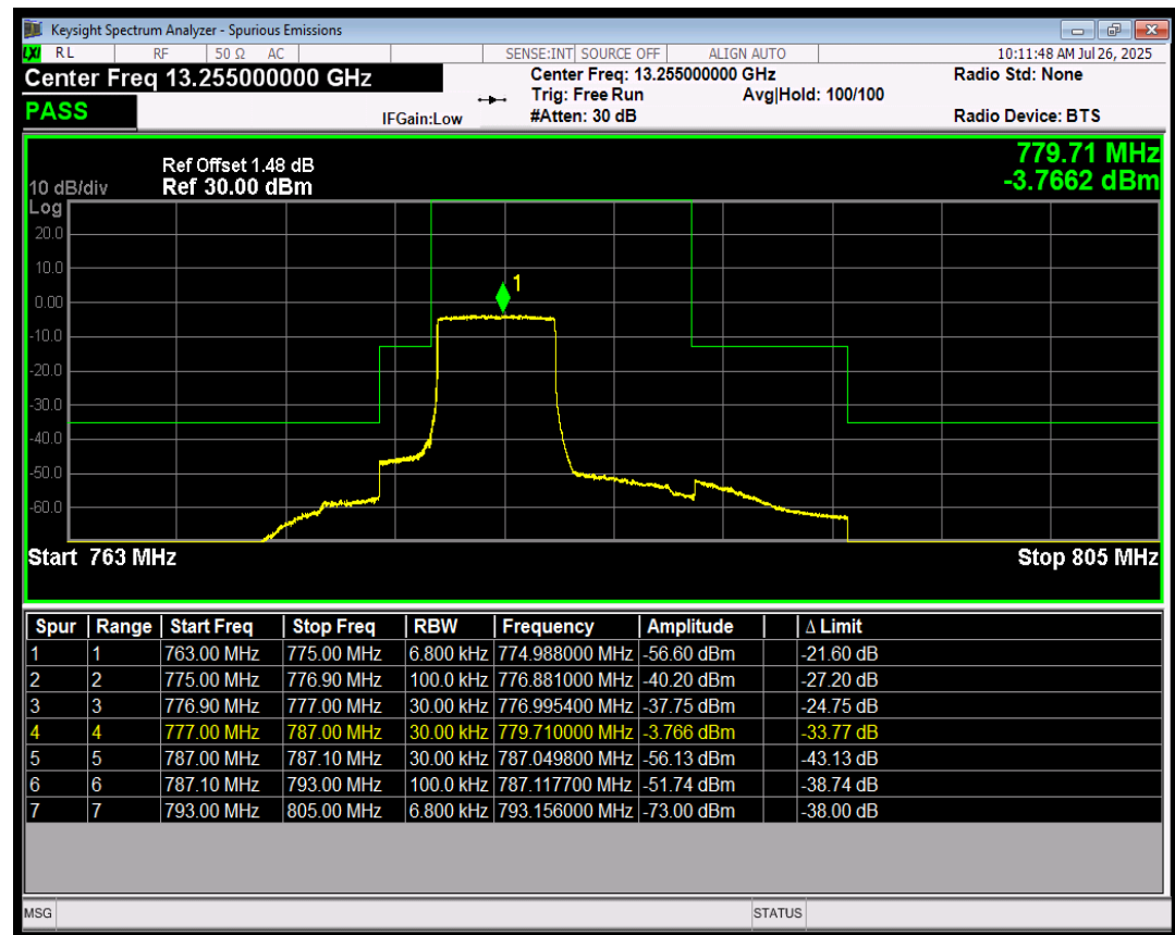
Band13 256QAM BW=5MHz LowChannel=23205 RB Size=25 Position=#0
