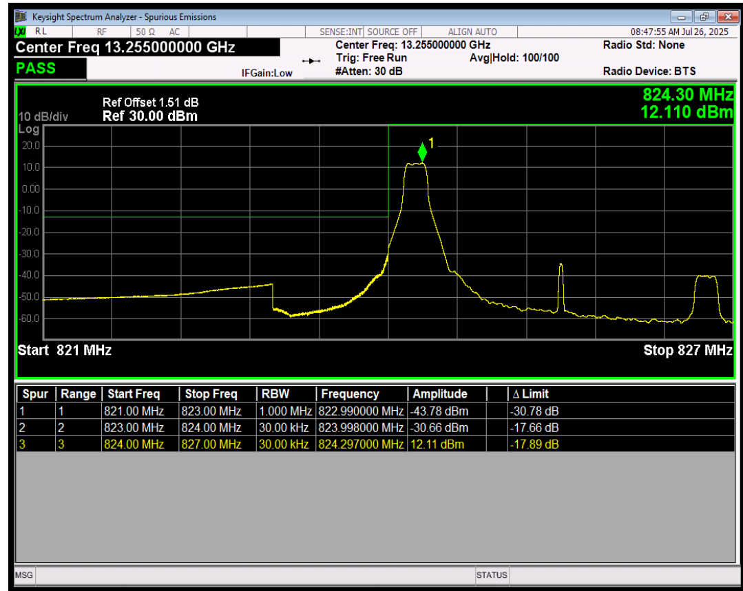
Band5 256QAM BW=3MHz LowChannel=20415 RB Size=1 Position=#0
