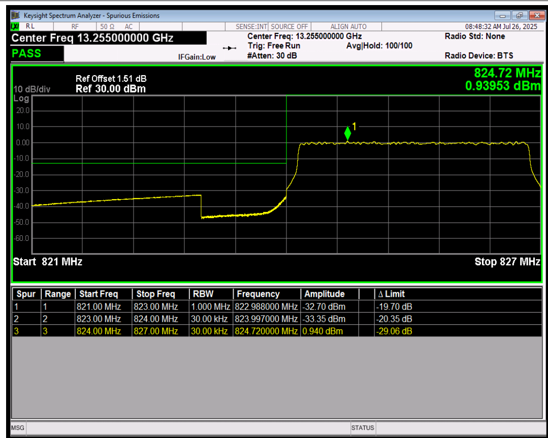
Band5 256QAM BW=3MHz LowChannel=20415 RB Size=15 Position=#0
