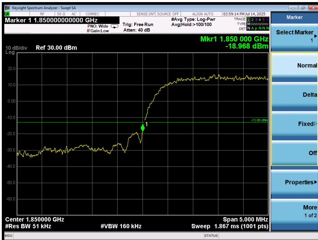
Band Edge\WCDMA B2\L
