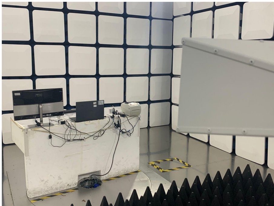
Above 1 GHz(65W)
