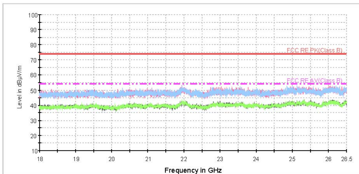
Radiated Emission from 18GHz to 26.5GHz
