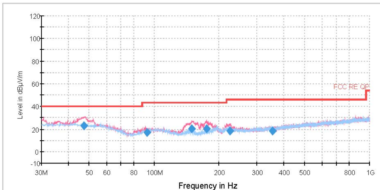
Radiated Emission from 30MHz to 1GHz
