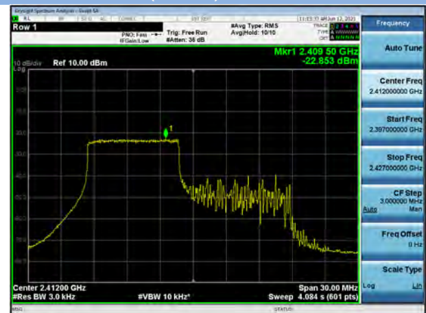
802.11ax-20 MHz(RU106) LOW CHANNEL
