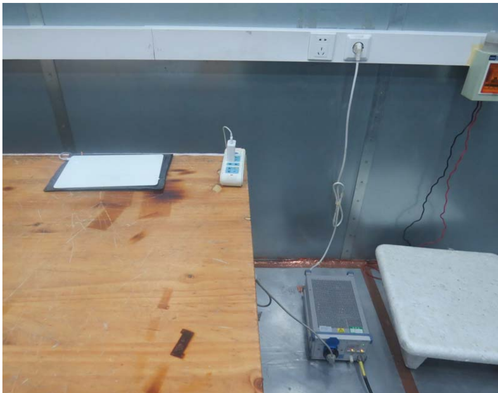
Picture 2 Conducted Emission Test Setup
