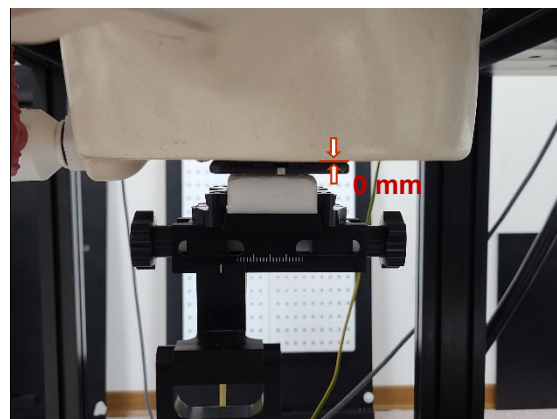
Photograph 28. Extremity, Back Surface, 0mm
