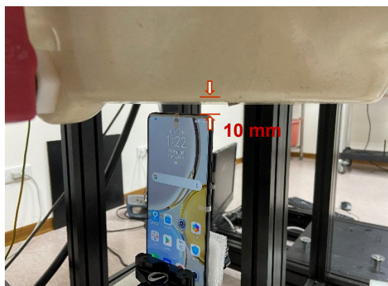
Photograph 17. Hotspot, Top Edge, 10mm
