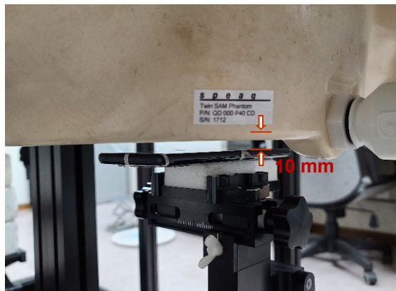
Photograph 13. Hotspot, Front Surface, 10mm
