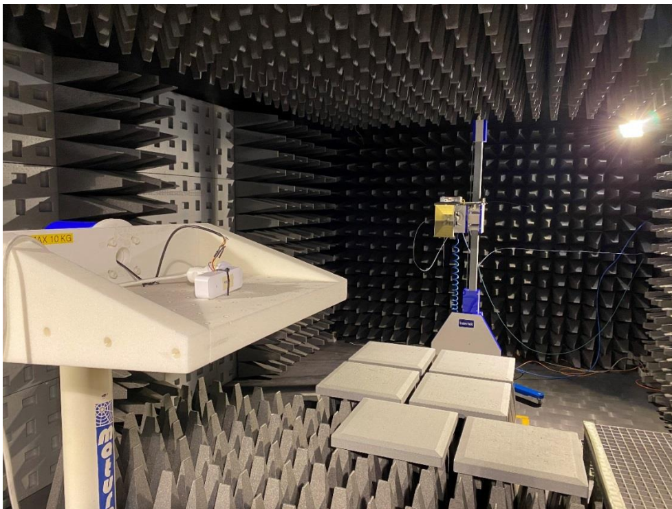
Test set up radiated emission above 1 GHz
