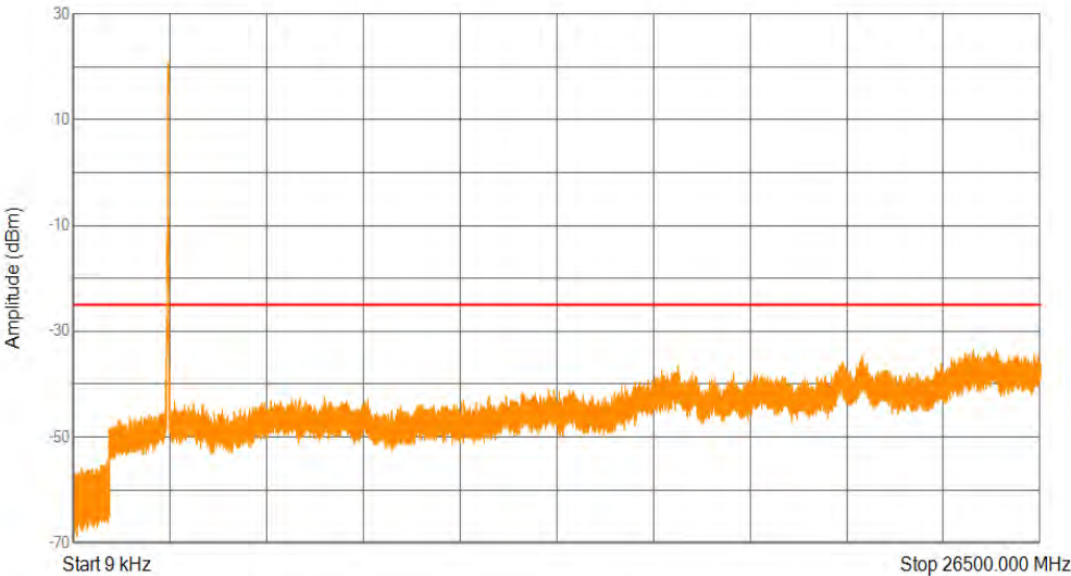
Band41(2555-2655) QPSK BW=15MHz Channel=40740 RB Size=75 Position=#0
