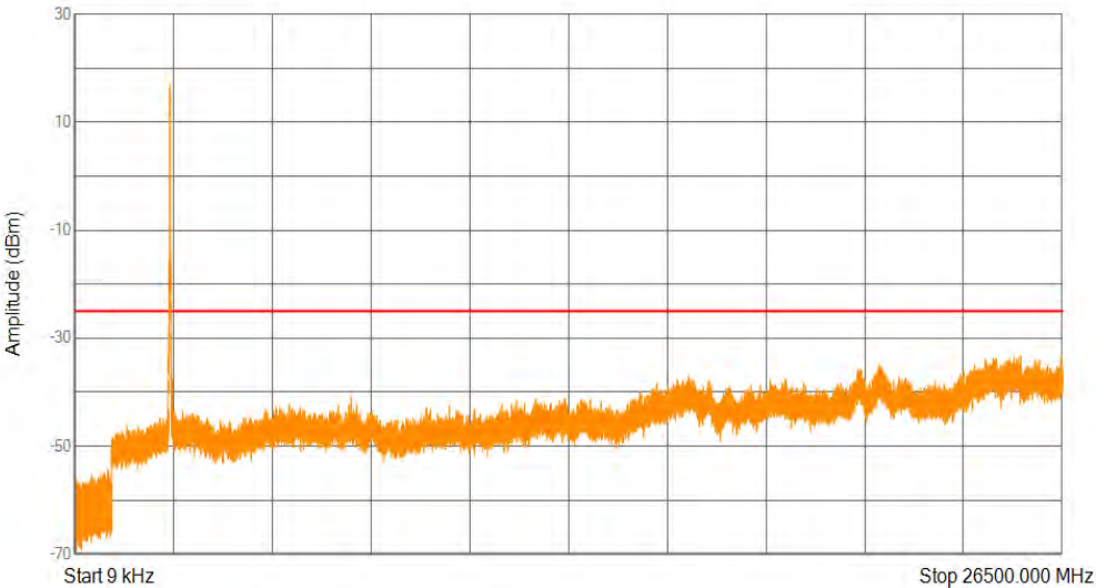
Band41(2555-2655) 16QAM BW=20MHz Channel=40340 RB Size=100 Position=#0
