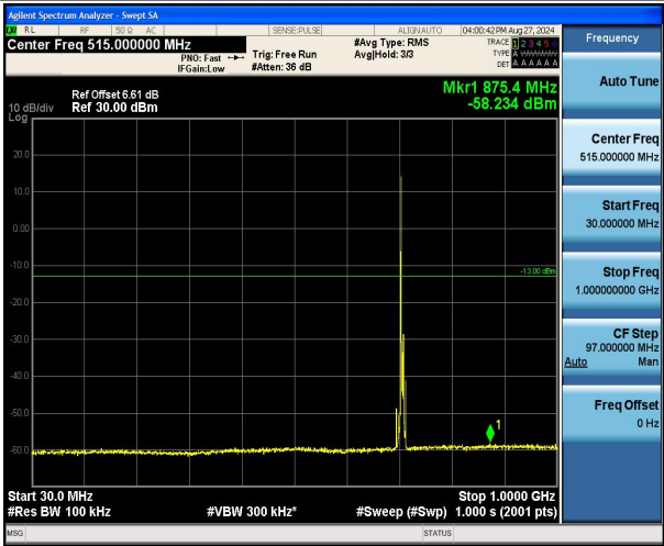
Band17_5MHz_16QAM_23825_1RB#0_30~1000_30~1000
