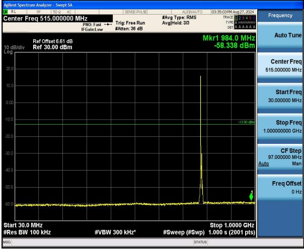
Band13_5MHz_QPSK_23230_1RB#0_30~1000_30~1000
