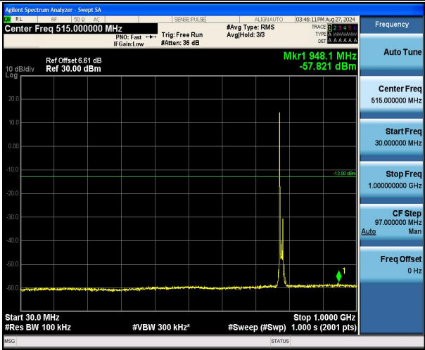
Band13_10MHz_QPSK_23230_1RB#0_30~1000_30~1000
