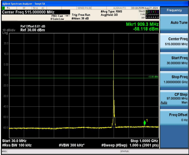
Band12_10MHz_16QAM_23130_1RB#0_30~1000_30~1000
