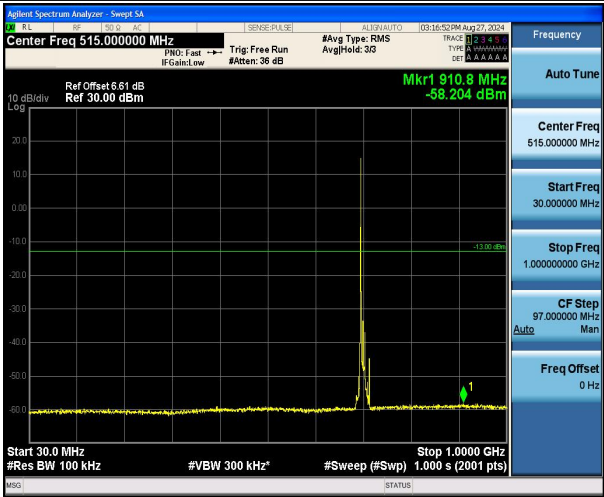
Band12_10MHz_QPSK_23095_1RB#0_30~1000_30~1000
