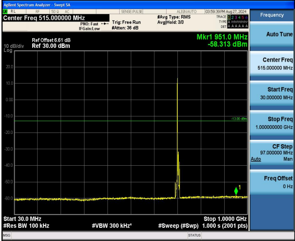
Band17_5MHz_16QAM_23790_1RB#0_30~1000_30~1000
