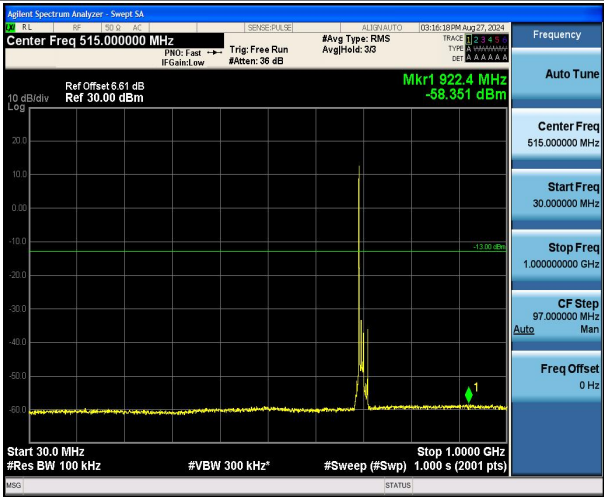
Band12_10MHz_16QAM_23060_1RB#0_30~1000_30~1000
