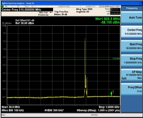
Band12_10MHz_QPSK_23060_1RB#0_30~1000_30~1000
