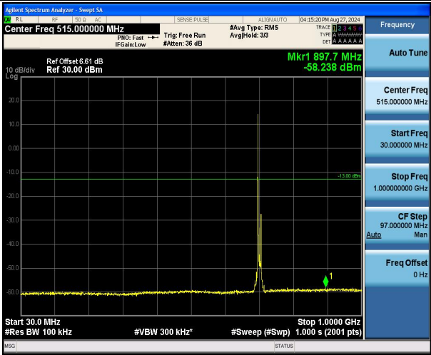
Band17_10MHz_16QAM_23780_1RB#0_30~1000_30~1000
