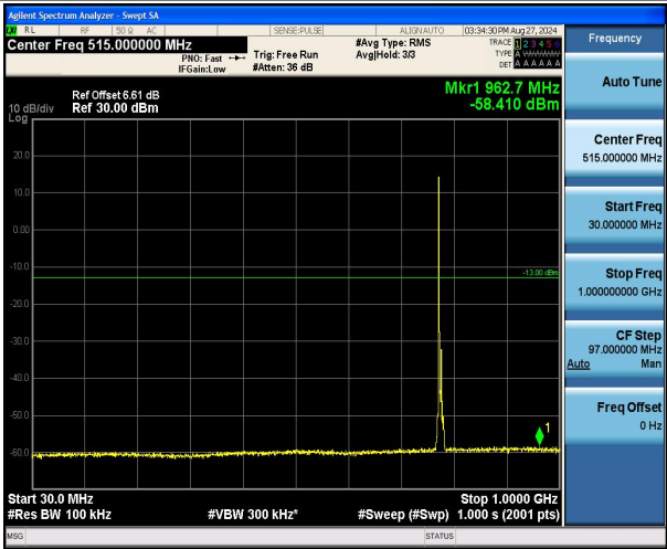
Band13_5MHz_16QAM_23205_1RB#0_30~1000_30~1000
