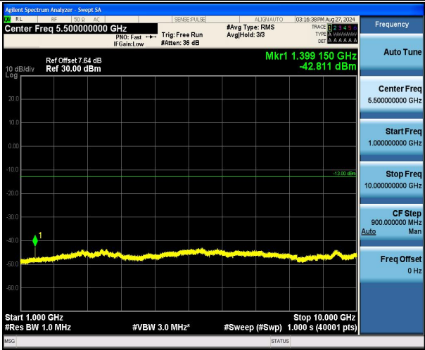
Band12_10MHz_16QAM_23060_1RB#0_1000~10000_1000~10000
