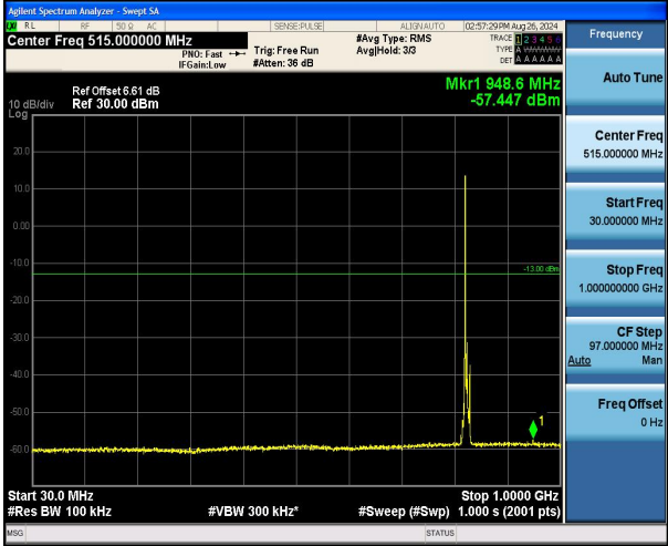
Band5_5MHz_16QAM_20425_1RB#0_30~1000_30~1000
