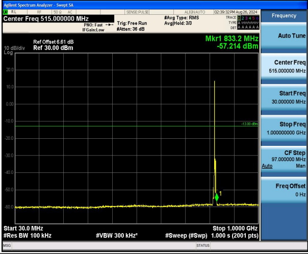
Band5_3MHz_16QAM_20415_1RB#0_30~1000_30~1000
