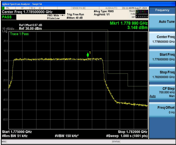
Band66_5MHz_QPSK_132647_25RB#0
