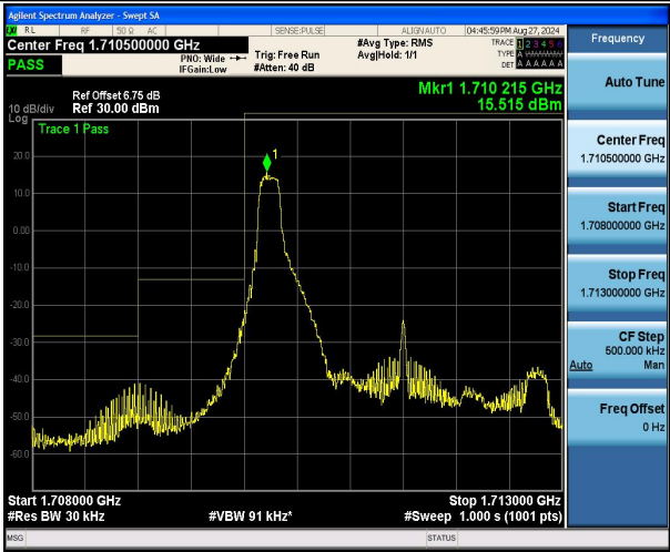
Band66_3MHz_QPSK_131987_1RB#0
