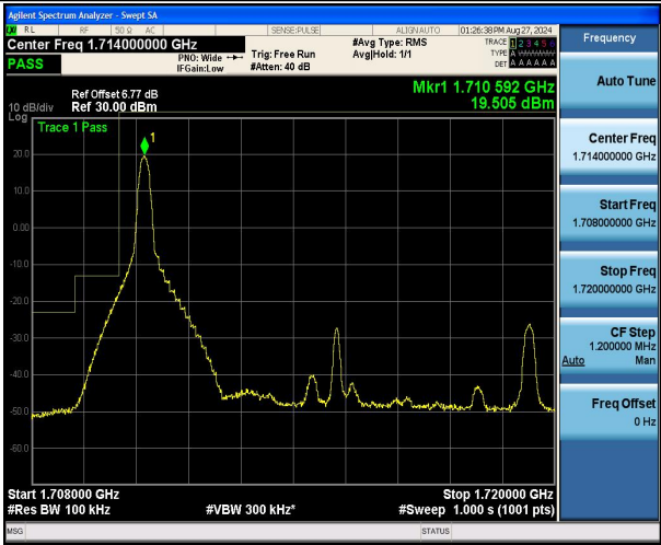
Band66_10MHz_QPSK_132022_1RB#0
