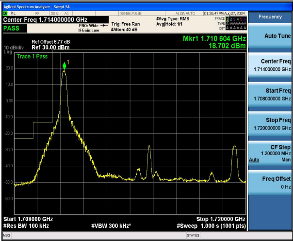
Band66_10MHz_16QAM_132022_1RB#0
