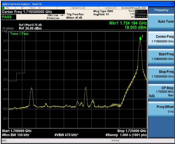
Band4_15MHz_16QAM_20025_1RB#74
