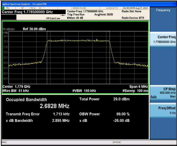
Band66-3MHz-QPSK-132657-15RB#0-PASS
