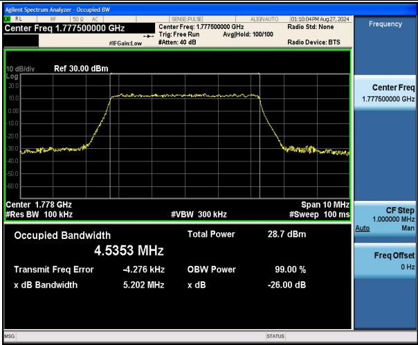
Band66-5MHz-16QAM-132647-25RB#0-PASS
