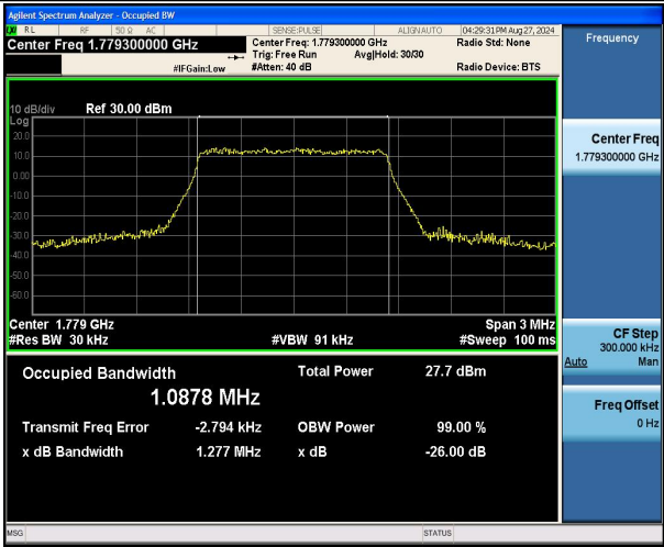
Band66-1.4MHz-16QAM-132665-6RB#0-PASS
