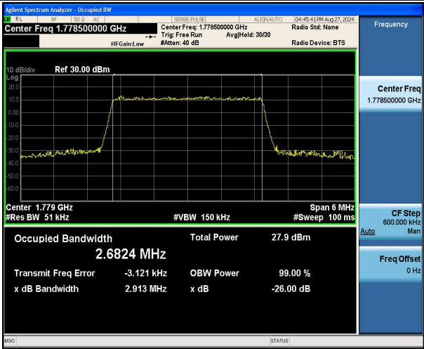
Band66-3MHz-16QAM-132657-15RB#0-PASS
