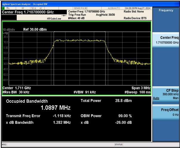
Band66-1.4MHz-QPSK-131979-6RB#0-PASS
