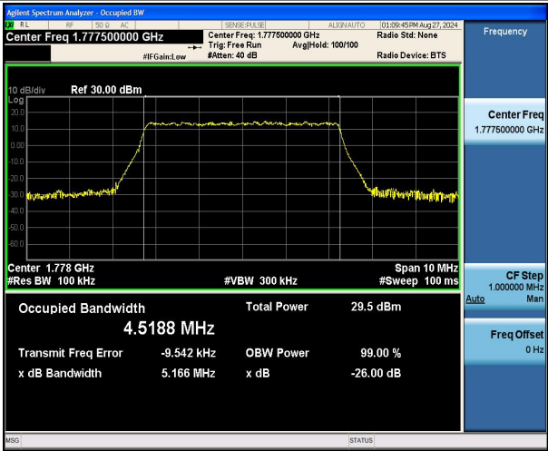
Band66-5MHz-QPSK-132647-25RB#0-PASS
