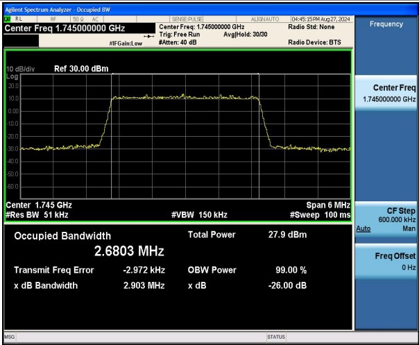
Band66-3MHz-16QAM-132322-15RB#0-PASS
