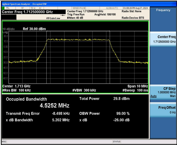
Band66-5MHz-QPSK-131997-25RB#0-PASS
