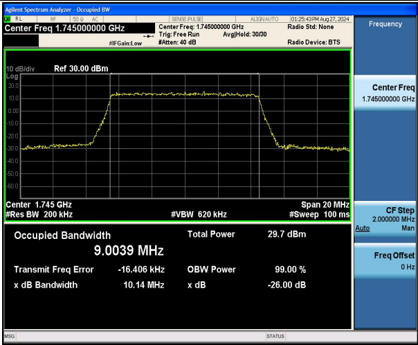
Band66-10MHz-QPSK-132322-50RB#0-PASS
