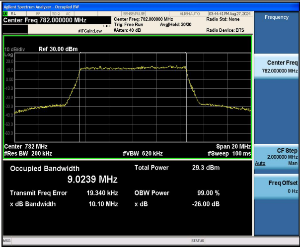
Band13-10MHz-16QAM-23230-50RB#0-PASS
