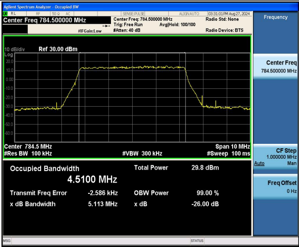
Band13-5MHz-QPSK-23255-25RB#0-PASS
