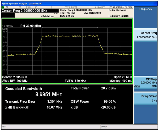
Band7-10MHz-16QAM-20800-50RB#0-PASS
