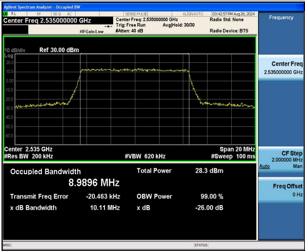
Band7-10MHz-16QAM-21100-50RB#0-PASS
