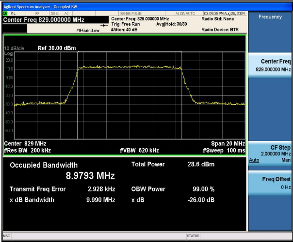
Band5-10MHz-16QAM-20450-50RB#0-PASS
