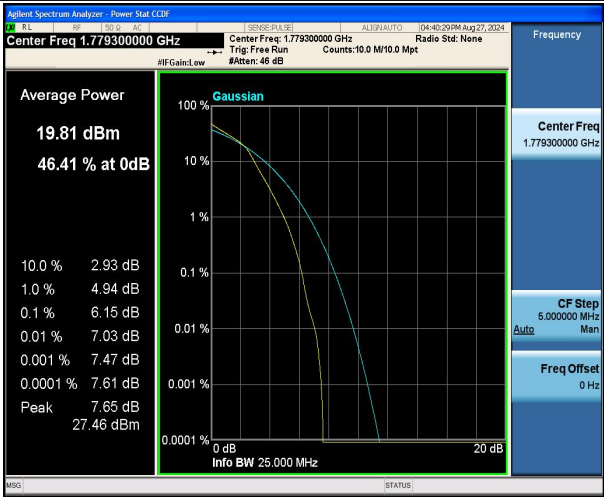
Band66-1.4MHz-16QAM-132665-6RB#0-PASS
