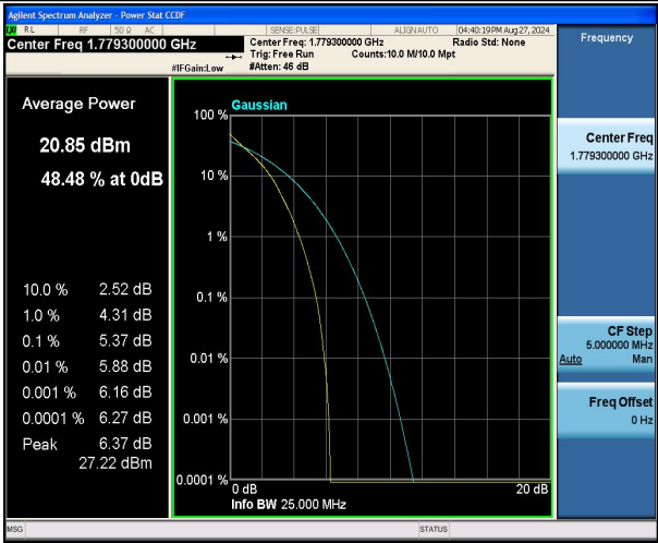
Band66-1.4MHz-QPSK-132665-6RB#0-PASS
