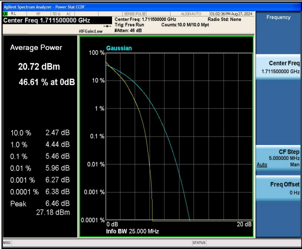
Band66-3MHz-QPSK-131987-15RB#0-PASS
