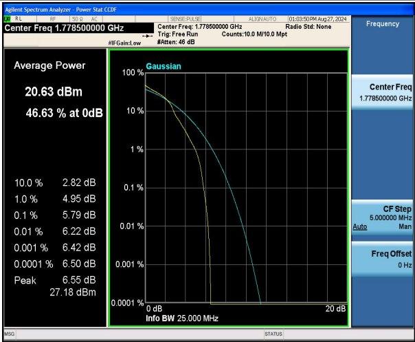
Band66-3MHz-16QAM-132657-1RB#0-PASS
