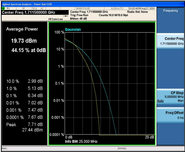
Band66-3MHz-16QAM-131987-15RB#0-PASS
