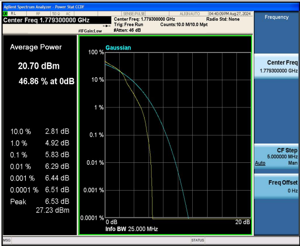
Band66-1.4MHz-16QAM-132665-1RB#0-PASS
