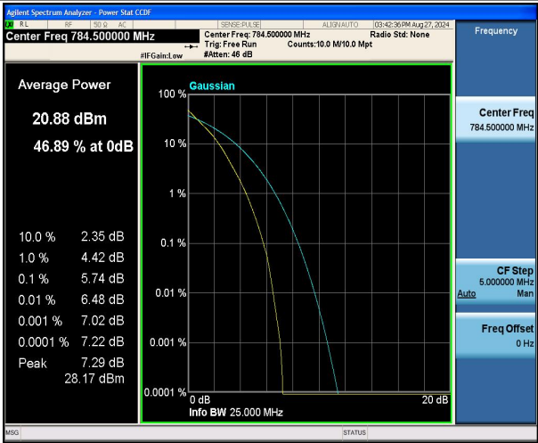
Band13-5MHz-QPSK-23255-25RB#0-PASS
