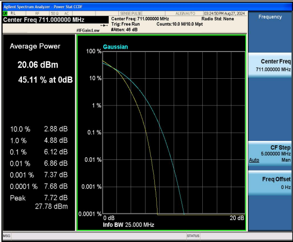
Band12-10MHz-16QAM-23130-50RB#0-PASS
