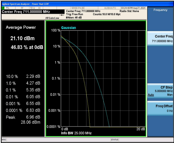
Band12-10MHz-QPSK-23130-50RB#0-PASS
