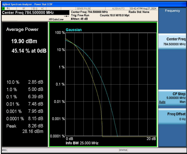
Band13-5MHz-16QAM-23255-25RB#0-PASS
