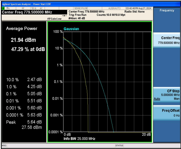
Band13-5MHz-QPSK-23205-1RB#0-PASS
