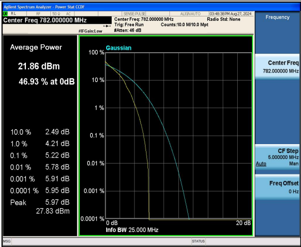
Band13-10MHz-QPSK-23230-1RB#0-PASS
