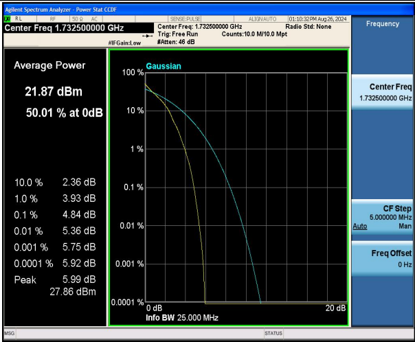
Band4-3MHz-QPSK-20175-1RB#0-PASS
