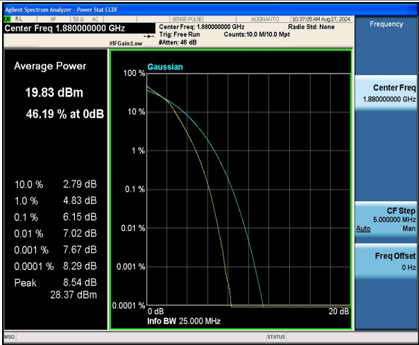
Band2-20MHz-16QAM-18900-100RB#0-PASS
