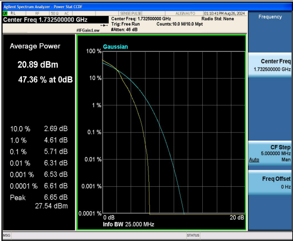
Band4-3MHz-16QAM-20175-1RB#0-PASS
