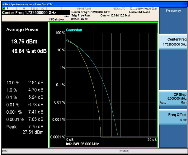
Band4-3MHz-16QAM-20175-15RB#0-PASS
