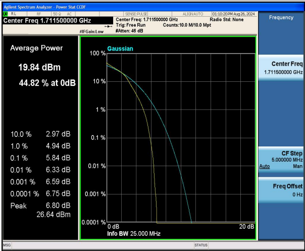
Band4-3MHz-16QAM-19965-15RB#0-PASS
