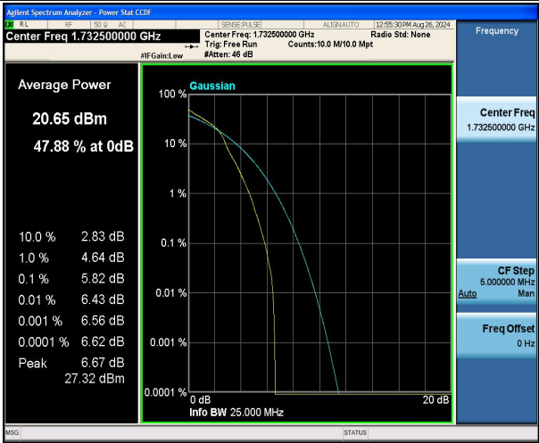
Band4-1.4MHz-16QAM-20175-1RB#0-PASS
