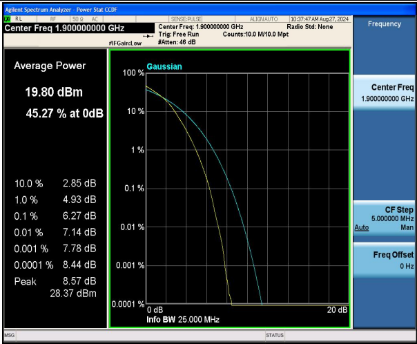
Band2-20MHz-16QAM-19100-100RB#0-PASS
