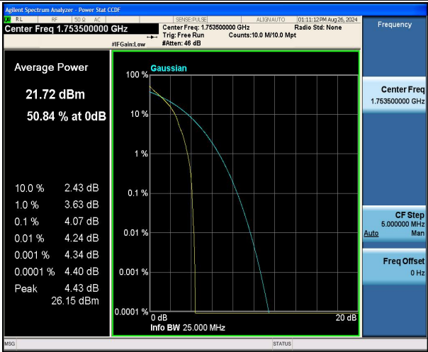
Band4-3MHz-QPSK-20385-1RB#0-PASS
